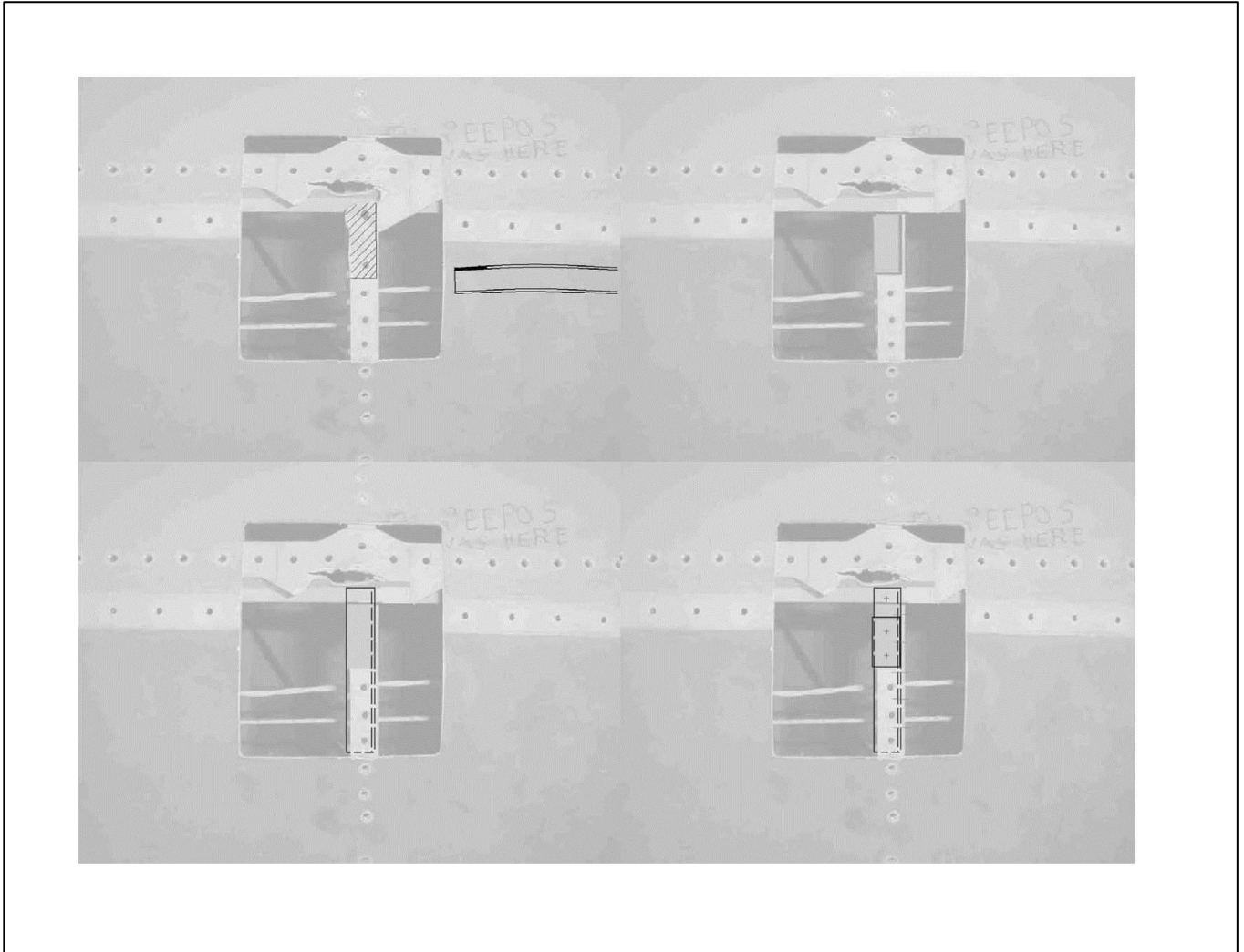
Figure 8: AH-64D Tailboom Battle Damage Example, Filler
