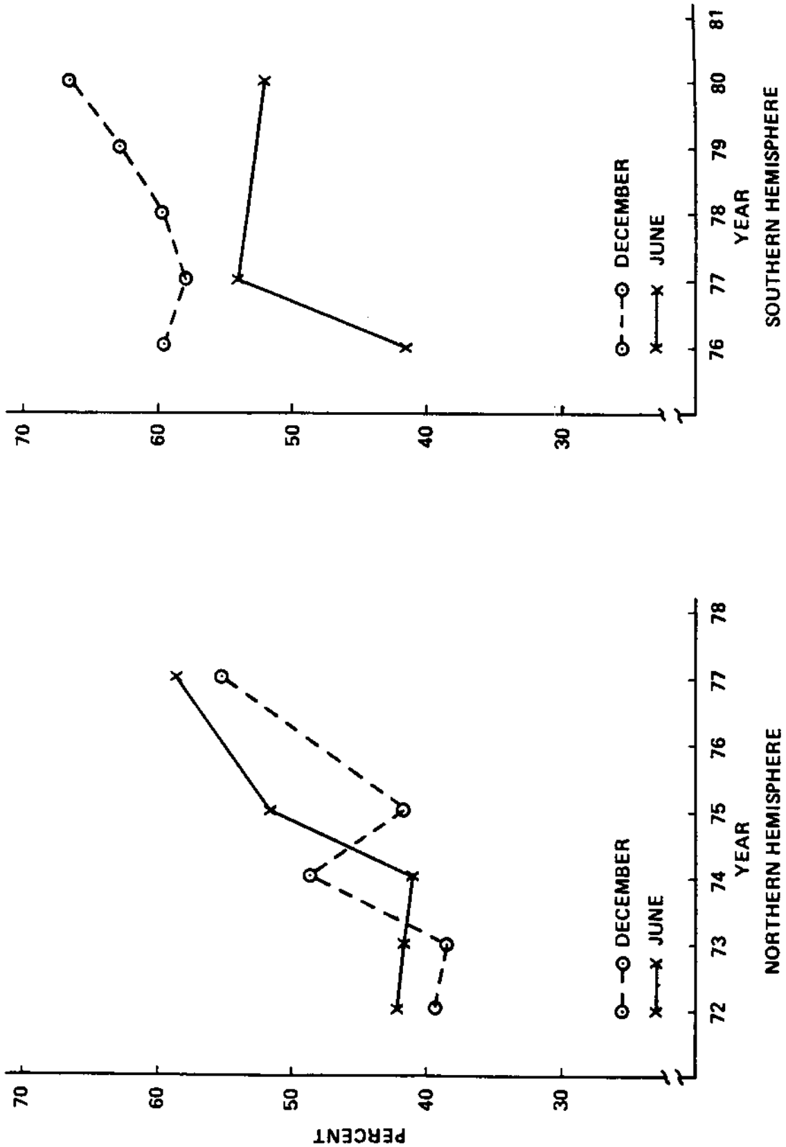
Figure 8.6 Mean monthly cloud cover.
