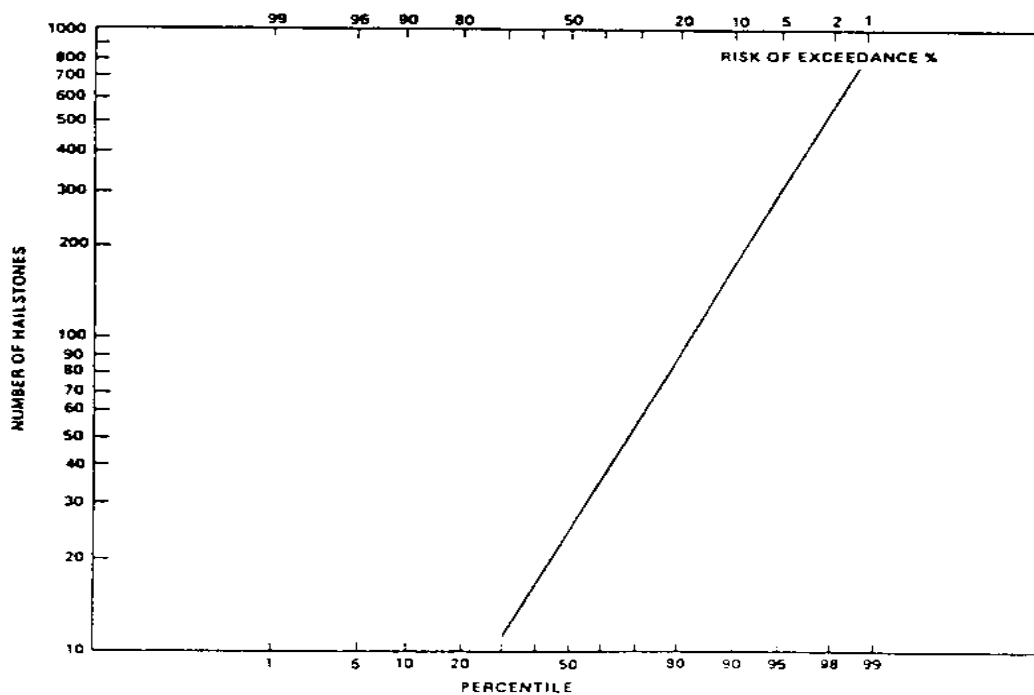
FIGURE 7.8 Probability (Percent) of Number of Stones Per Hailfall on Hailpad of 930 cm² (1 ft²).
