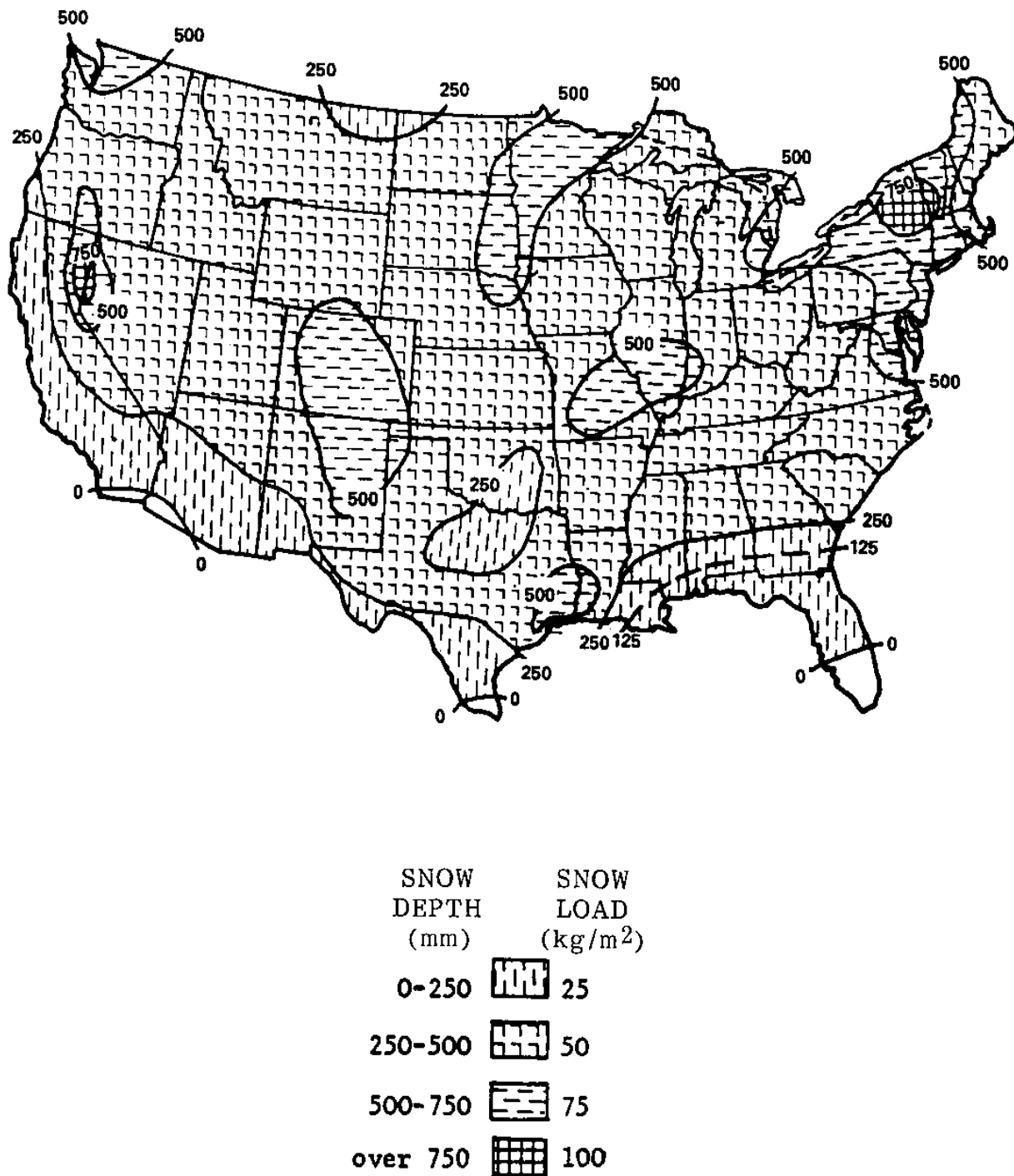
FIGURE 5.5 Extreme 24-h Maximum Snowfall (mm) and Maximum Snow Load.
