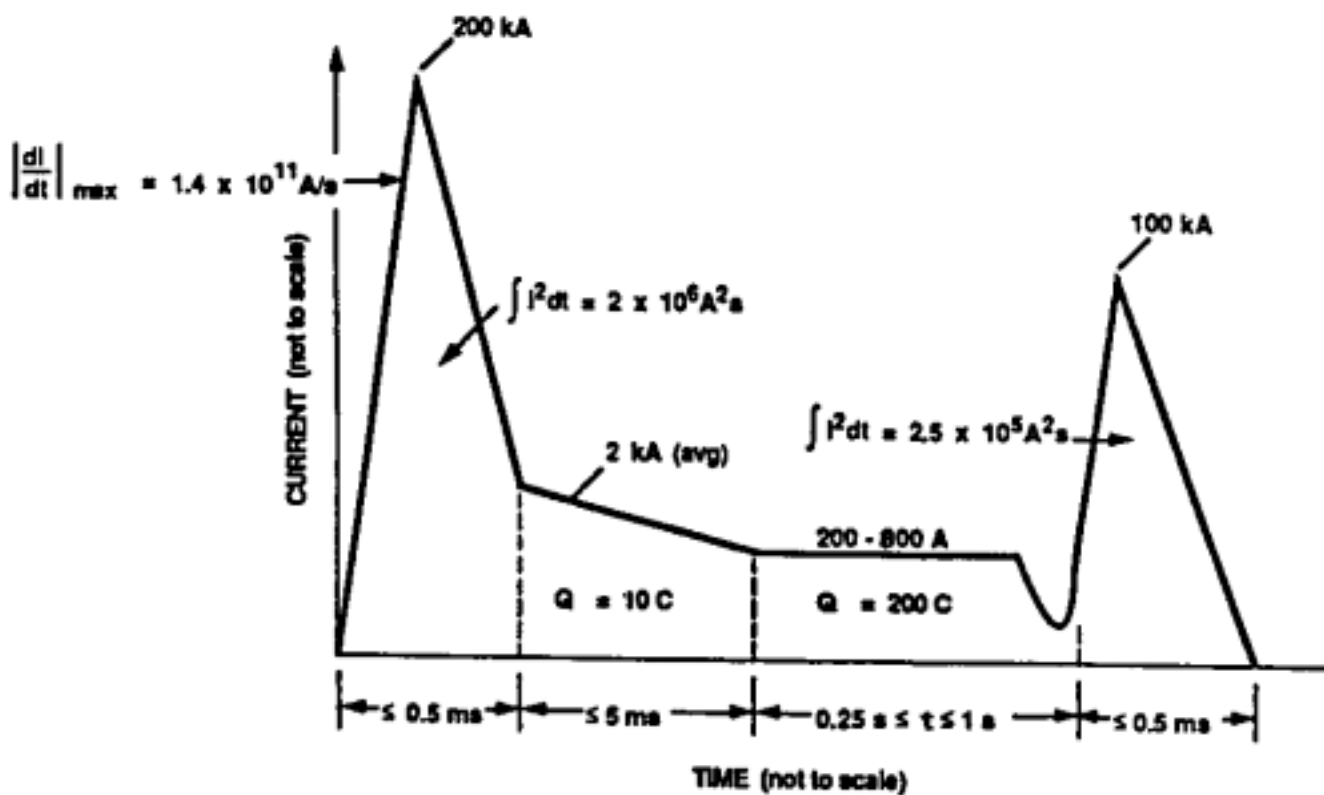
FIGURE 9.9 Current Waveform Composed of the Four Components A, B, C, and D Shown in Figure 9.8 (Ref. 9.5).
