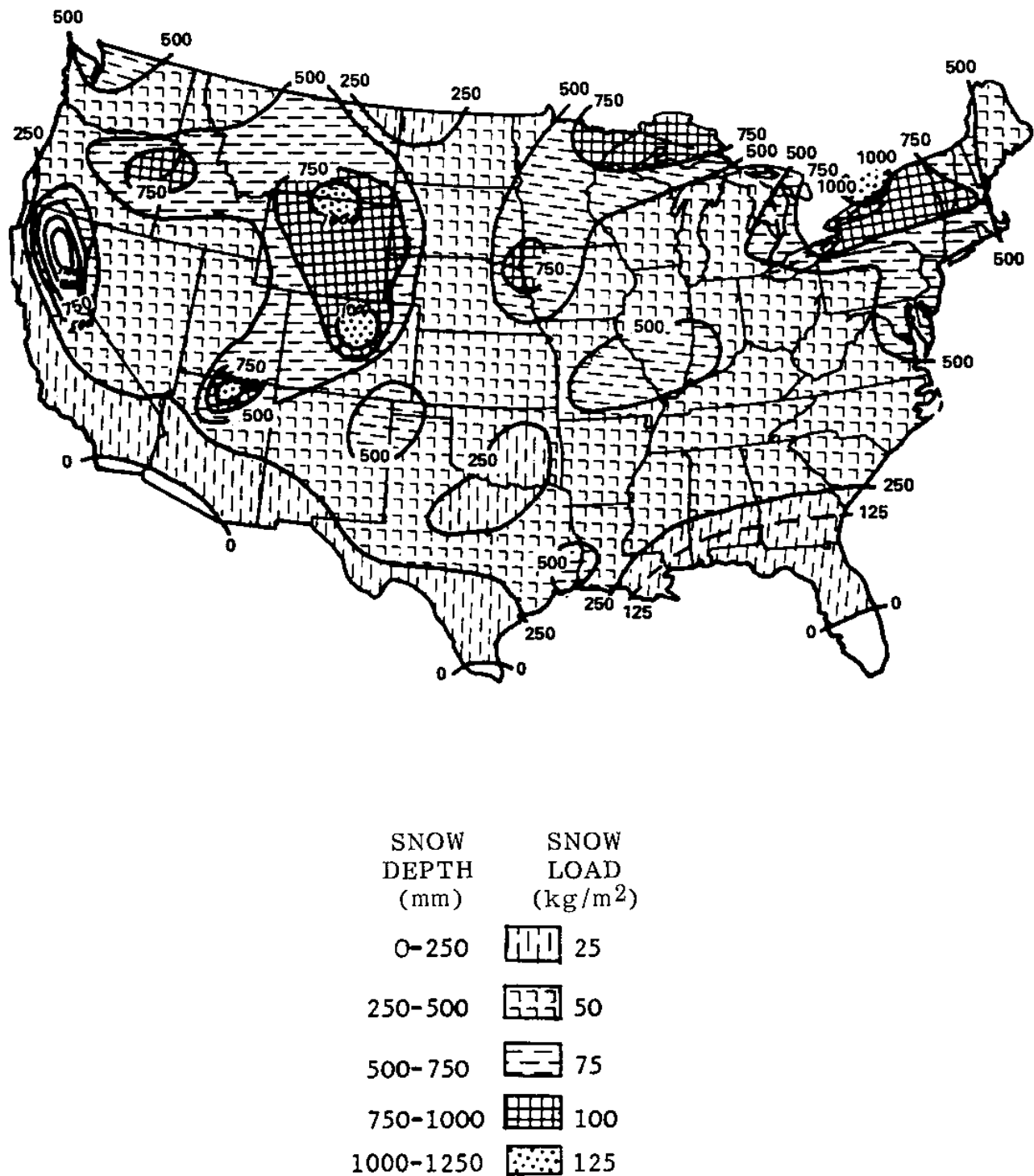
FIGURE 5.6 Extreme Storm Maximum Snowfall (mm) and Maximum Snow Load.
