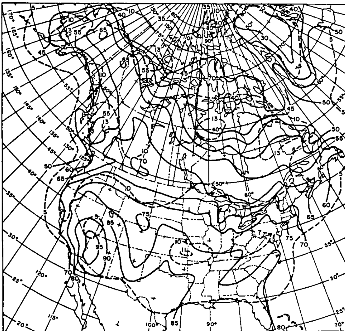
FIGURE 5.4 Isotherms of July Hourly Surface Temperatures. (Approximate Mean Values (°F) are Shown by Solid Lines, Standard Deviations (°F) By Broken Lines. The Approximations were Made to Yield the Best Estimates of Upper 80- to 99-Percentile Values by Normal Distribution (Ref. 5.3).
