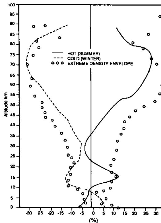
FIGURE 3.3 Relative Deviations (%) of Extreme VAFB Density Profiles with Respect to VRA-71.
