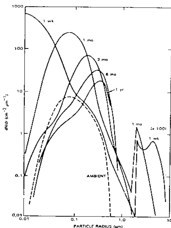
FIGURE 10-1. Evolution of the Volcanic Aerosol Size Distribution at 20 Km in the Simulated El Chichon Eruption Cloud. Size Distributions are Shown at Various Times, and are Compared to the Ambient Size Distribution (Ref. 10.6).
