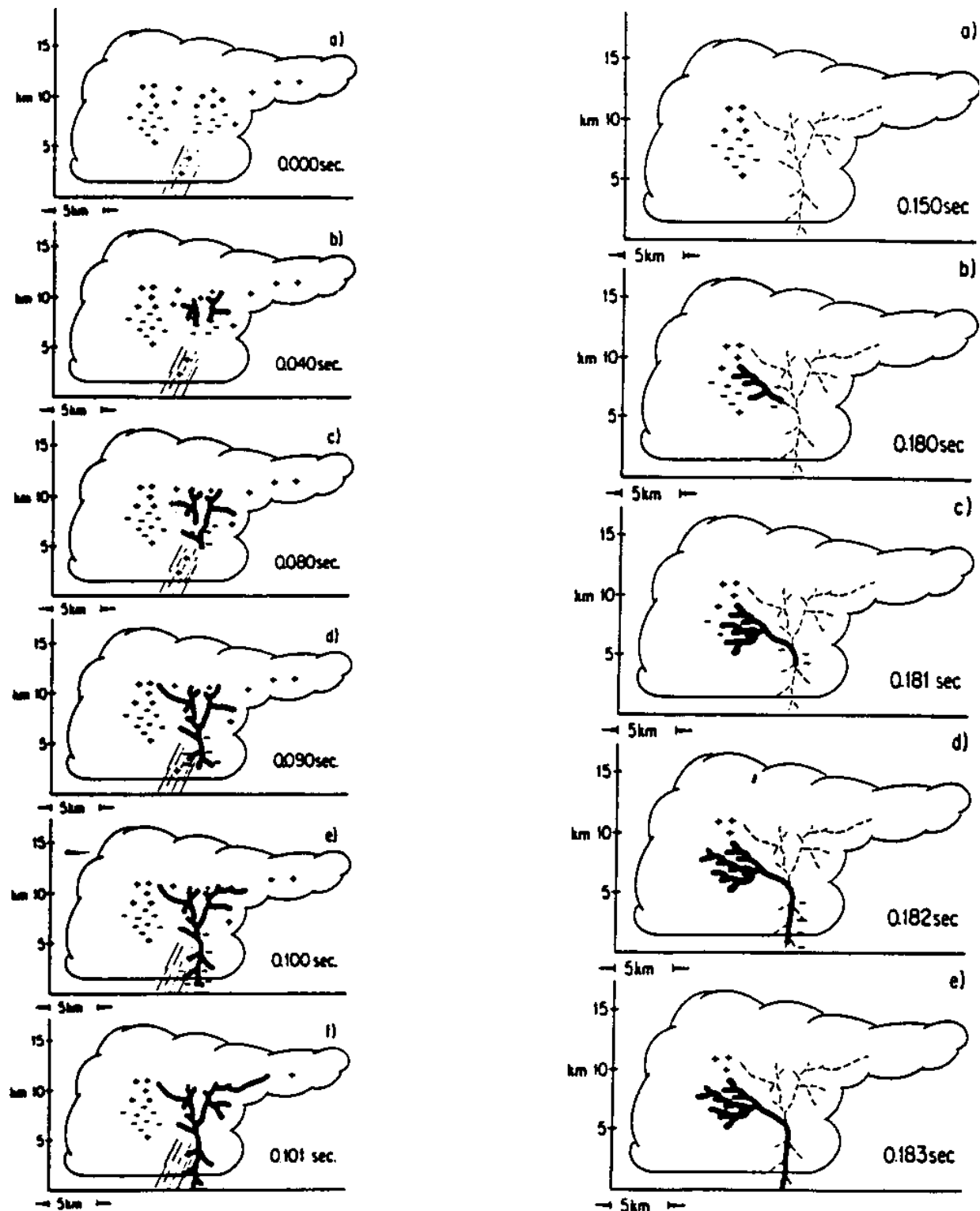
FIGURE 9.5. First Column is a Sketch of the Luminous Processes that Form the Stepped Leader and the First Return Stroke in a Cloud-To-Ground Lightning Flash. Second Column Shows the Development of a Lightning Dart-Leader and a Return Stroke Subsequent to the First in a Cloud-to-Ground Lightning (Ref. 9.22).
