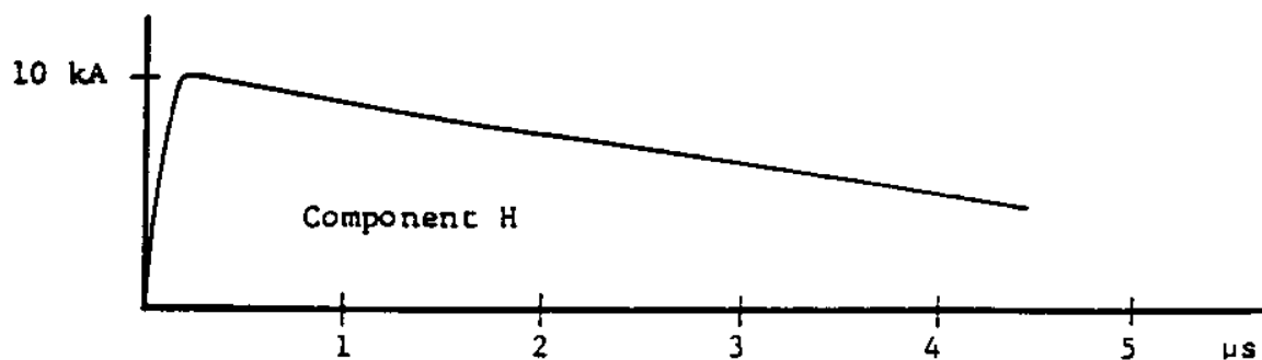
FIGURE 9.8 (Cont'd) The SAE 1987 Current Test Waveforms for Severe Direct Lightning Strikes to Aircraft (Ref. 9.5)
