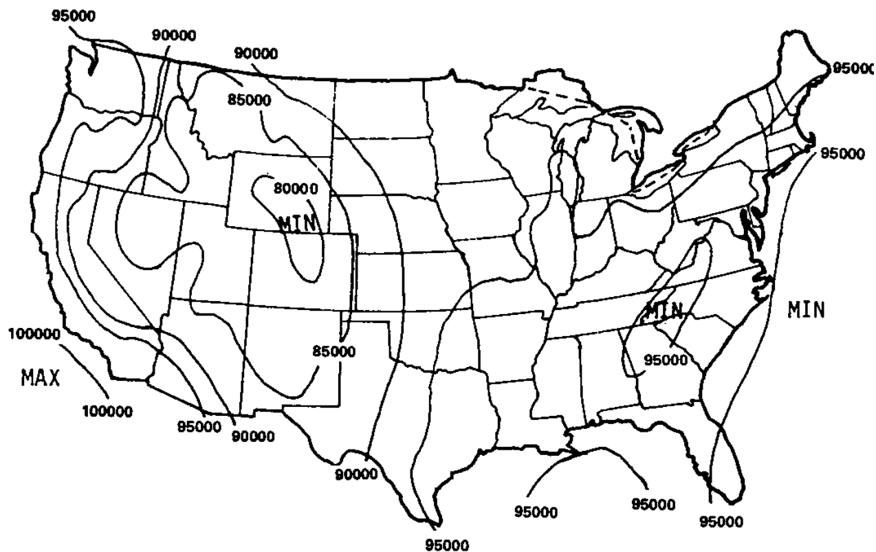
FIGURE 5.9 Maximum Absolute Station Pressure ( \text{N/m}^2 )
