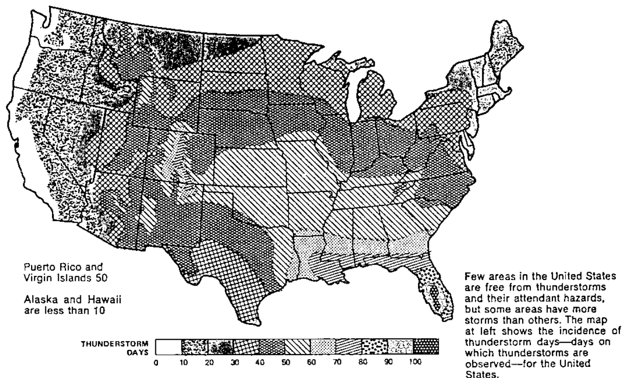
FIGURE 9.4 Incidence of Thunderstorm Days, Per Year (Ref. 9.17).
