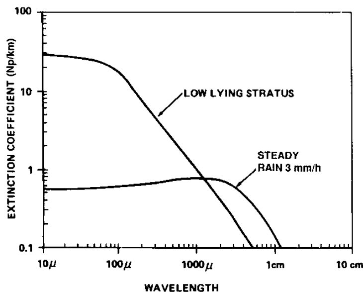
FIGURE 8.1 Extinction Coefficient as a Function of Wavelength.
