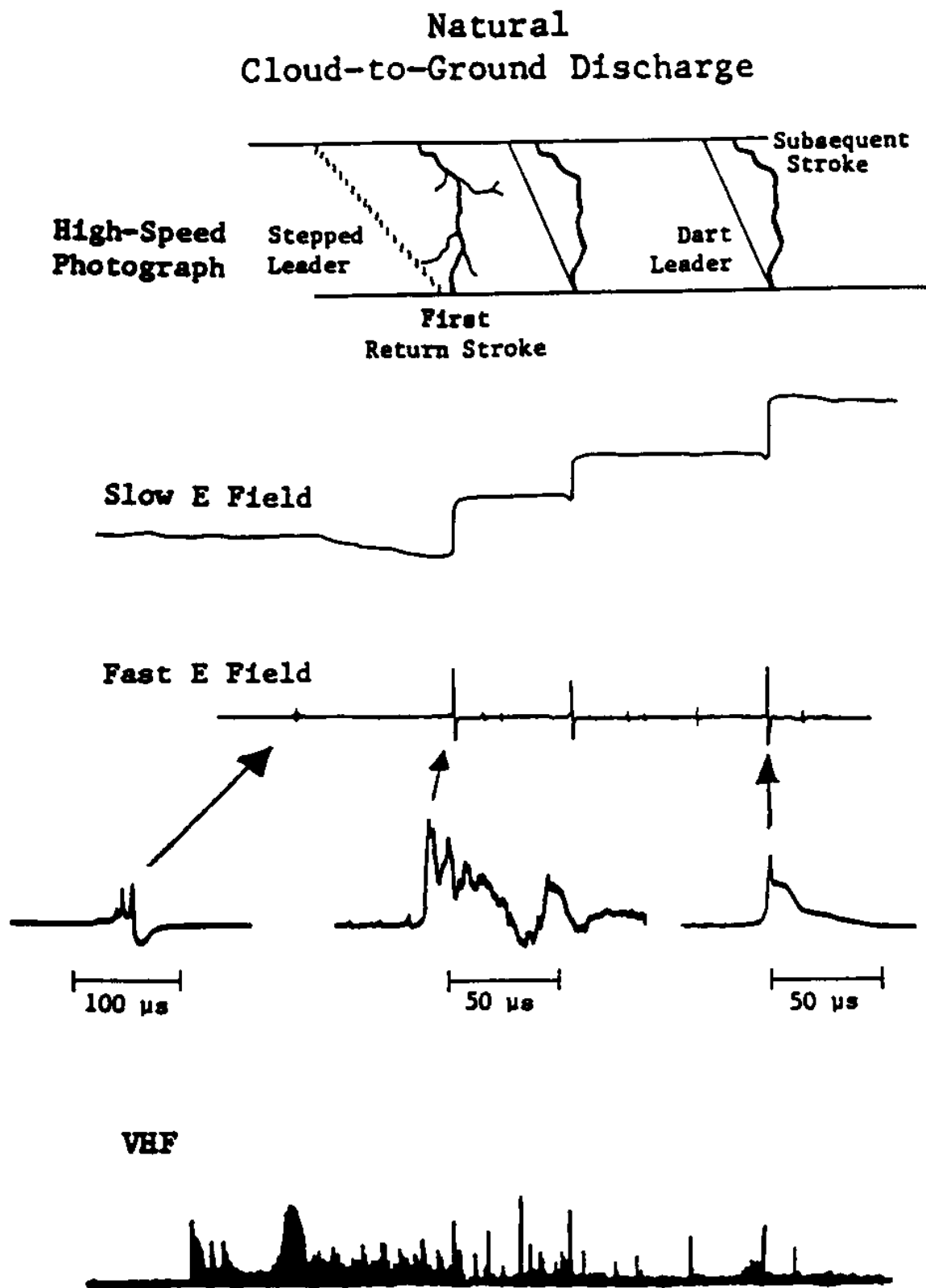
FIGURE 9.6 Simultaneous Photographic and Electric Field Measurements for a Multiple Stroke, Cloud-To-Ground Lightning Flash. The Schematic at the Bottom is an Example of a VHF Lightning Radiation Signature (Adapted From Ref. 9.10).
