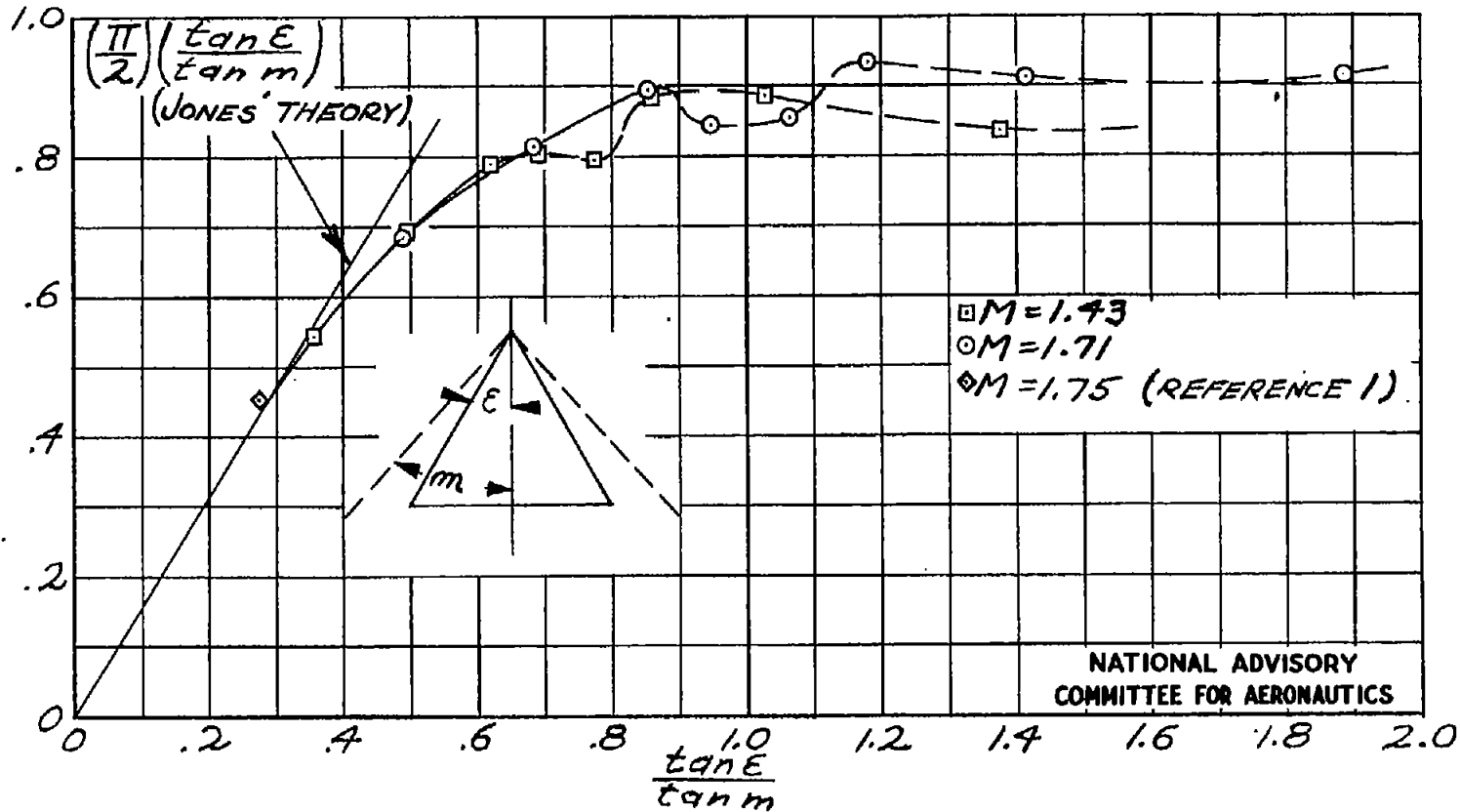
Figure 5.- Triangular wing lift curve slope results from figures 3 and 4.
