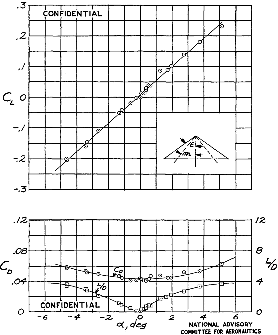
(a) Wing 1; R=340,000 Figure 4.- Triangular wing lift and drag test results for M=1.71 .
