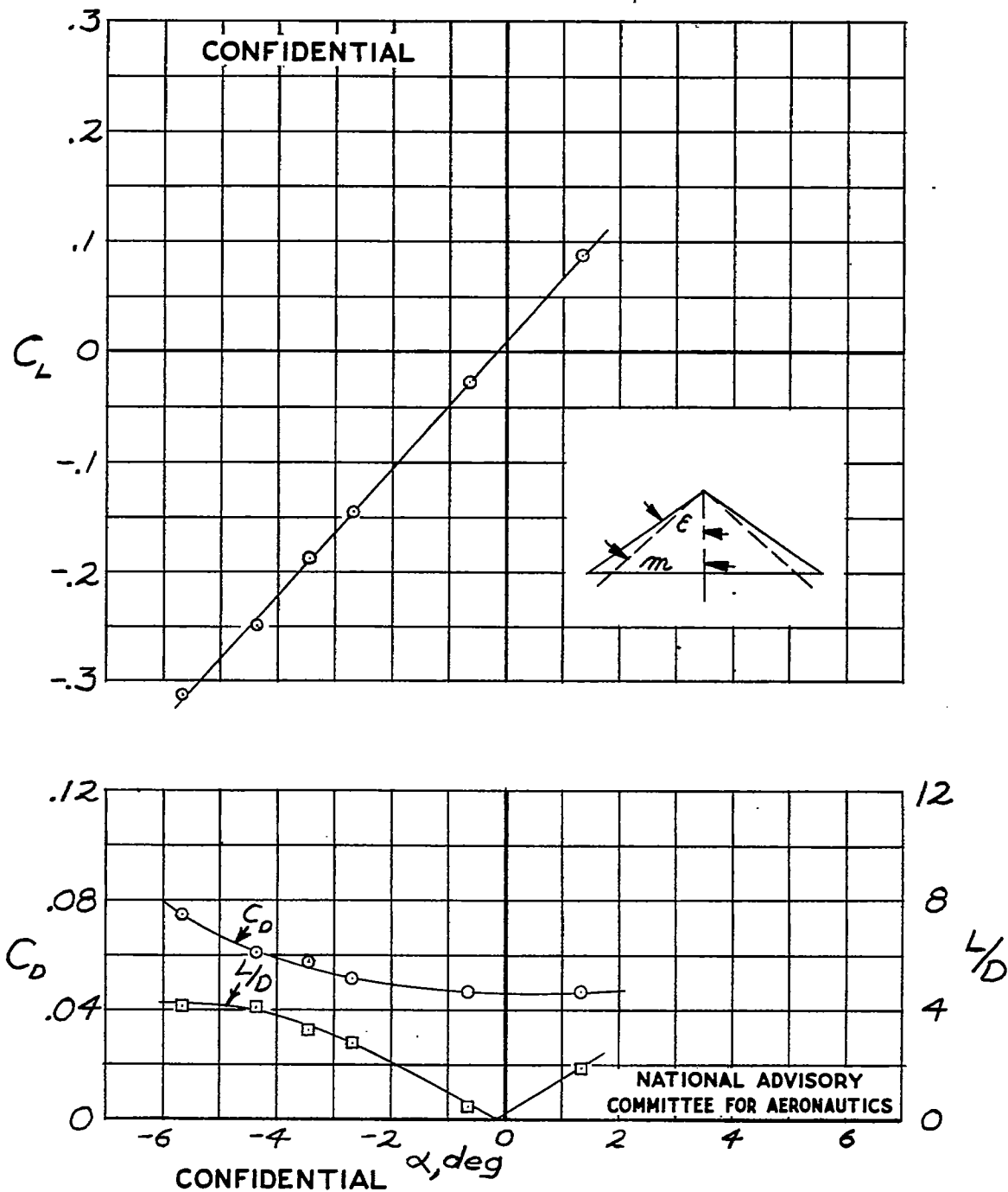
(a) Wing 1; R=360,000 Figure 3.- Triangular wing lift and drag test results for M=1.43 .
