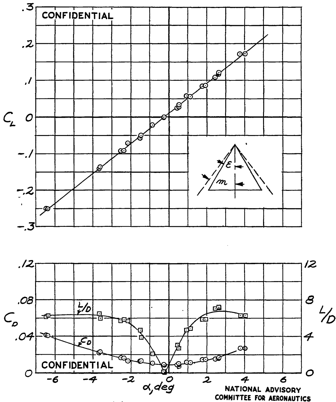
(g) Wing 7; R = 760,000 Figure 4.- Continued.
