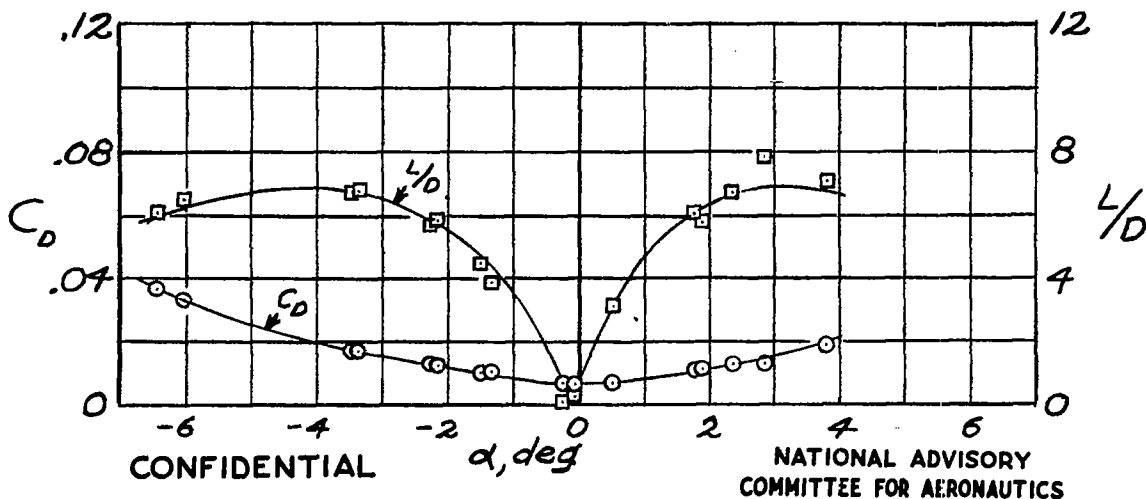
(h) Wing 8; R=940,000 Figure 4.- Concluded.
