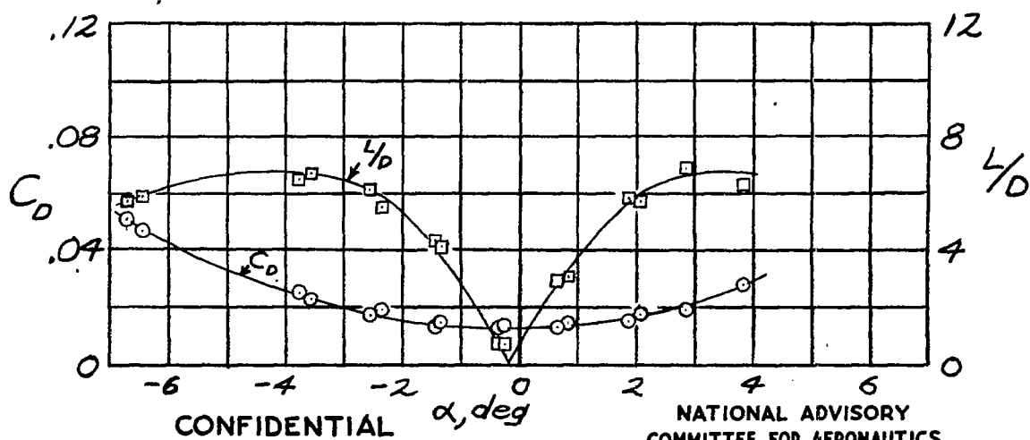
(f) Wing 6; R = 660,000 Figure 4.- Continued.
