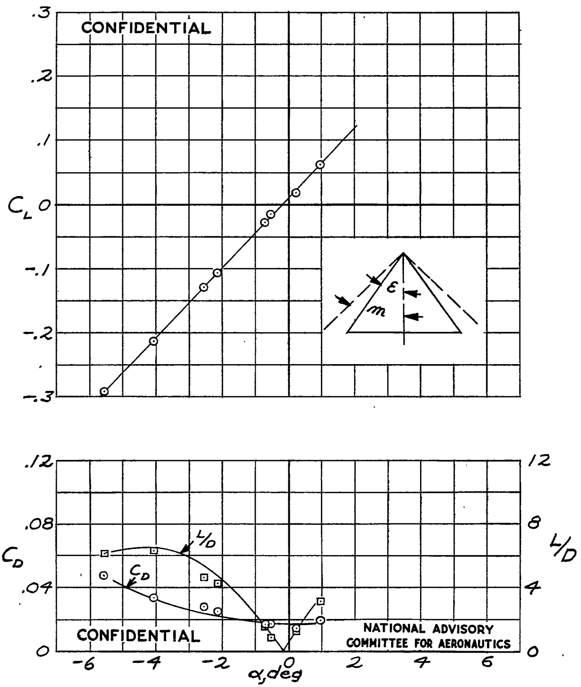
(e) Wing 5; R = 640,000 Figure 3.- Continued.
