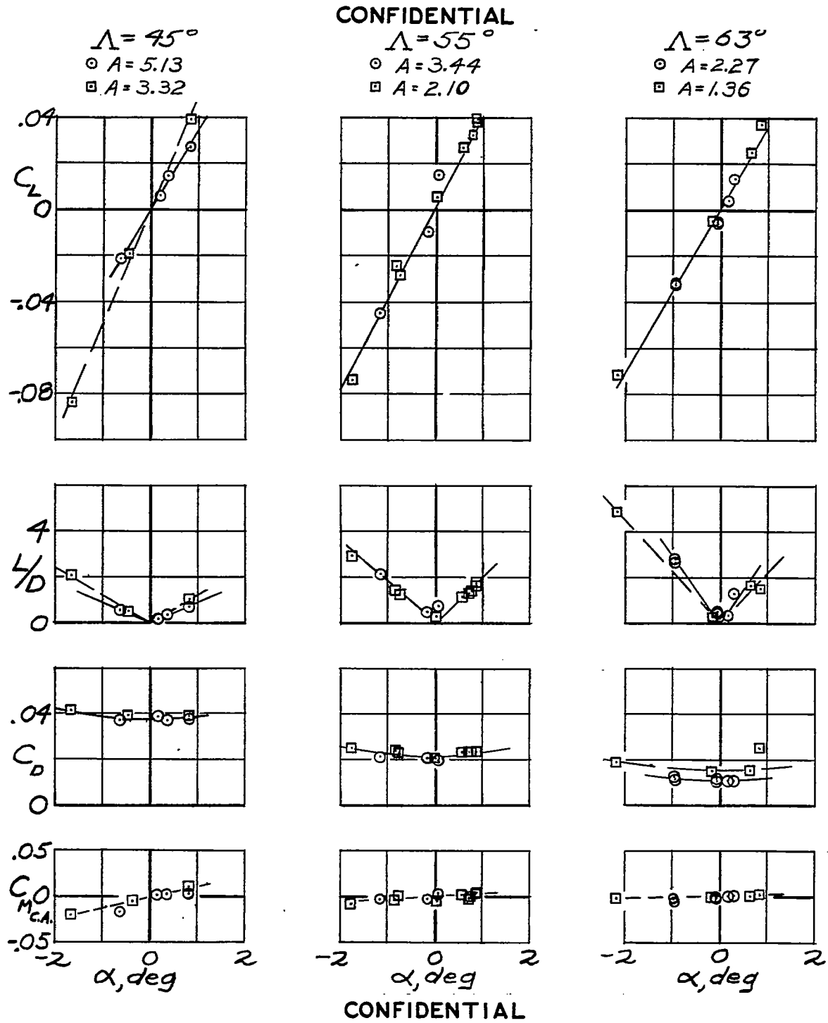
Figure 9.- Sweptback wing test results for M = 1.43 . NATIONAL ADVISORY COMMITTEE FOR AERONAUTICS
