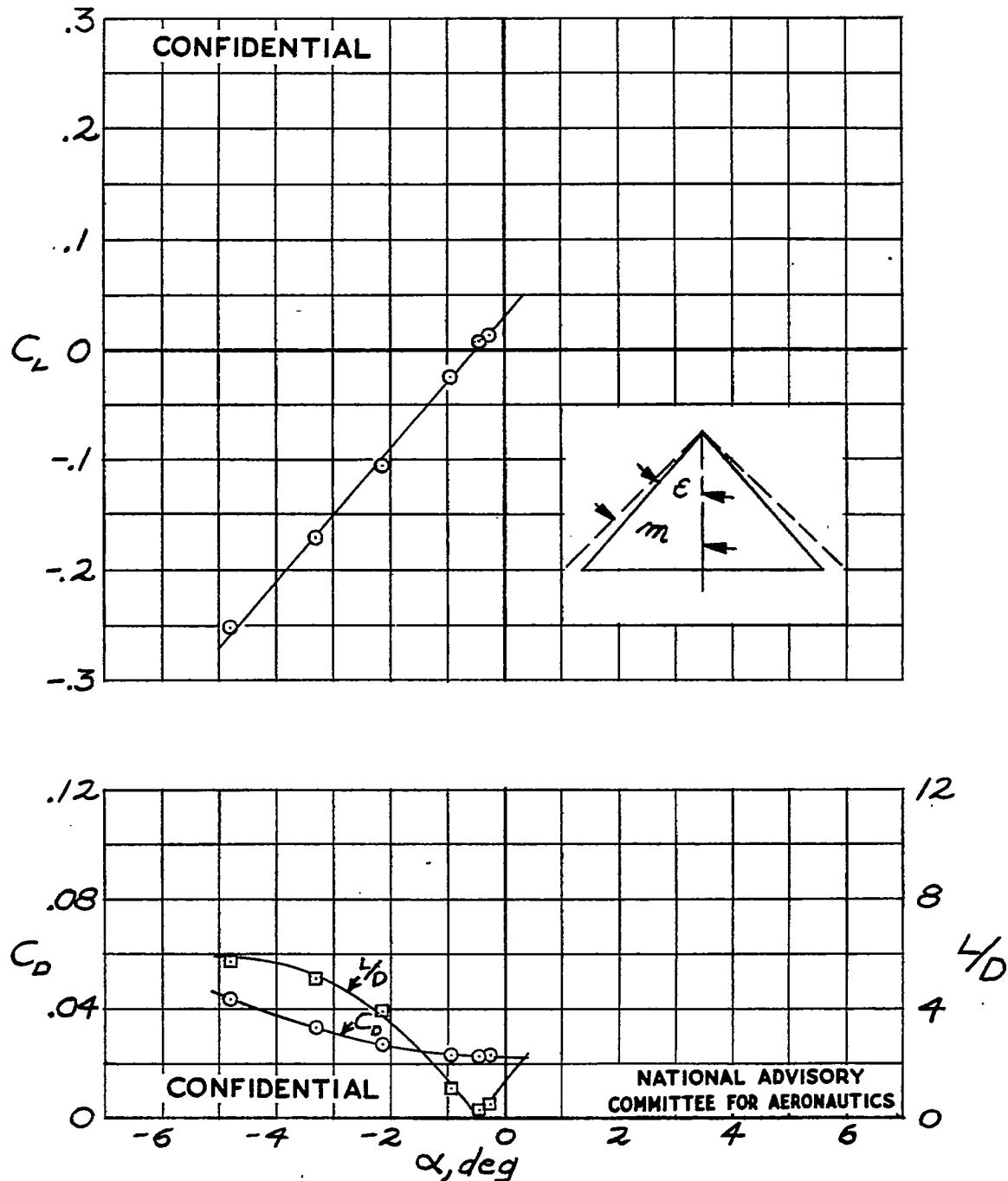
(c) Wing 3; R=540,000 Figure 3.- Continued.
