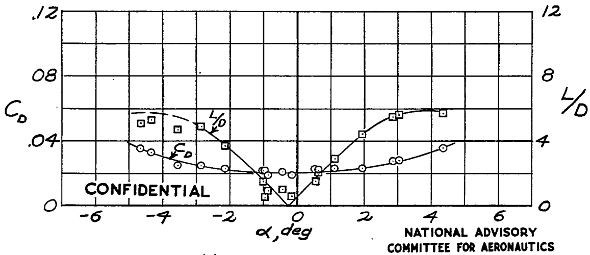
(c) Wing 3; R=520,000 Figure 9.- Continued.
