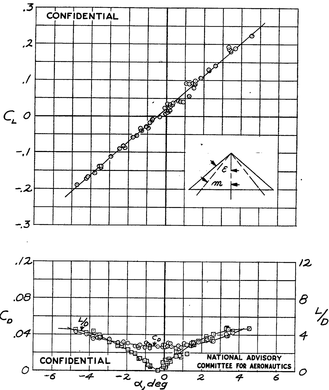
(b) Wing 2; R = 440,000 Figure 4.-Continued.
