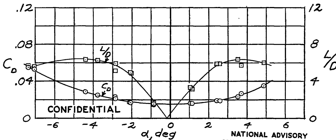
(e) Wing 5; R = 620,000 Figure 4. - Continued.
