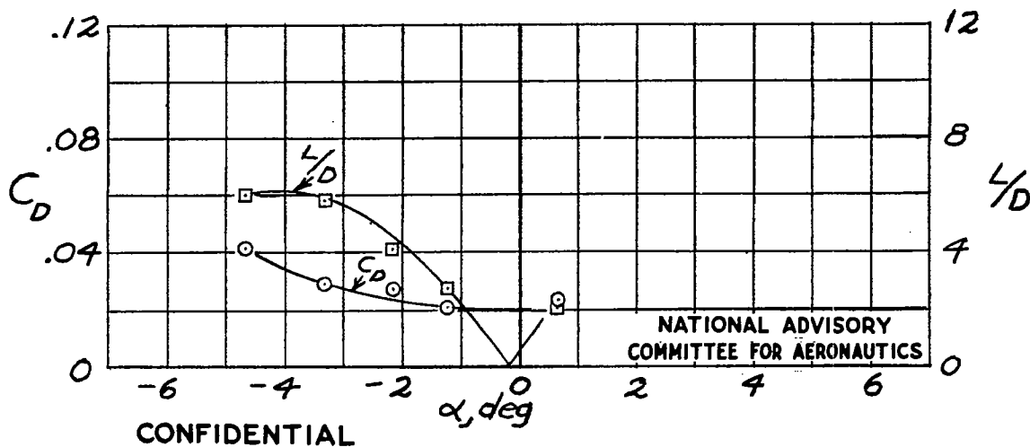
(d) Wing 4; R = 600,000 Figure 3.-Continued.
