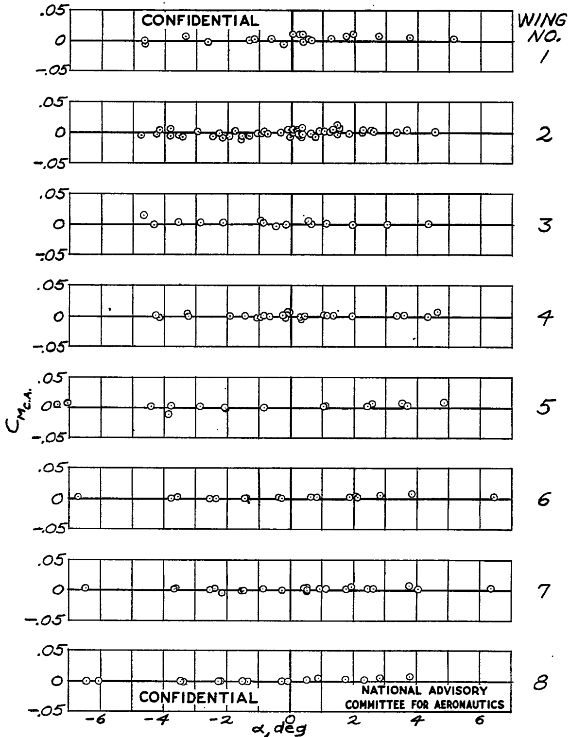
Figure 7.- Triangular wing moment test results for M=1.71 .
