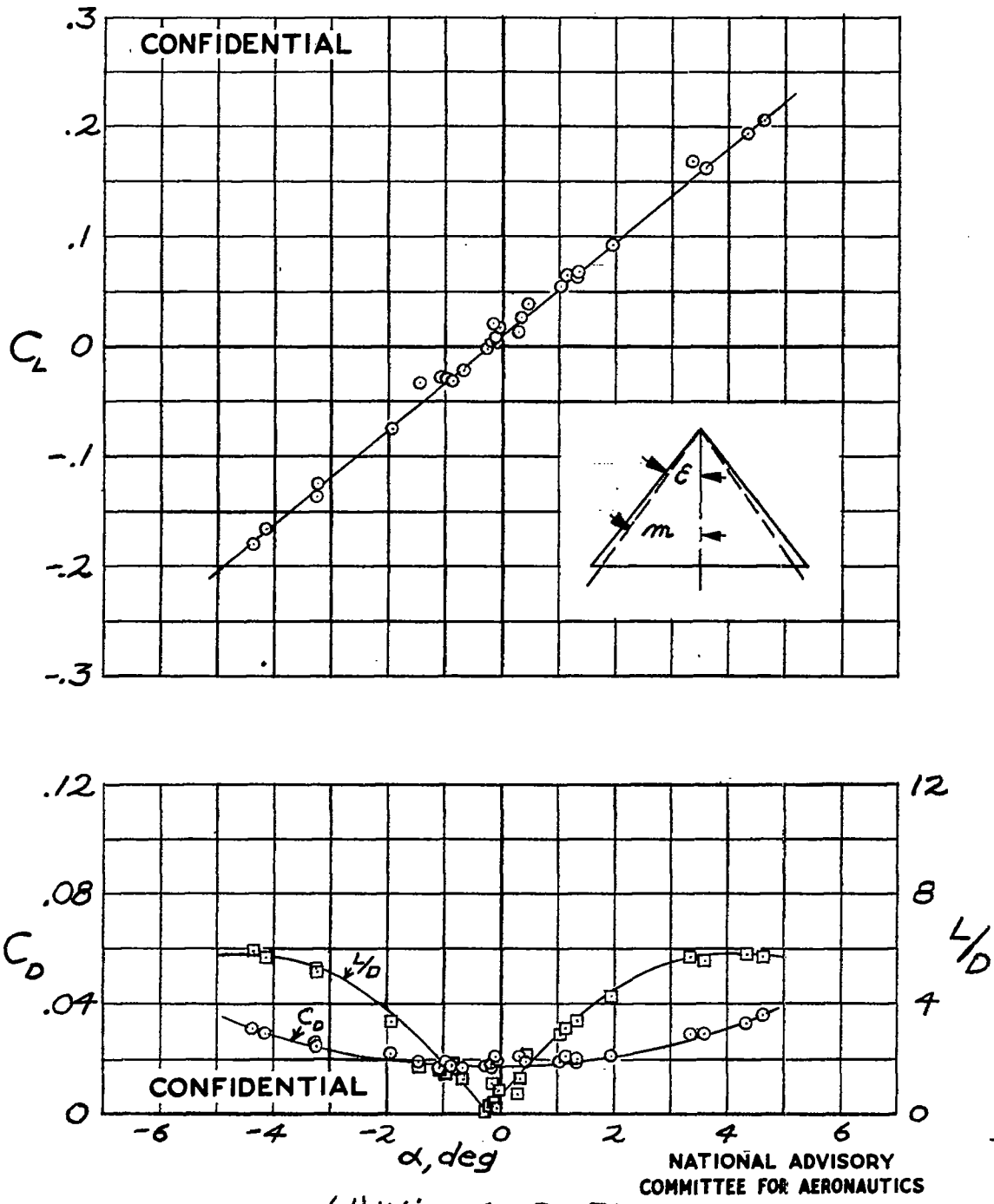
(d) Wing 4; R=560,000 Figure 4. - Continued.
