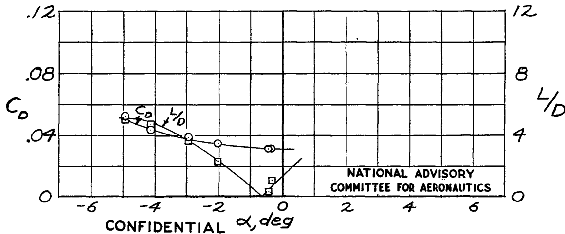
(b) Wing 2; R = 480,000 Figure 3.- Continued.
