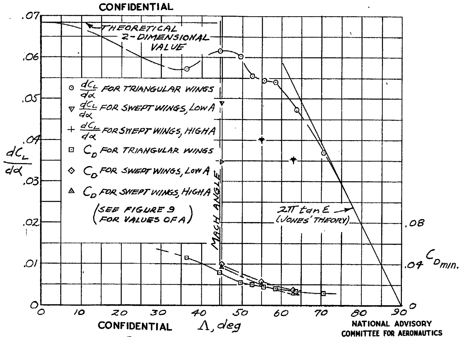
Figure 10.- Comparison of lift and drag results for triangular and sweptback wings at M = 1.43 .
