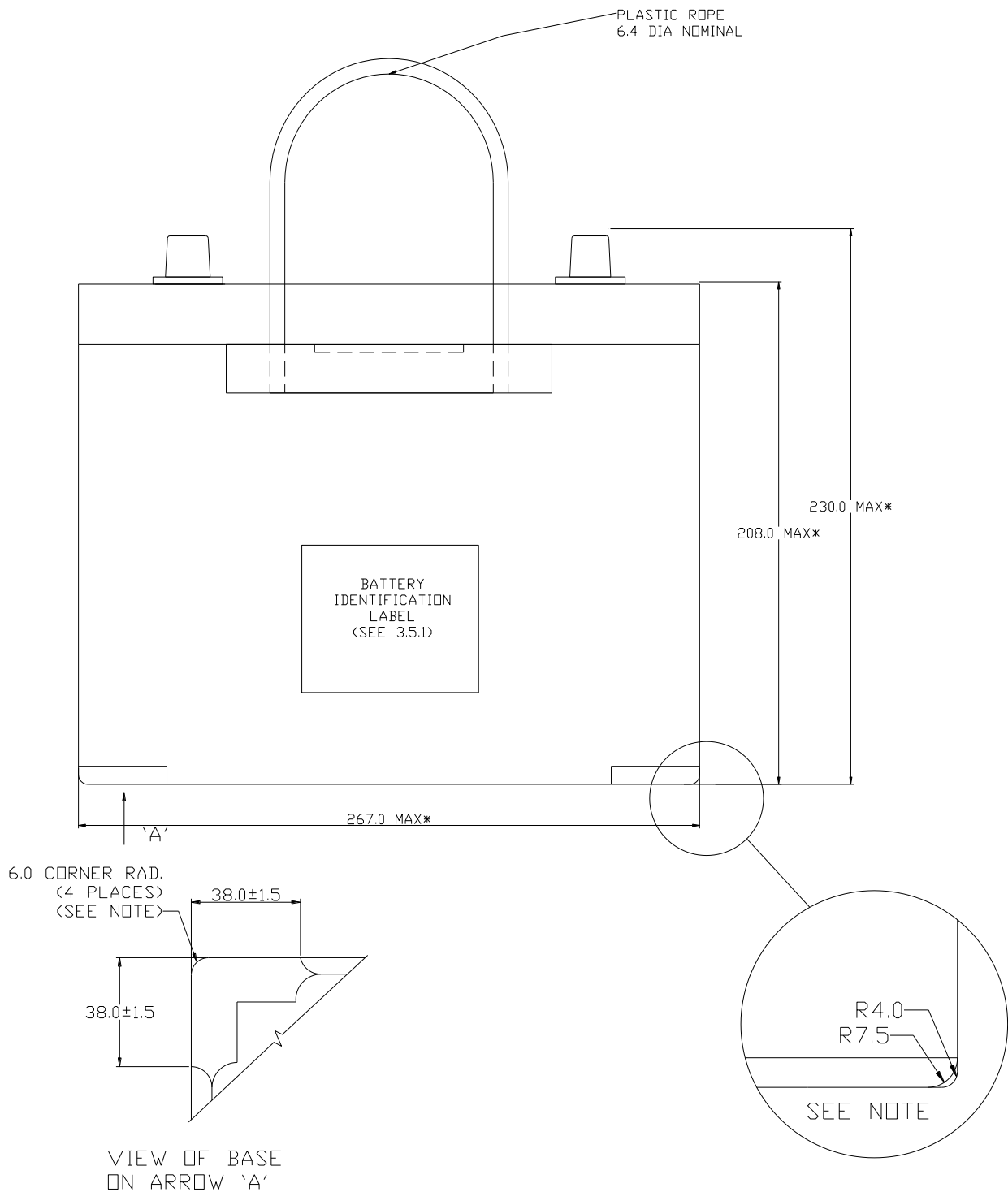
FIGURE A-5. Side view dimensions of battery.
