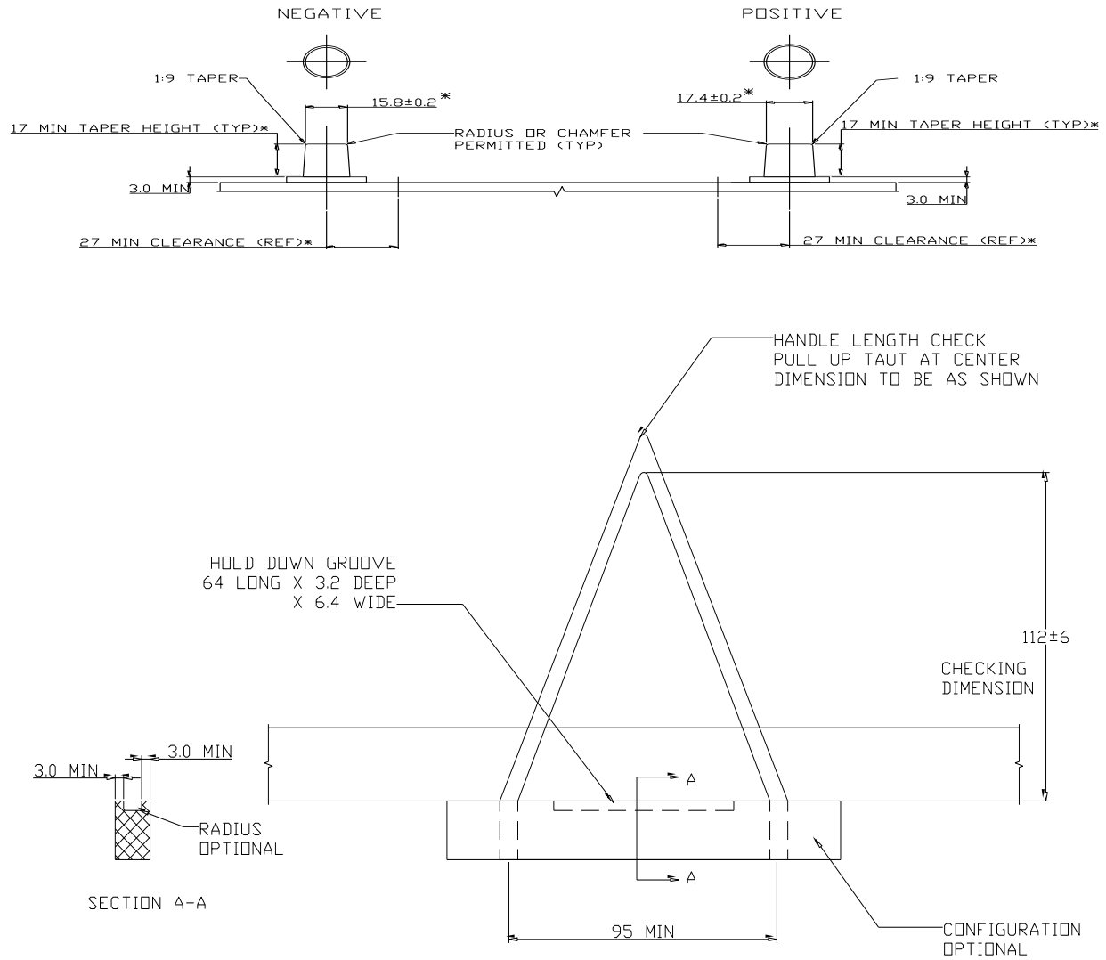
FIGURE A-6. Handle and post details.
