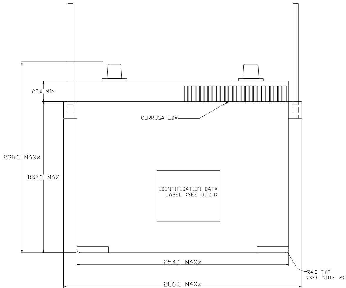
FIGURE A-4. Front view dimensions of battery.
