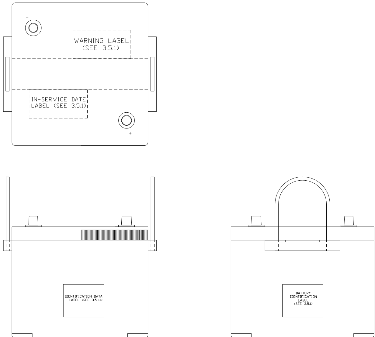
FIGURE A-2. Battery overview.
