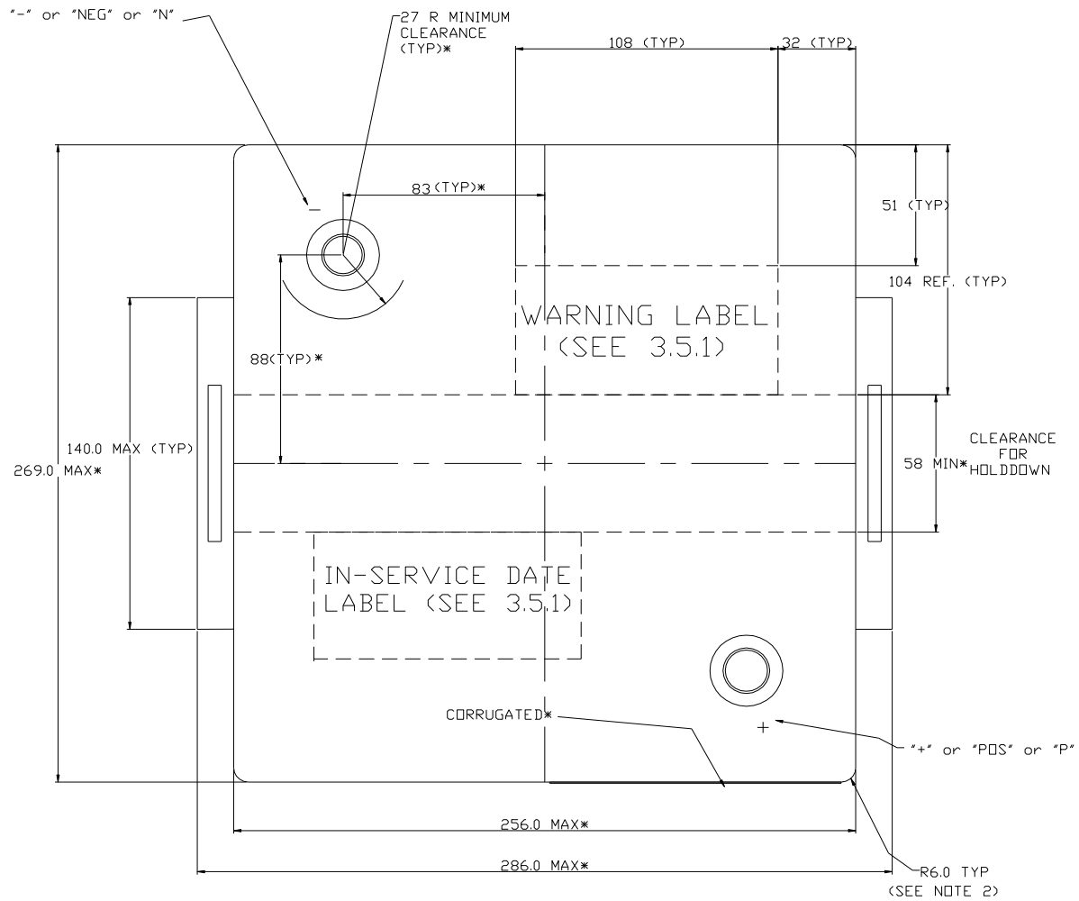
FIGURE A-3. Top view dimensions of battery.
