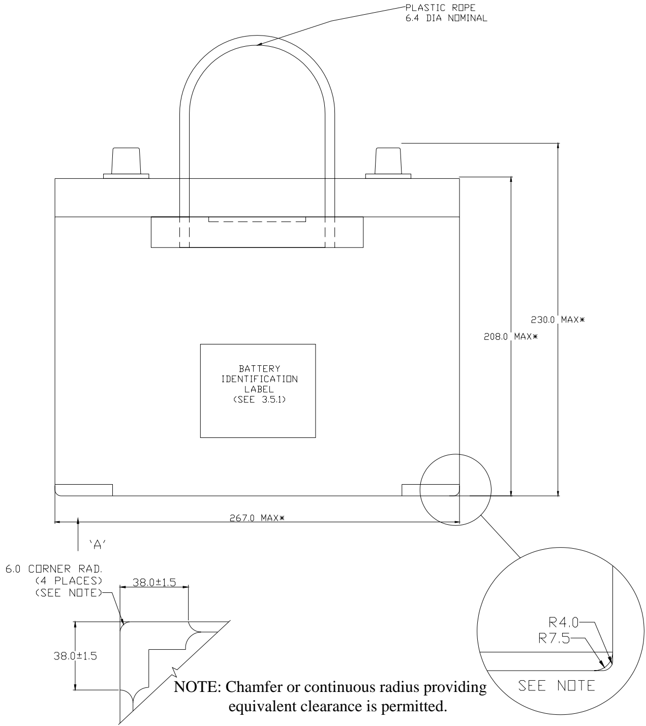
VIEW OF BASE ON ARROW 'A' FIGURE A-5. Side view dimensions of battery.
