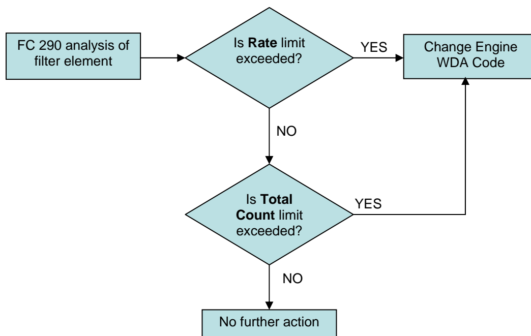
Figure 31: Proposed FC 290 Limit Logic
