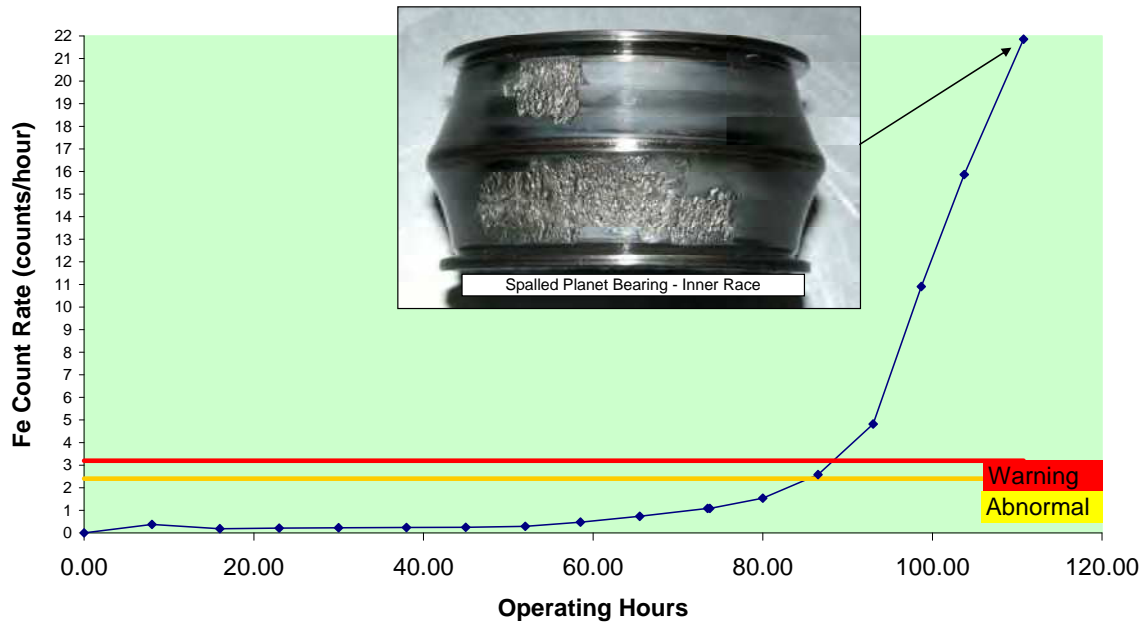
HTTF Metalscan Data with Overlaid Limits
