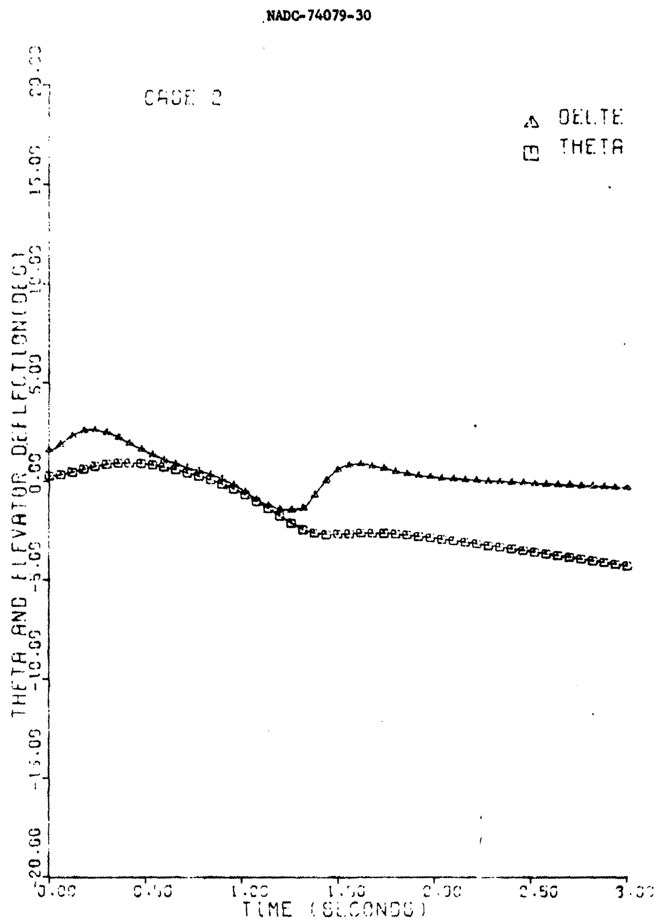
Figure 13. MQM-74C Pitch Attitude and Elevator Deflection Time History
