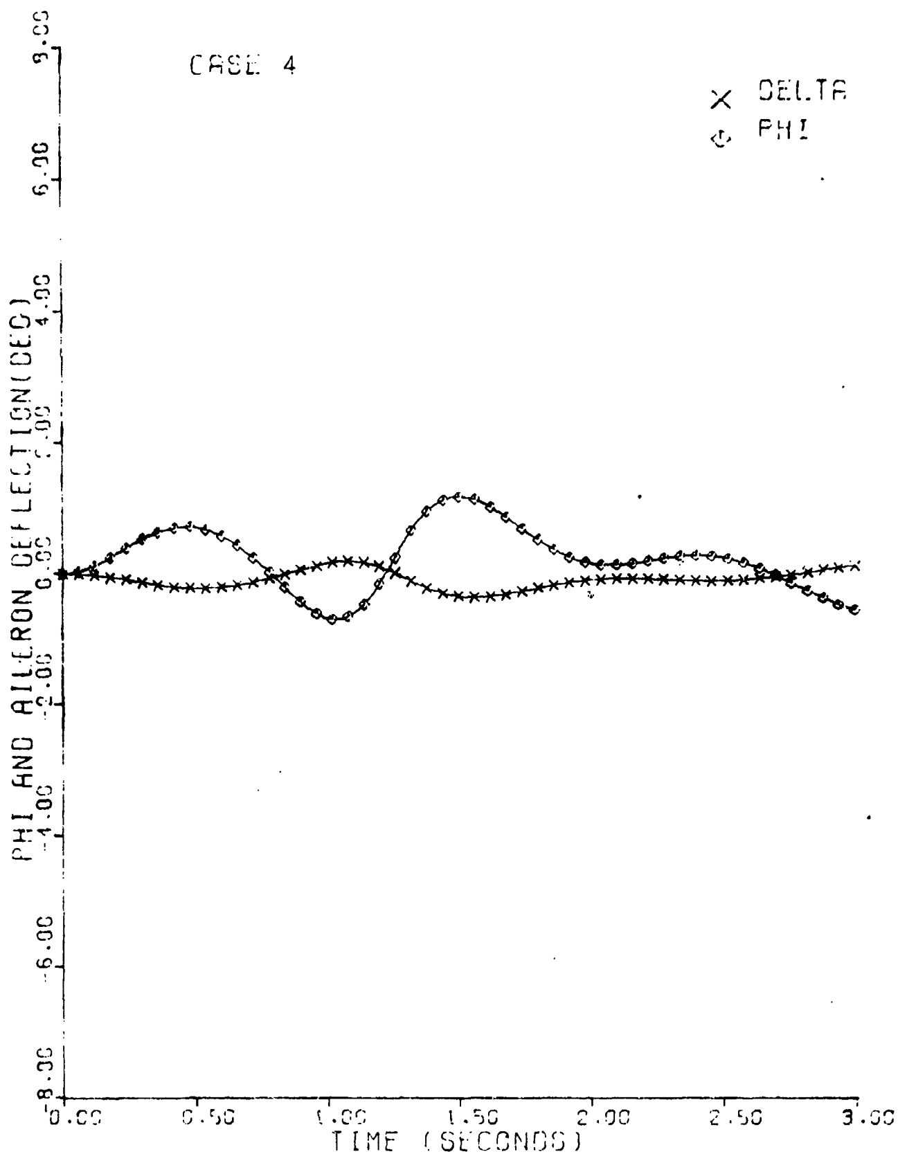
Figure 26. MQM-74C Roll Angle and Aileron Time History
