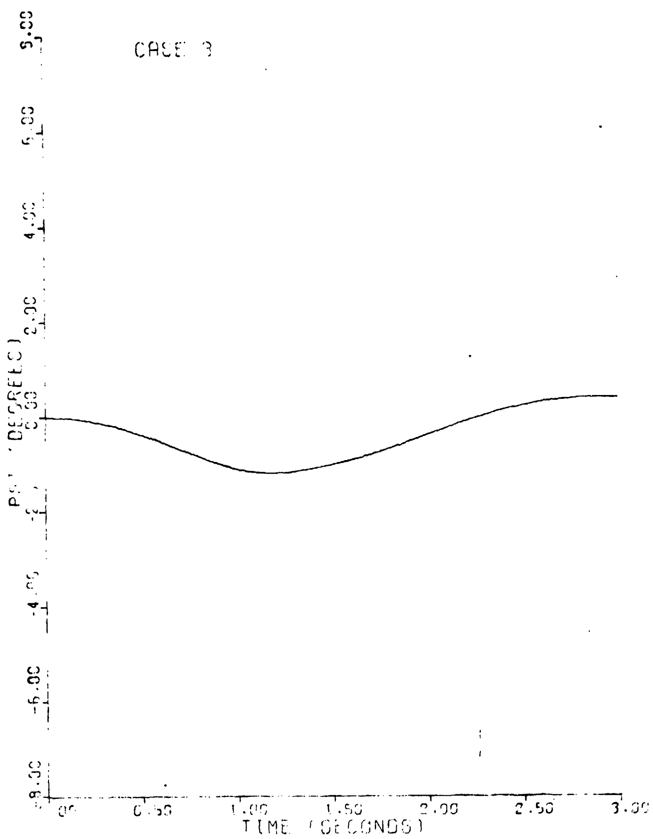
Figure 17. MQM-74C Yaw Time History 23
