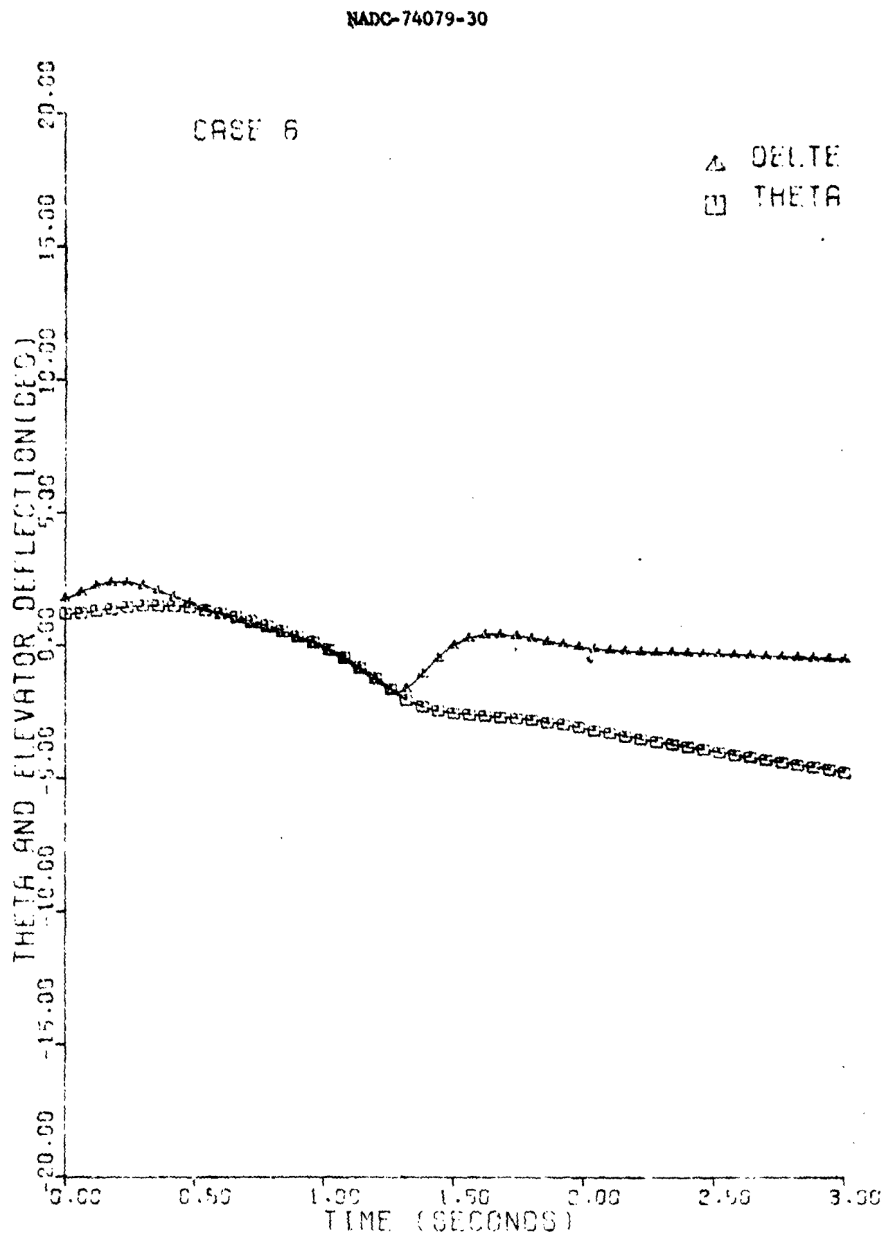
Figure 37. MQM-74C Pitch Attitude and Elevator Deflection Time History
