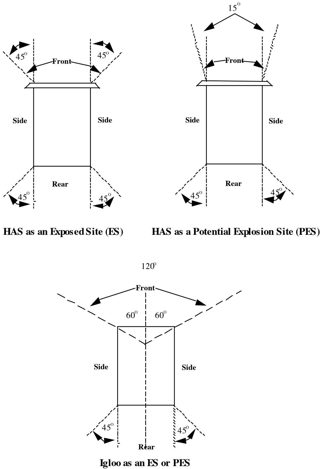
Figure 3.4. Hazard Zones for Hardened Aircraft Shelters and Igloos.
