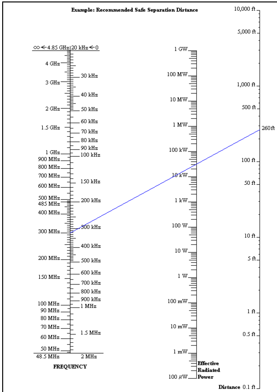
Figure 9.3. Example: Recommended SSD for HERO SUSCEPTIBLE Munitions; —Expsed” Configuration.
