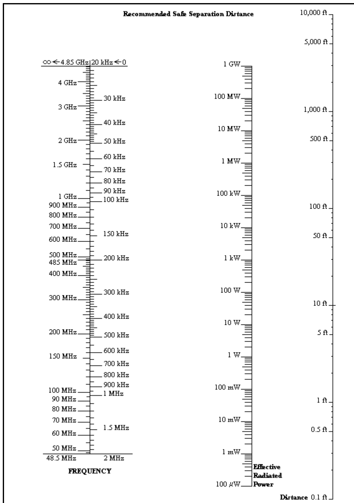
Figure 9.2. Recommended SSD for HERO SUSCEPTIBLE Munitions; —Expsed” Configuration.
