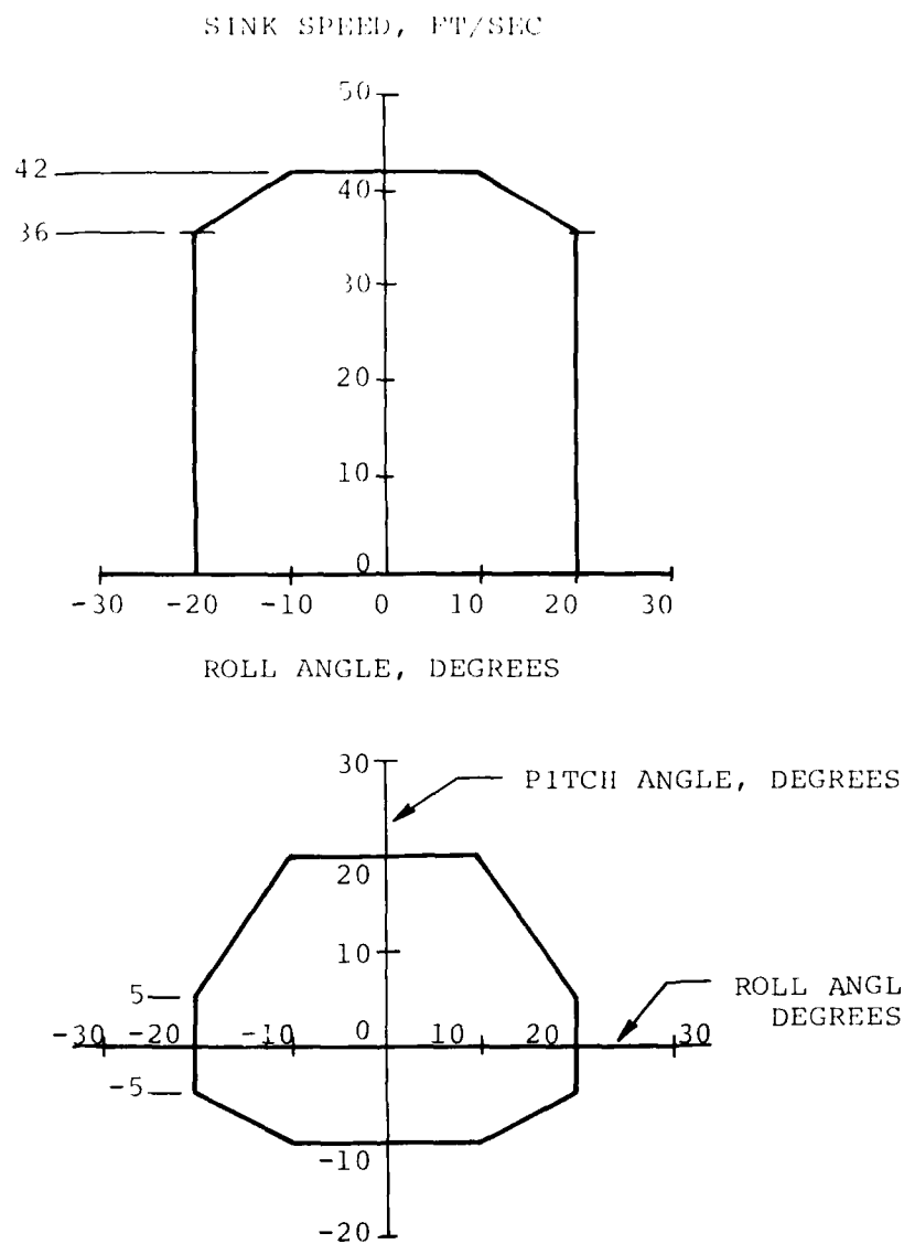
Figure B-1. Crash impact conditions.
