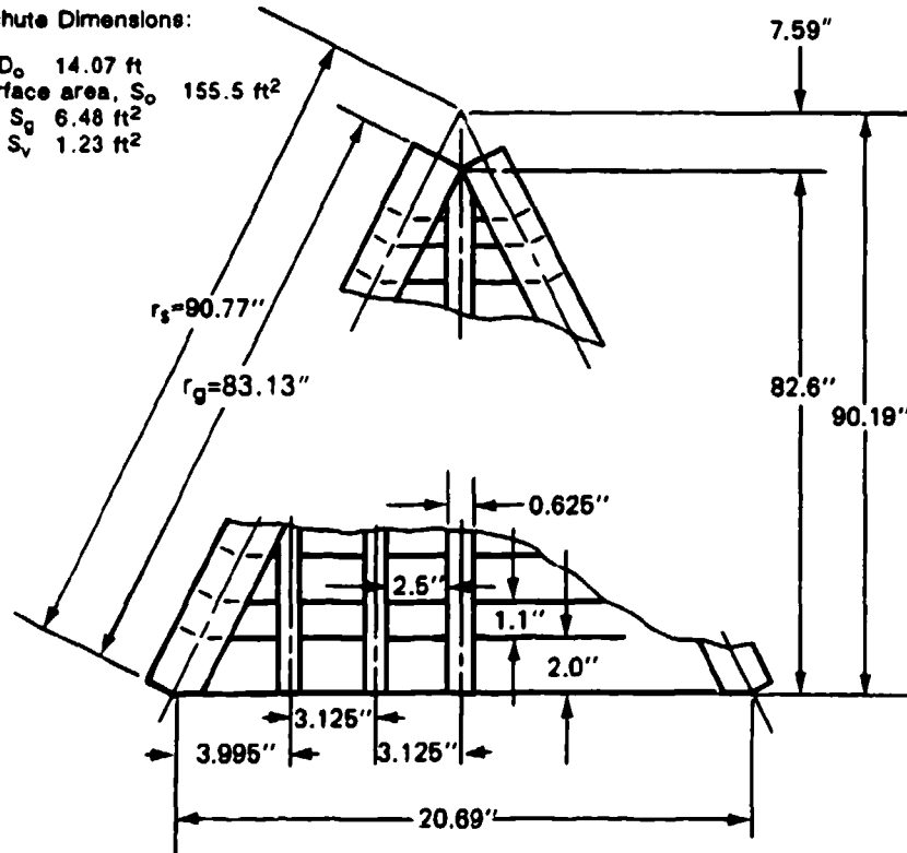
FIGURE 7-22. Final Gore Dimensions.
