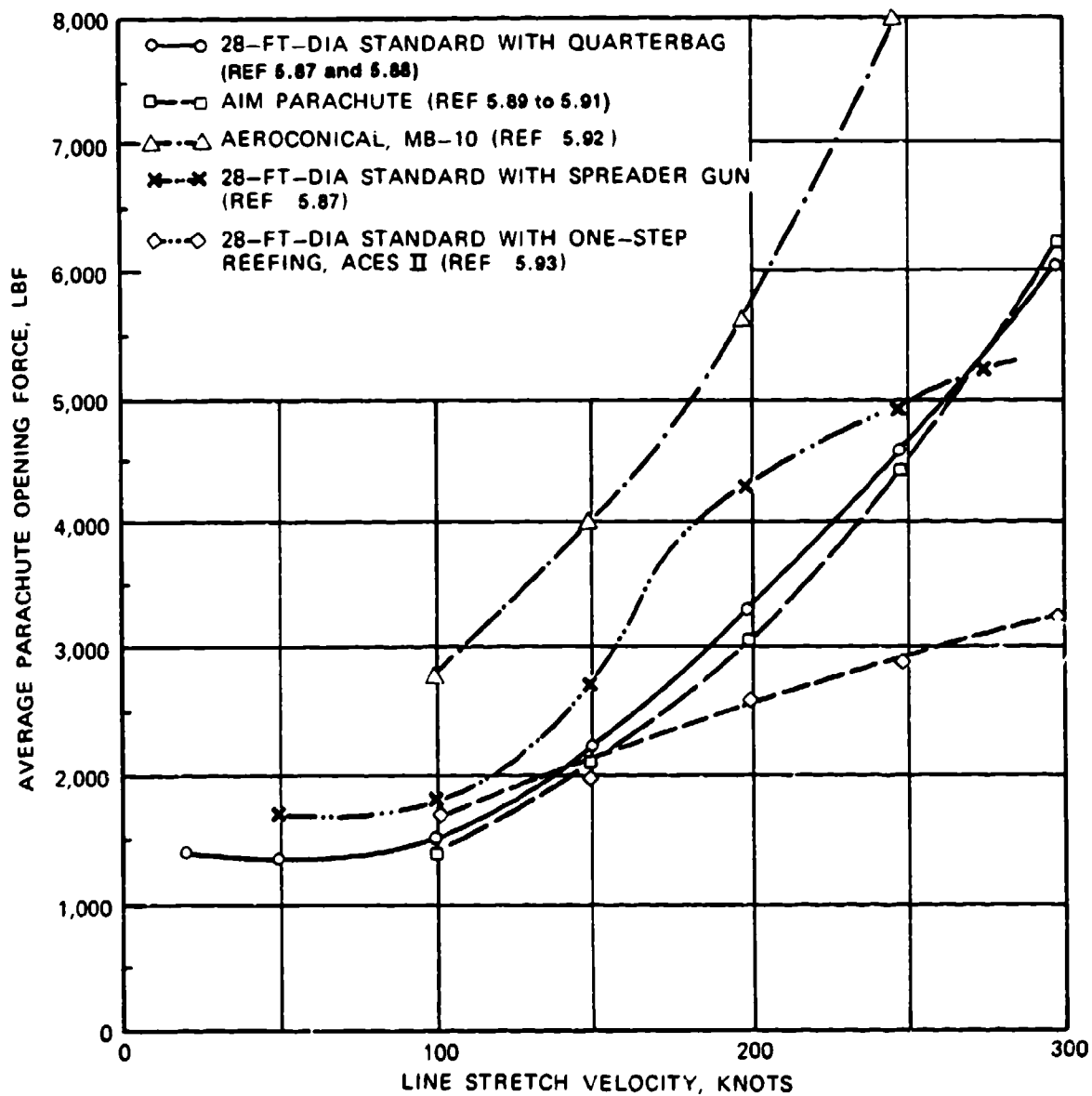
FIGURE 5-53. Opening Forces of Various Personnel Parachutes.
