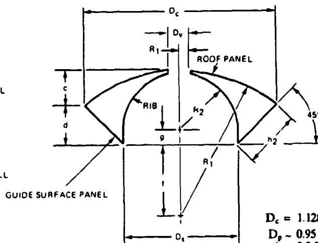
RIB LAYOUT
