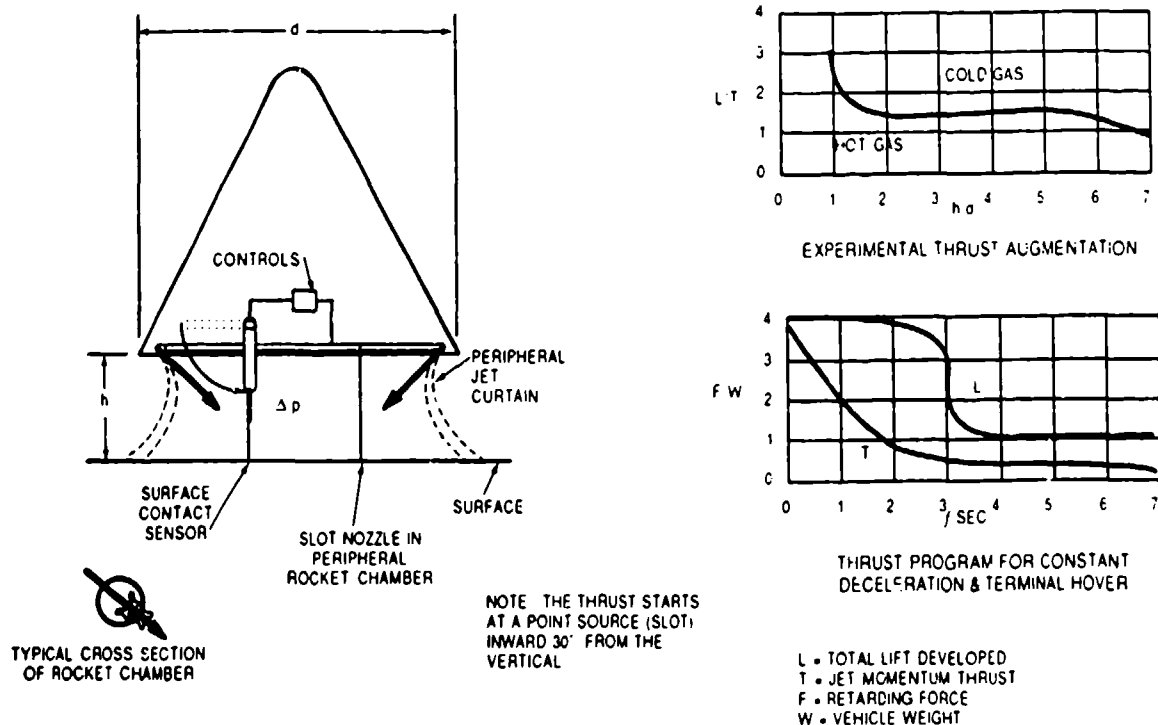
FIGURE 6-84. Design and Performance Details of the Skirt Jet Retrorocket System.
