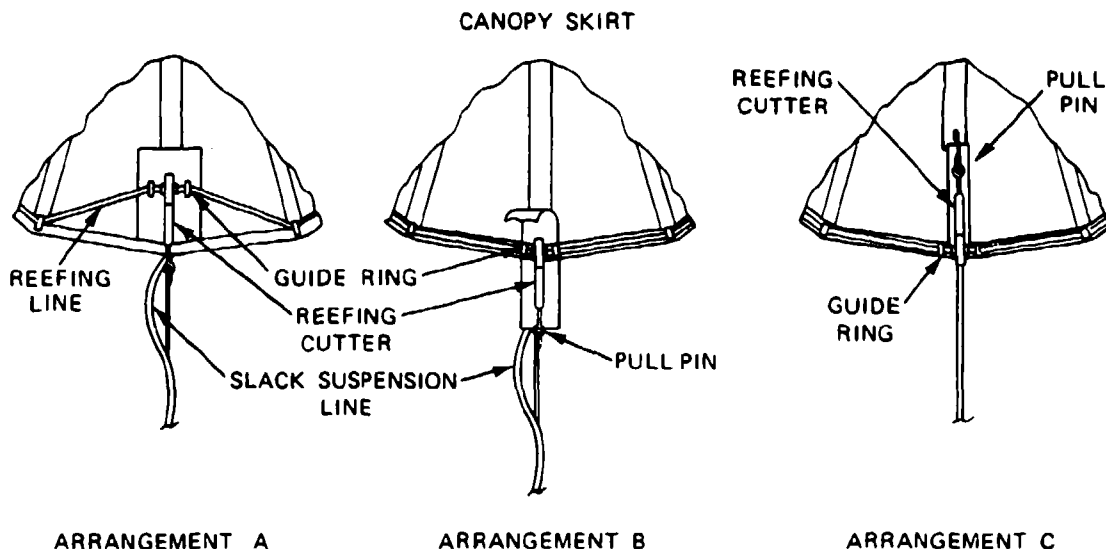
FIGURE 6-44. Three Methods of Reefing Cutter Installation.
