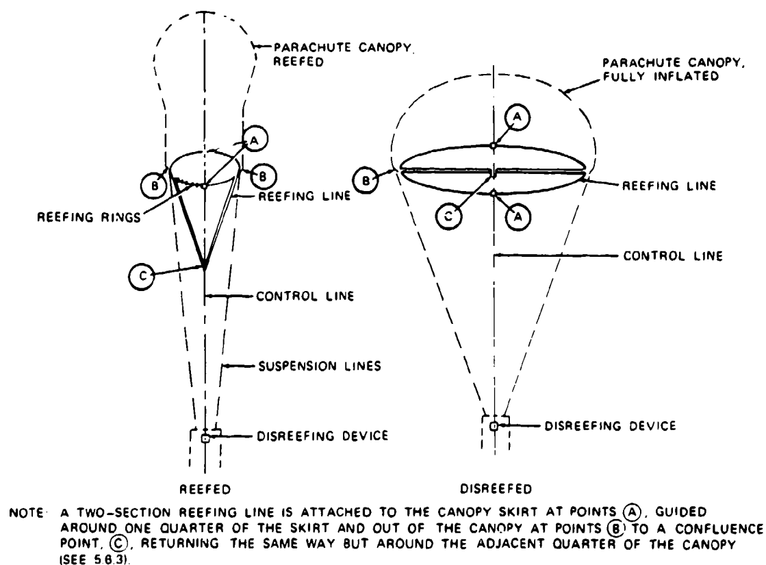
FIGURE 5-67. Parachute Skirt Reefing With Control Line.
