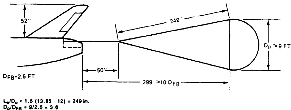
FIGURE 7-18. Drogue Chute Arrangement.
