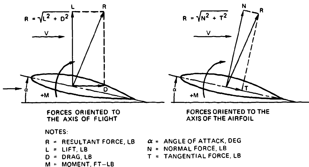
FIGURE 4-7. Aerodynamic Forces Acting on an Airfoil.
