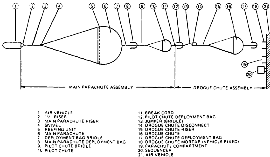
FIGURE 6-11. Typical Parachute Recovery System.
