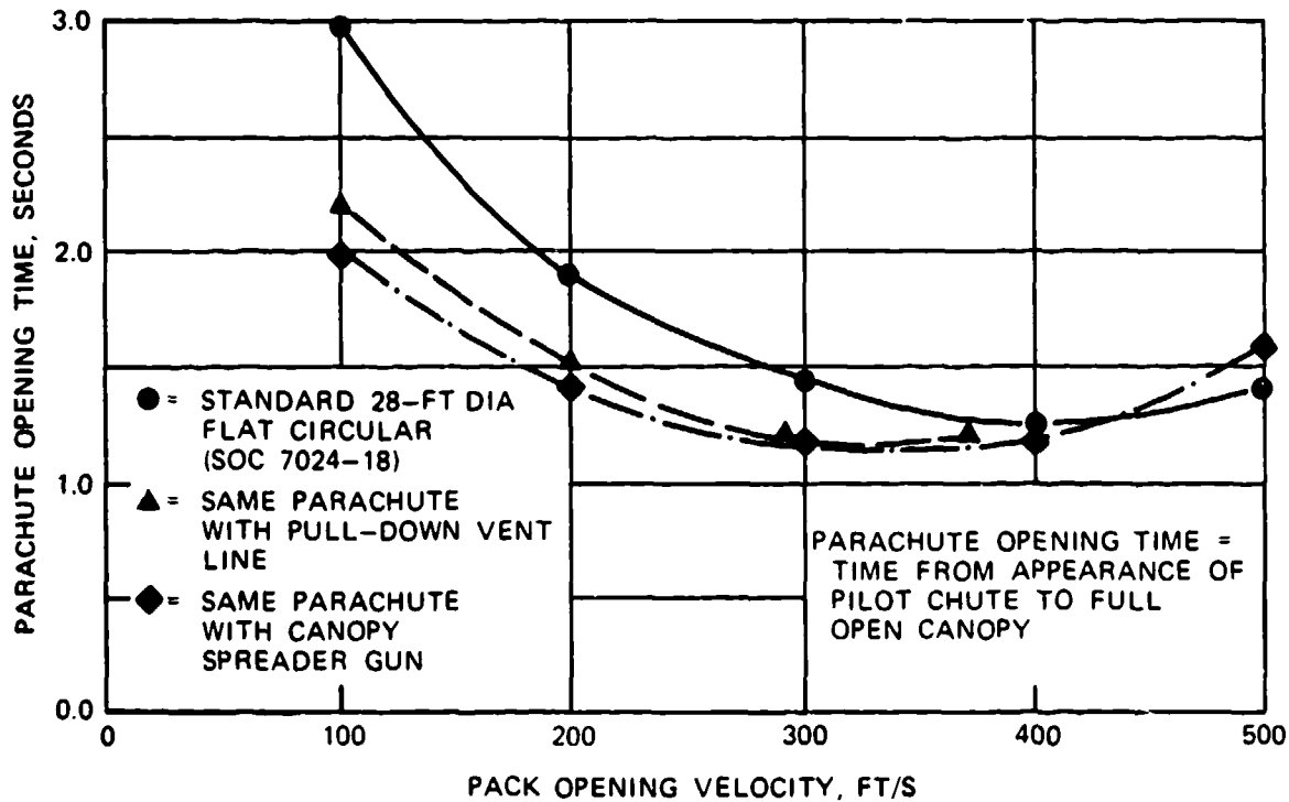
FIGURE 5-55. Opening Time Comparison of Three Configurations of the 28-Foot-Diameter Personnel Parachute: Standard, Standard With Pull-Down Vent Line, and Standard with Spreader Gun.
