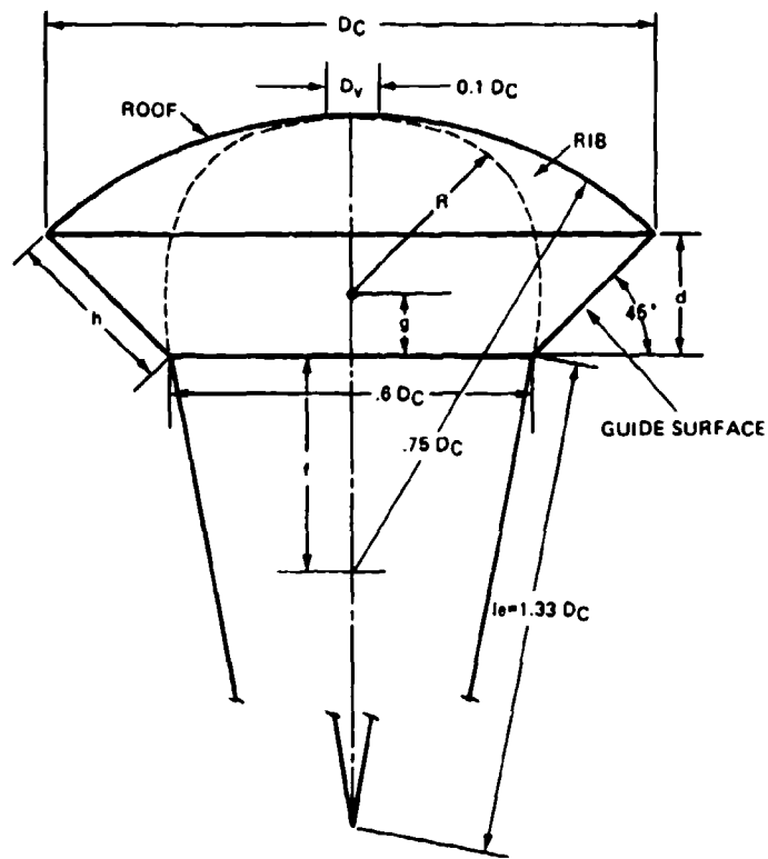
PARACHUTE LAYOUT
