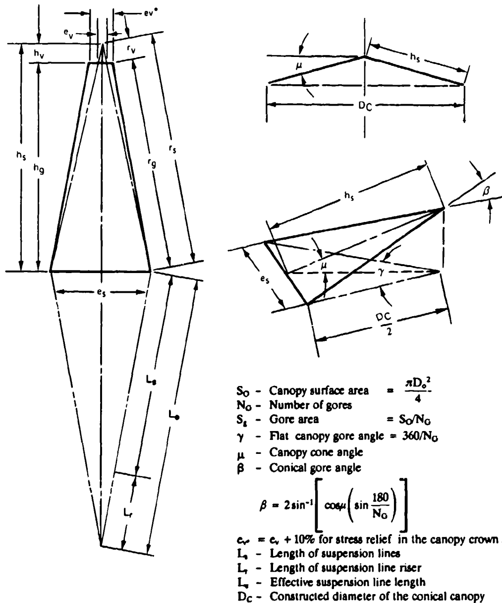
FIGURE 6-15. Circular Flat and Circular Conical Canopy Designs.
