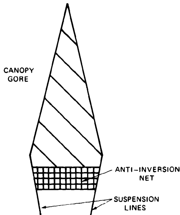
FIGURE 6-33. Canopy Gore with Anti-Inversion Net (Only One Gore Shown).
