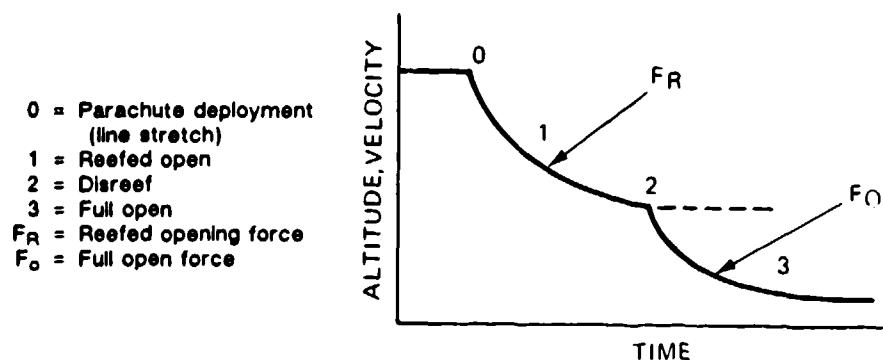
FIGURE 7-8. Velocity-Time Profile.
