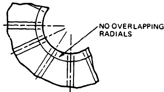
FIGURE 7-14. Vent Construction.
