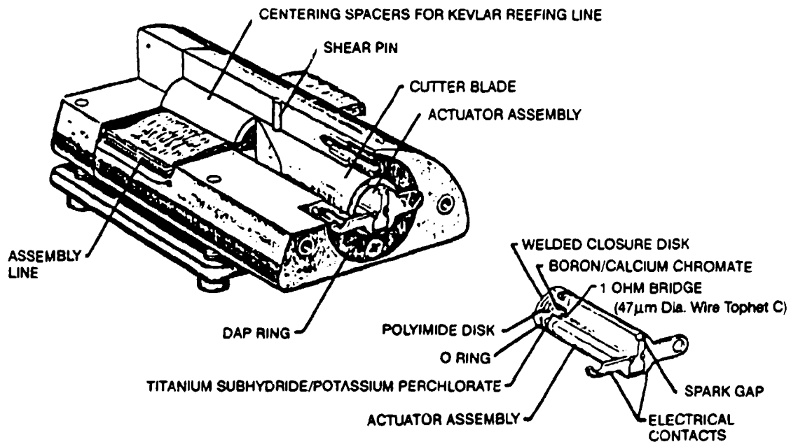
FIGURE 6-50. Sandia MC 3133 Reefing-Line-Cutter Installation.
