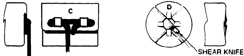
(1) TWO FLAPS WITH LINE STOWS (2) 4 FLAPS WITH TIE CORD AND SHEAR KNIFE (b) Typical Bag Closure.
