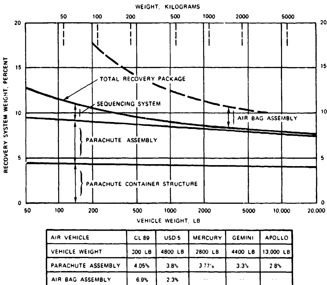
FIGURE 6-61. Parachute Recovery System Weight as Percentage of Air Vehicle Weight.
