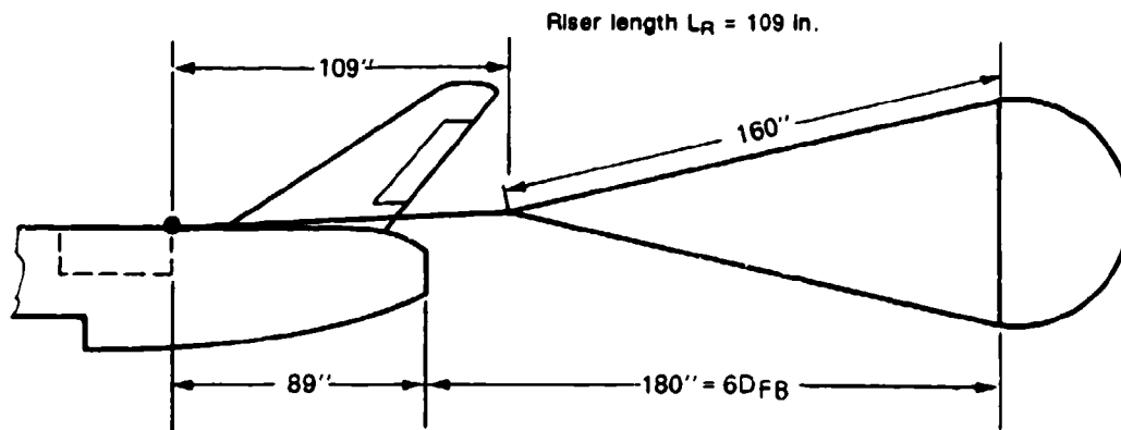
FIGURE 7-5. Extraction-Parachute Assembly.
