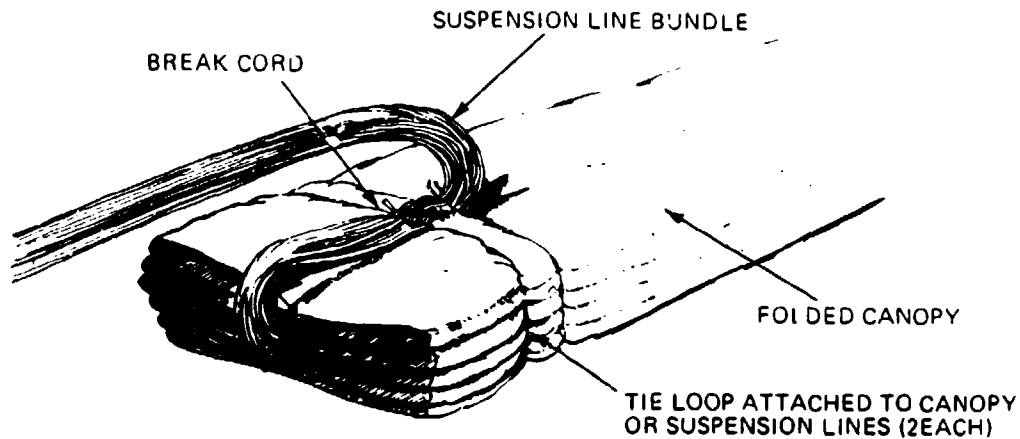
FIGURE 6-39. Skirt Hesitator.
