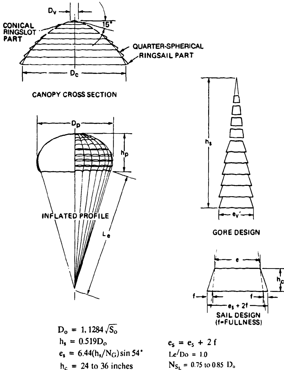
FIGURE 6-28. Typical Design of Ringsail Parachute.
