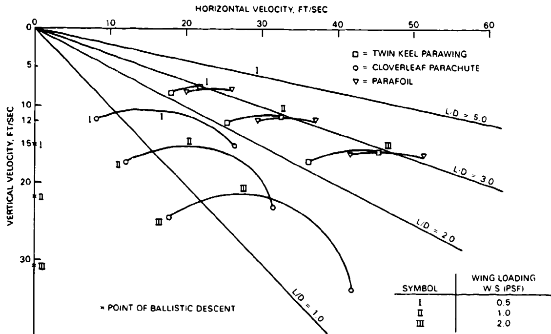
FIGURE 5-107. Flight Performance of Maneuverable Parachute-Vehicle Systems.
