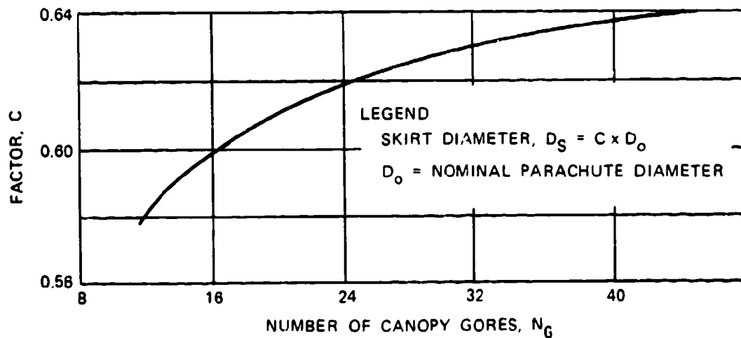
FIGURE 5-78. Canopy-Skirt Diameter as a Function of the Number of Gores for a Ribbon Parachute With D_p = 0.67 D_o .
