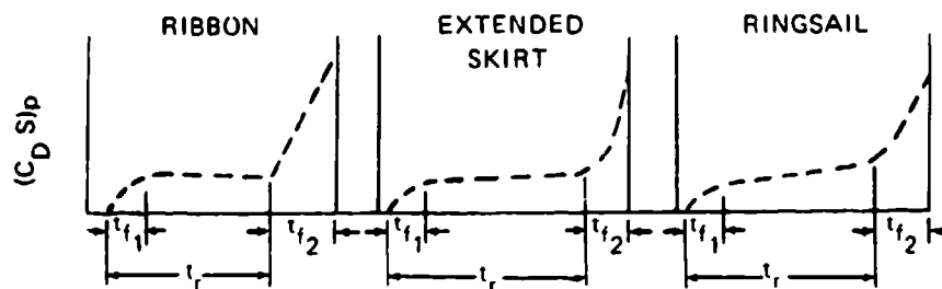
FIGURE 5-39. Typical Drag-Area-Versus-Time Increase for Reefed Parachutes.
