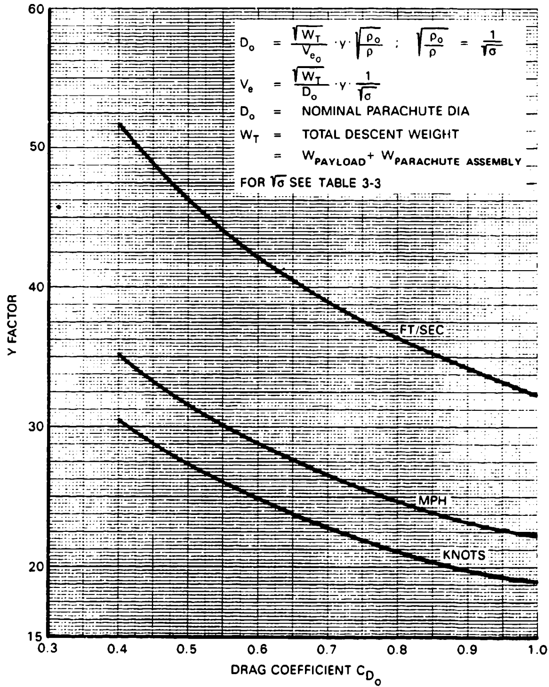
FIGURE 5-112. Y-Factor as Function of Drag Coefficient, C_{D_o} , and Velocity.
