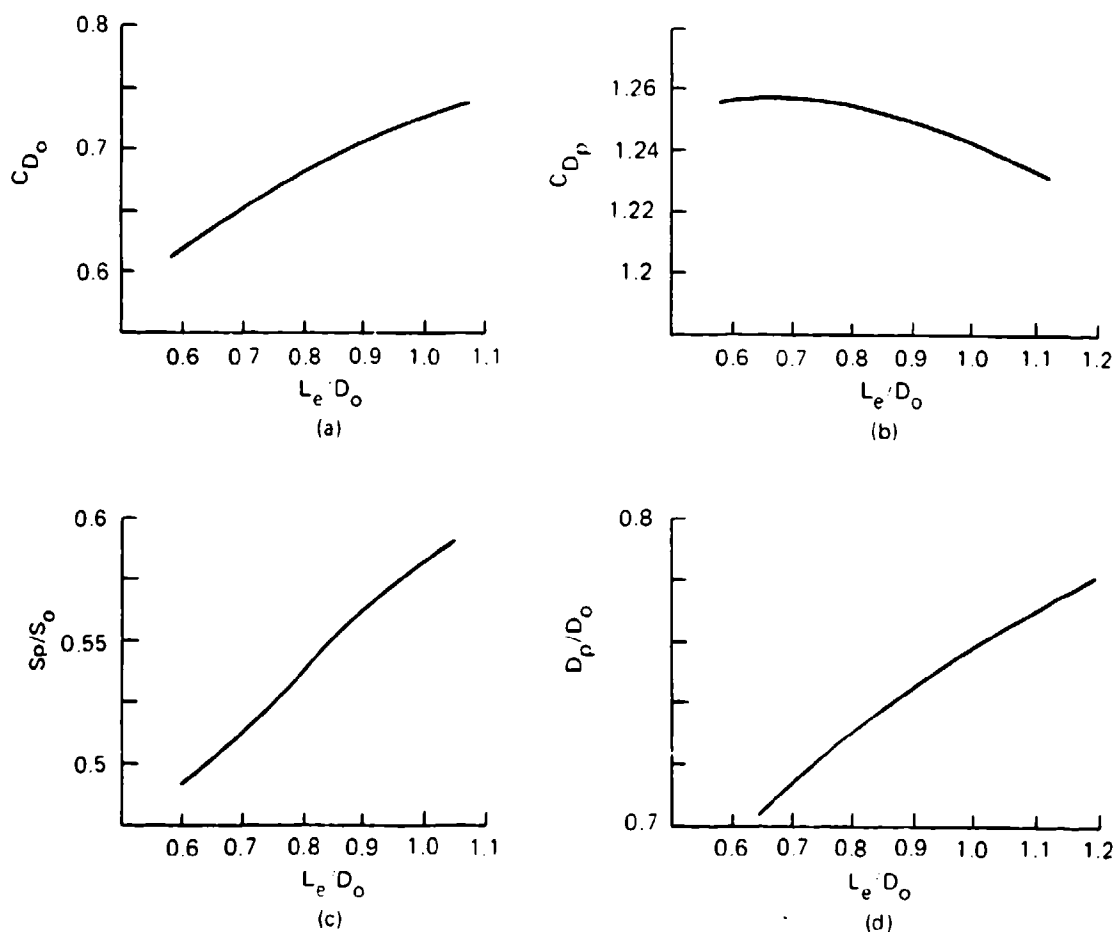
FIGURE 5-19. Drag Coefficients, C_{D_o} and C_{D_p} ; Canopy Area Ratio, S_p/S_o ; and Diameter Ratio, D_p/D_o ; as a Function of Suspension-Line Ratio, L_e/D_o , for a 1-Meter-Diameter Model Parachute.
