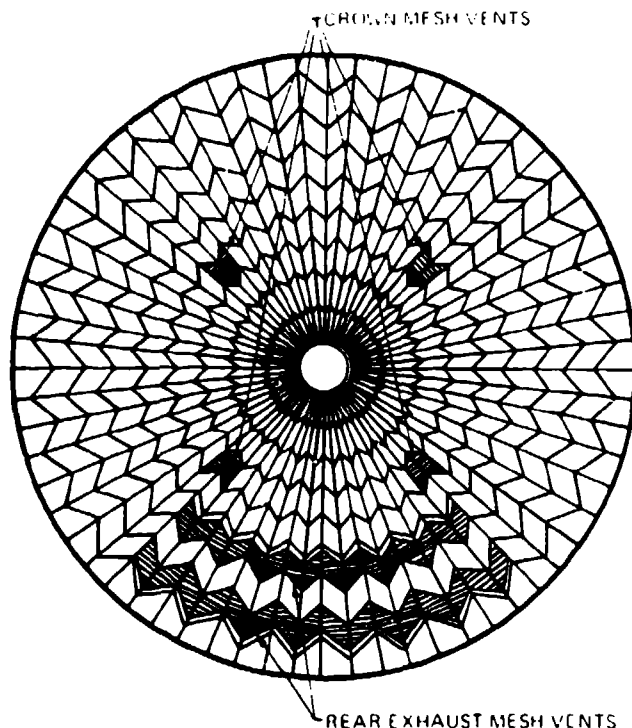
FIGURE 8-9. Main Canopy Plan.
