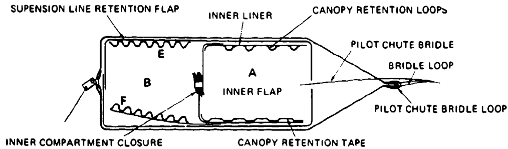
(a) Typical Deployment Bag.
