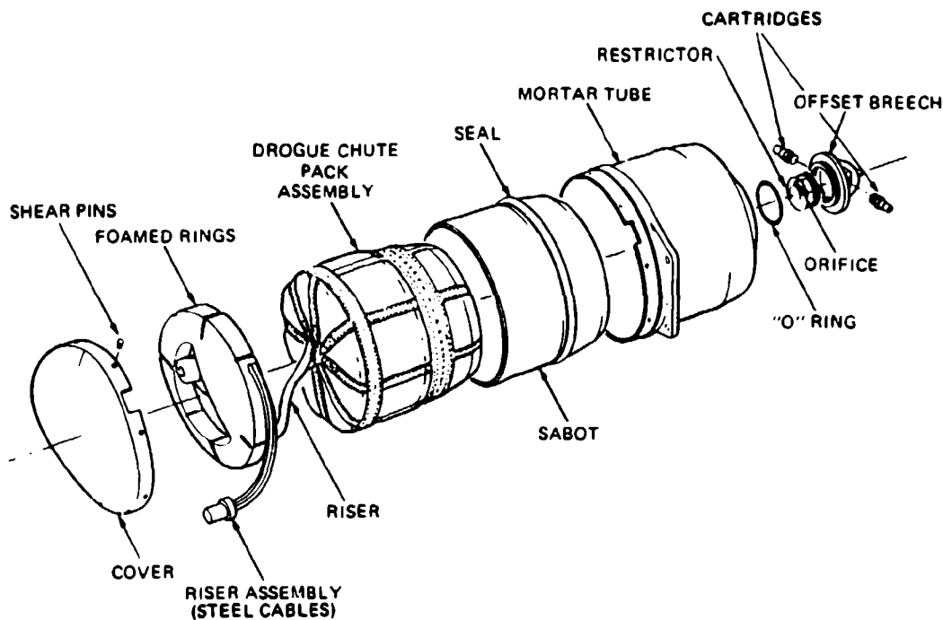
FIGURE 6-8. Mortar Assembly of the Apollo Drogue Chutes.
