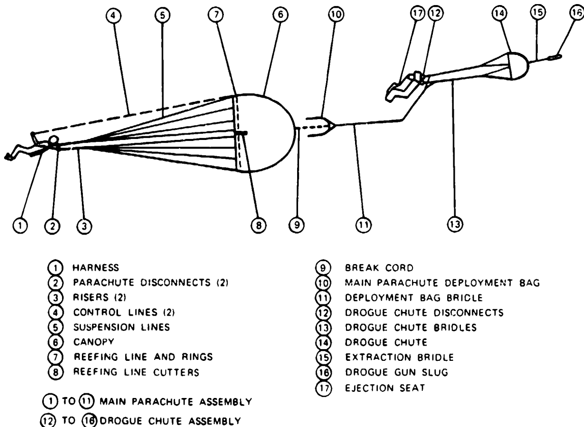
FIGURE 2-2. Schematic and Nomenclature of a Typical Ejection Seat Parachute Assembly.
