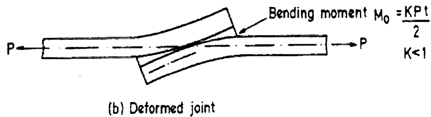
Figure 3.3 A geometrical representation of the Goland and Reissner (1944) bending moment factor ( t = adherent thickness).
