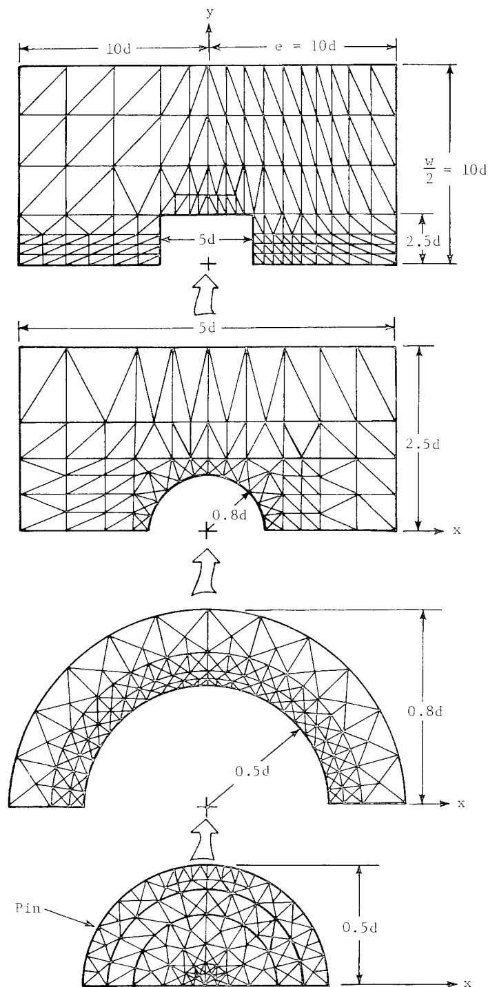
Figure 2.- Finite-element model.
