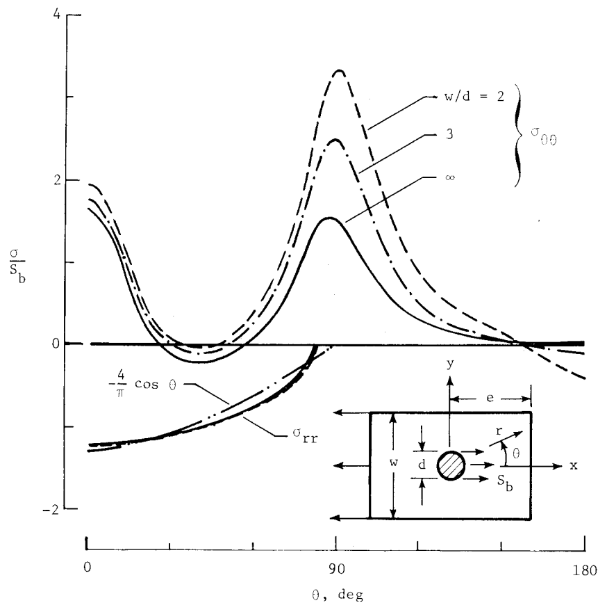
(a) Stresses along hole boundary ( r = R ).
