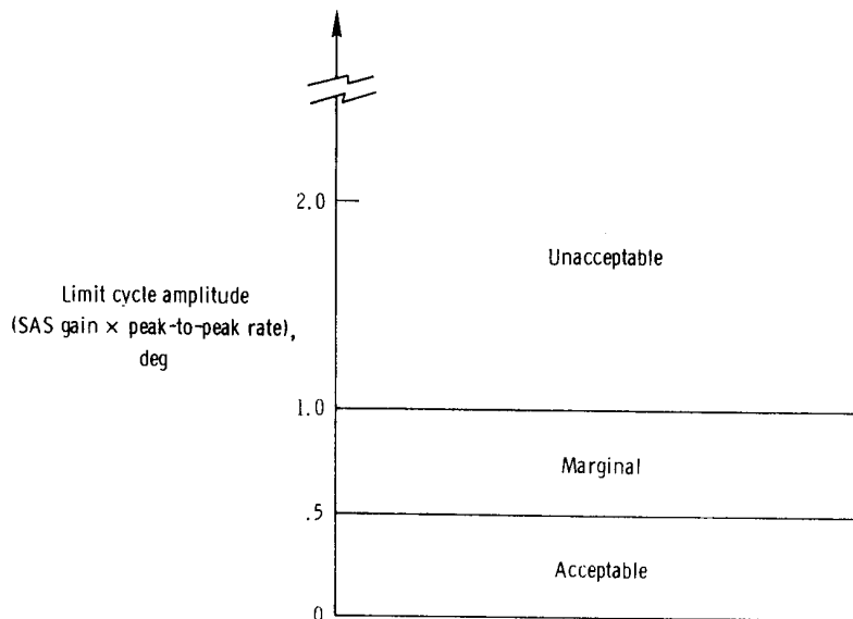
Figure 19. Summary rating scale of limit cycle characteristics, based on pilot evaluations and flight data from several research vehicles.
