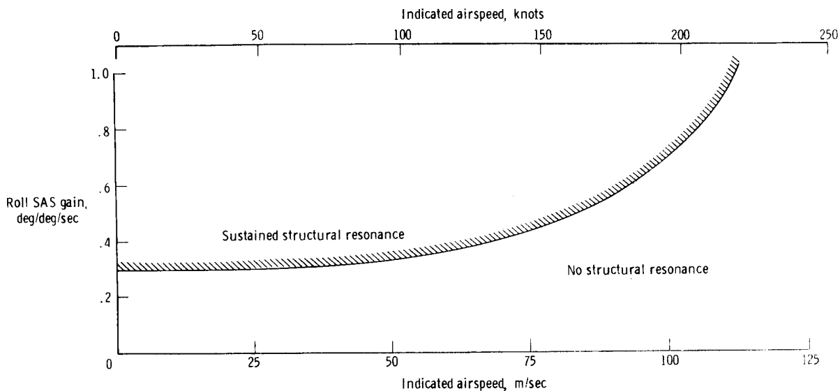
Figure 18. Typical results from structural resonance tests performed with the HL-10 lifting body mated to the launch airplane.
