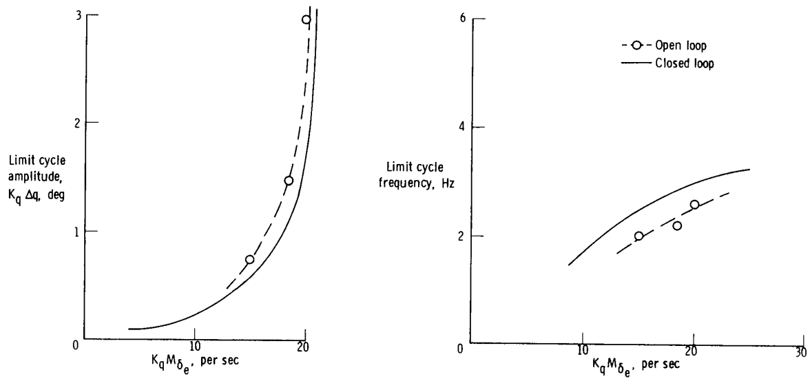
Figure 10. Comparison of limit cycle characteristics determined by the Bode plot and analog computer methods for the M2-F2 lifting body.
