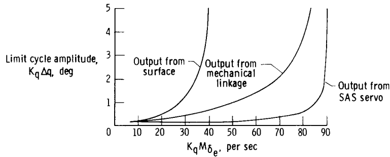
Figure 7. Typical limit cycle ground test characteristics of the pitch SAS of the HL-10 lifting body at various points within the system.
