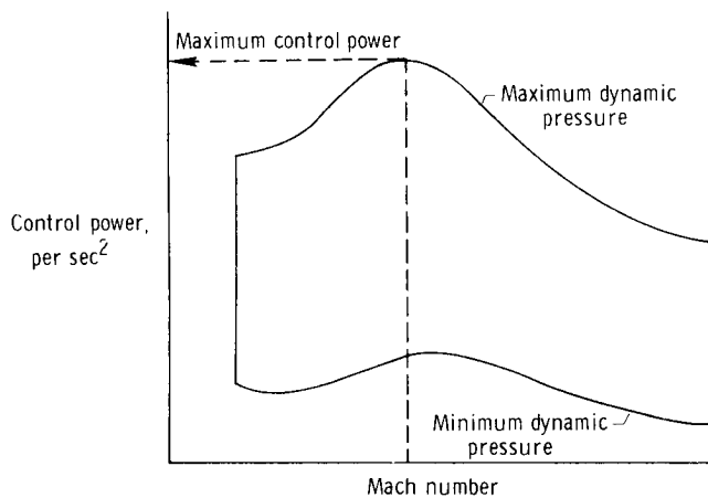
Figure 3. Typical vehicle flight envelope for analysis of limit cycle characteristics.
