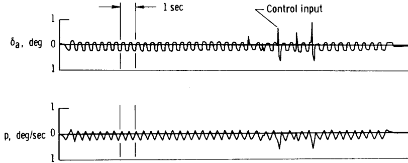
(a) Stable limit cycle; K_p L_{\delta_a} = 10 per sec.
