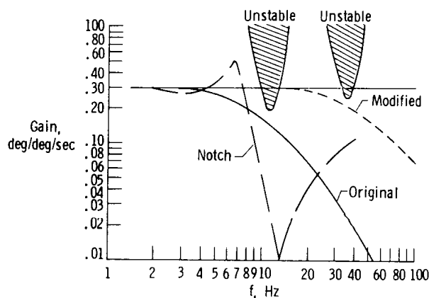
Figure 17. Effect of filters on high-frequency stability of the X-15 airplane (ref. 1).
