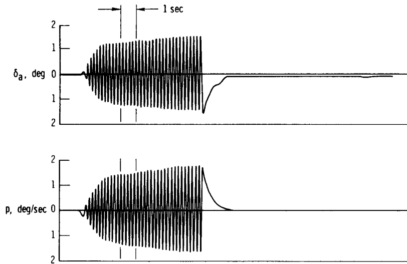
(b) Unstable limit cycle; K_p L_{\delta_a} = 37.5 per sec.
