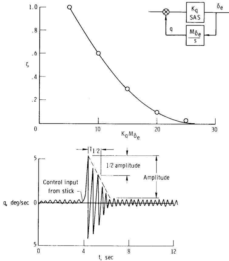
Figure 8. Damping of limit cycle characteristics of the pitch SAS of the M2-F2 lifting body.
