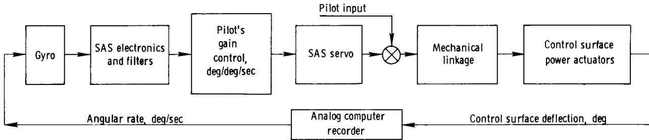
Figure 4. Limit cycle test setup.
