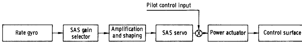
Figure 1. Functional diagram of typical SAS used in analysis.
