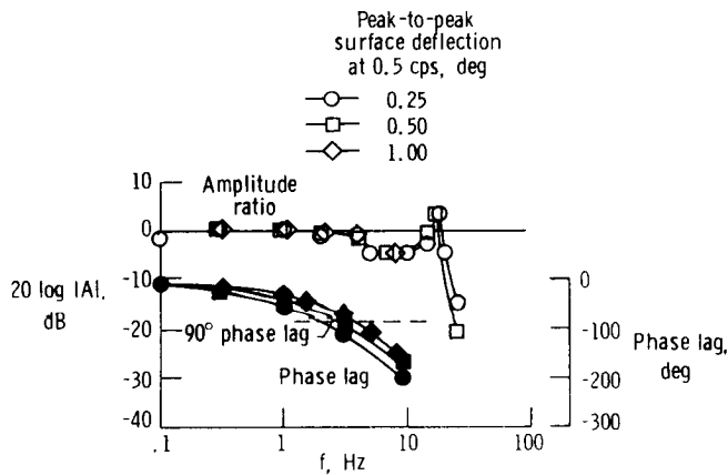
Figure 2. Frequency response of the pitch SAS of the X-24A lifting body. Gyro to control surface.
