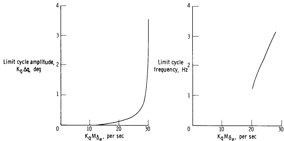
Figure 6. Typical limit cycle ground test characteristics of the pitch SAS of the X-24A lifting body.
