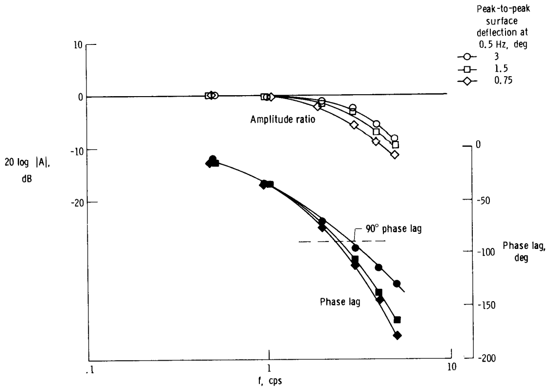
Figure 9. Frequency response of the pitch SAS of the M2-F2 lifting body. Gyro to control surface.
