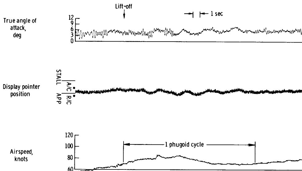
Figure 7. Time history of a short-field takeoff when pilot used angle-of-attack display instrument.
