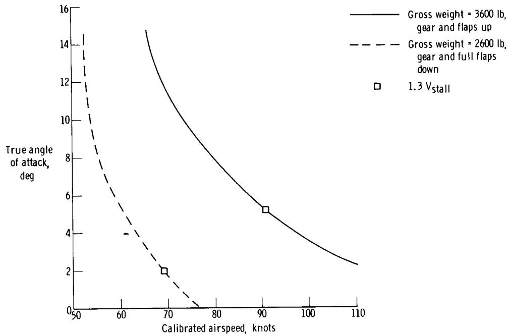
Figure 4. Variation of angle of attack with airspeed for the test airplane with power off, as determined from full-scale wind-tunnel test data.
