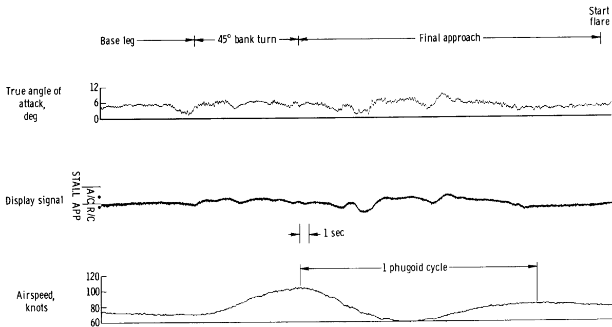
Figure 9. Time history of landing approach when pilot used angle-of-attack display instrument.
