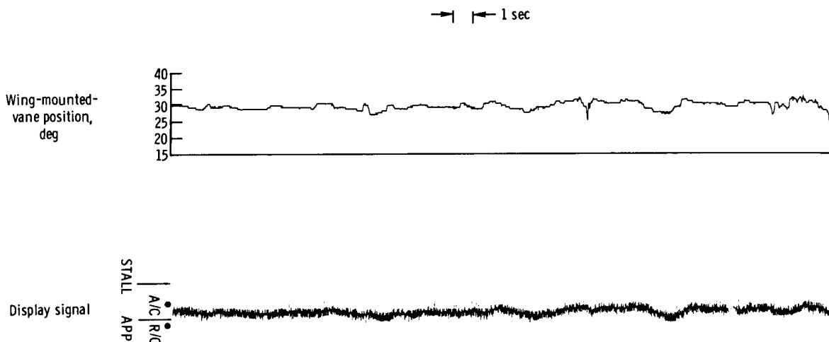
Figure 6. Time history of position and display signal of wing-mounted vane during a landing approach.
