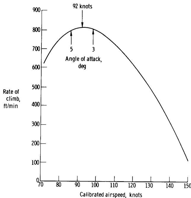
Figure 8. Rate-of-climb performance as a function of airspeed of the test airplane. Gross weight, 3450 pounds; gear and flaps up; 6000 feet altitude; 64° F.
