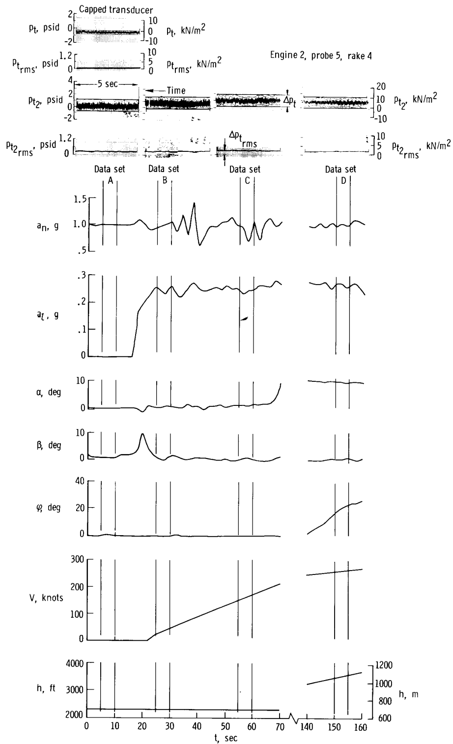
Figure 10.— Data samples and time histories of selected flight parameters during XB-70-1 takeoff data-set intervals.
