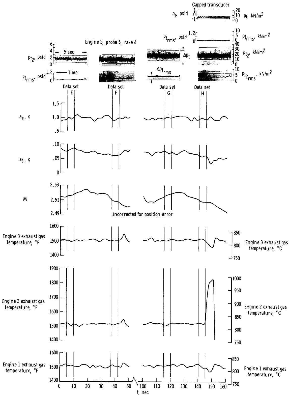
Figure 11.— Data samples and time histories of selected flight parameters during XB-70-1 Mach = 2.5 turbulence test data-set intervals.
