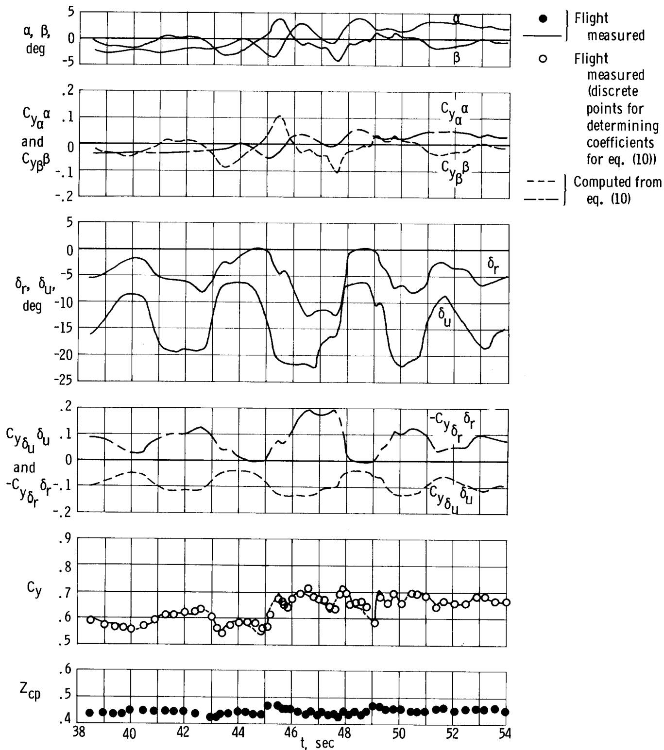
Figure 6. — Time history of flight M-16 maneuver. q = 260 to 296 lb/ft 2 ( 12,449 to 14,172 N/m 2 ); M = 0.46 to 0.49 .
