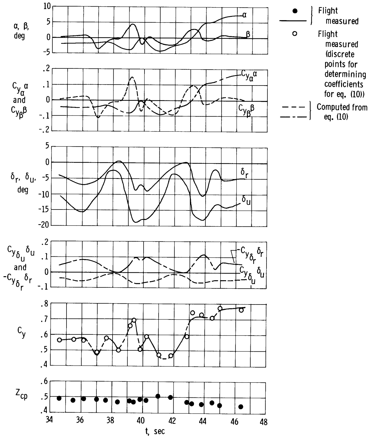
Figure 5. — Time history of flight M-10 maneuver. q = 225 to 260 \text{ lb/ft}^2 ( 10,773 to 12,449 \text{ N/m}^2 ); M = 0.59 to 0.62 .
