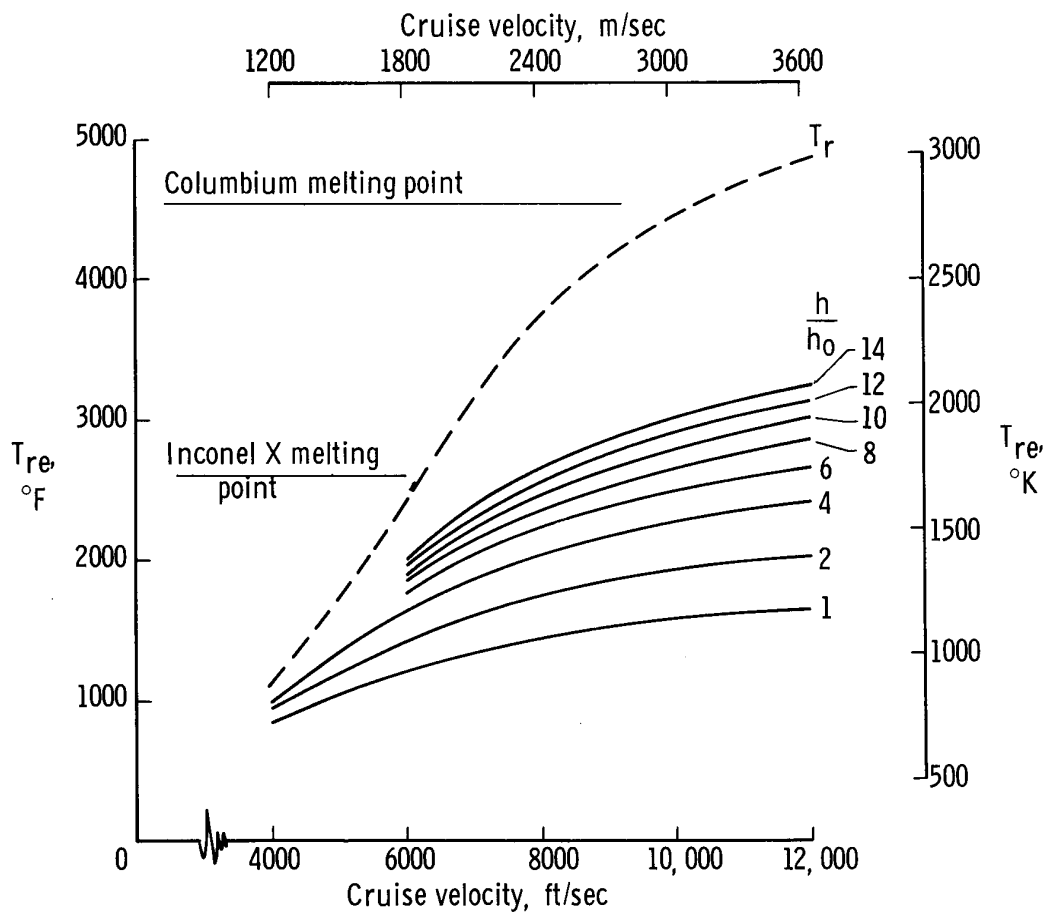
Figure 15. — Effect of increasing turbulent heat-transfer coefficient on radiation-equilibrium temperature for a flat plate at zero angle of attack. q_{\infty} = 1000 \text{ lb/ft}^2 ( 47,880 \text{ N/m}^2 ); x = 10 \text{ ft} ( 3.05 \text{ m} ); \epsilon = 0.85 .
