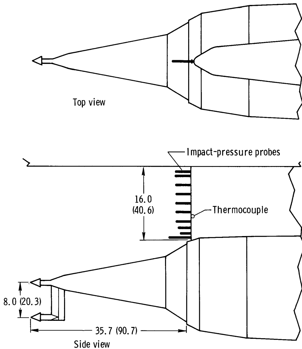
Figure 4.— Dummy ramjet engine and pylon with pertinent instrumentation. Dimensions in inches (centimeters).
