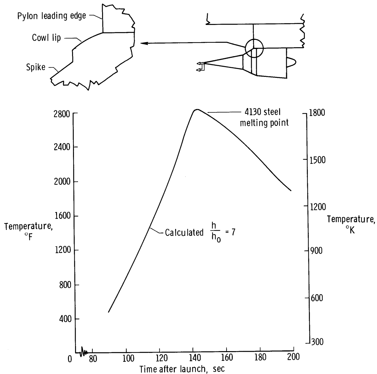
Figure 13. - Calculated temperature time history of cowl-lip interference zone.
