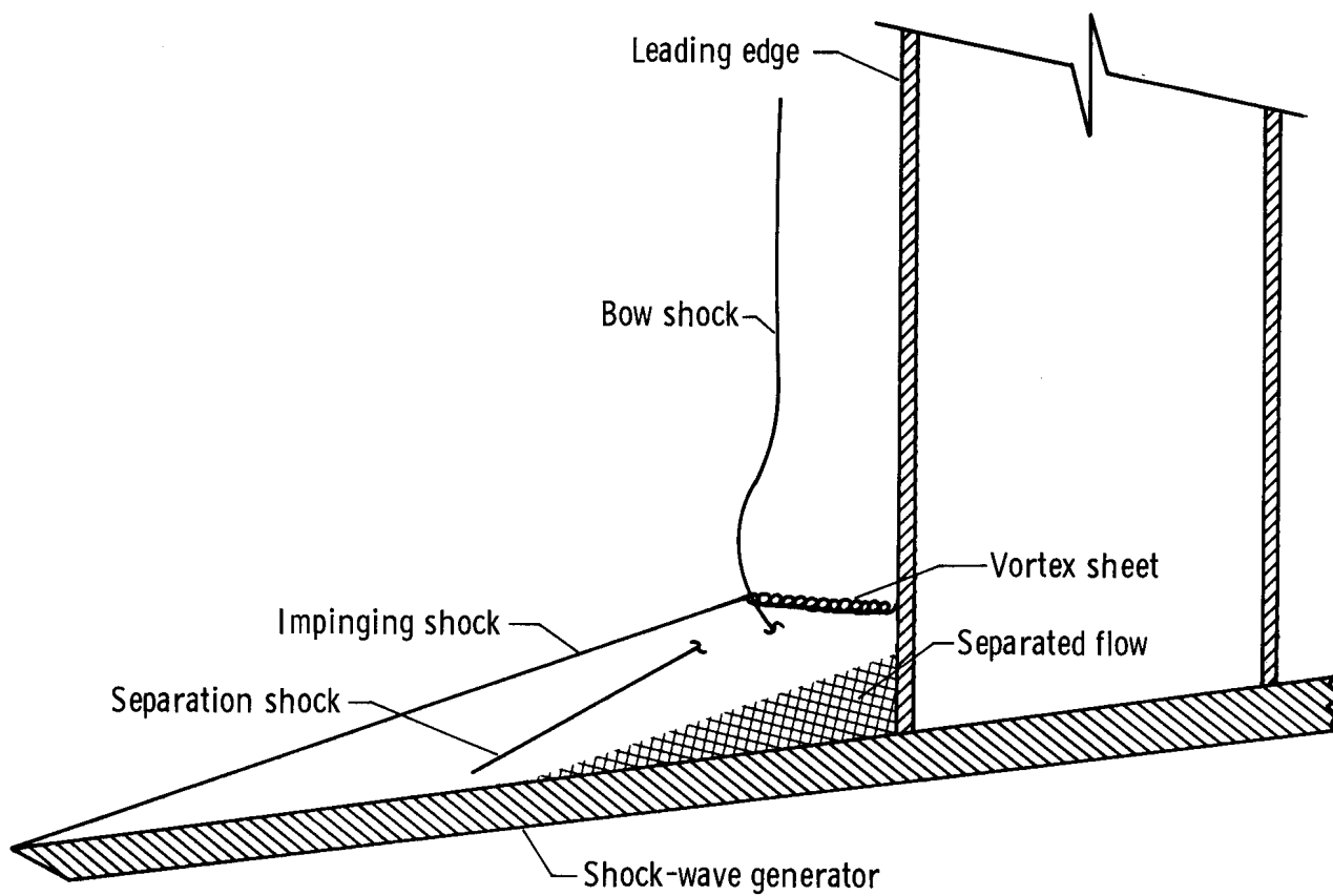
Figure 8. — Flow field associated with leading-edge shock impingement (adapted from ref. 4, appendix A).
