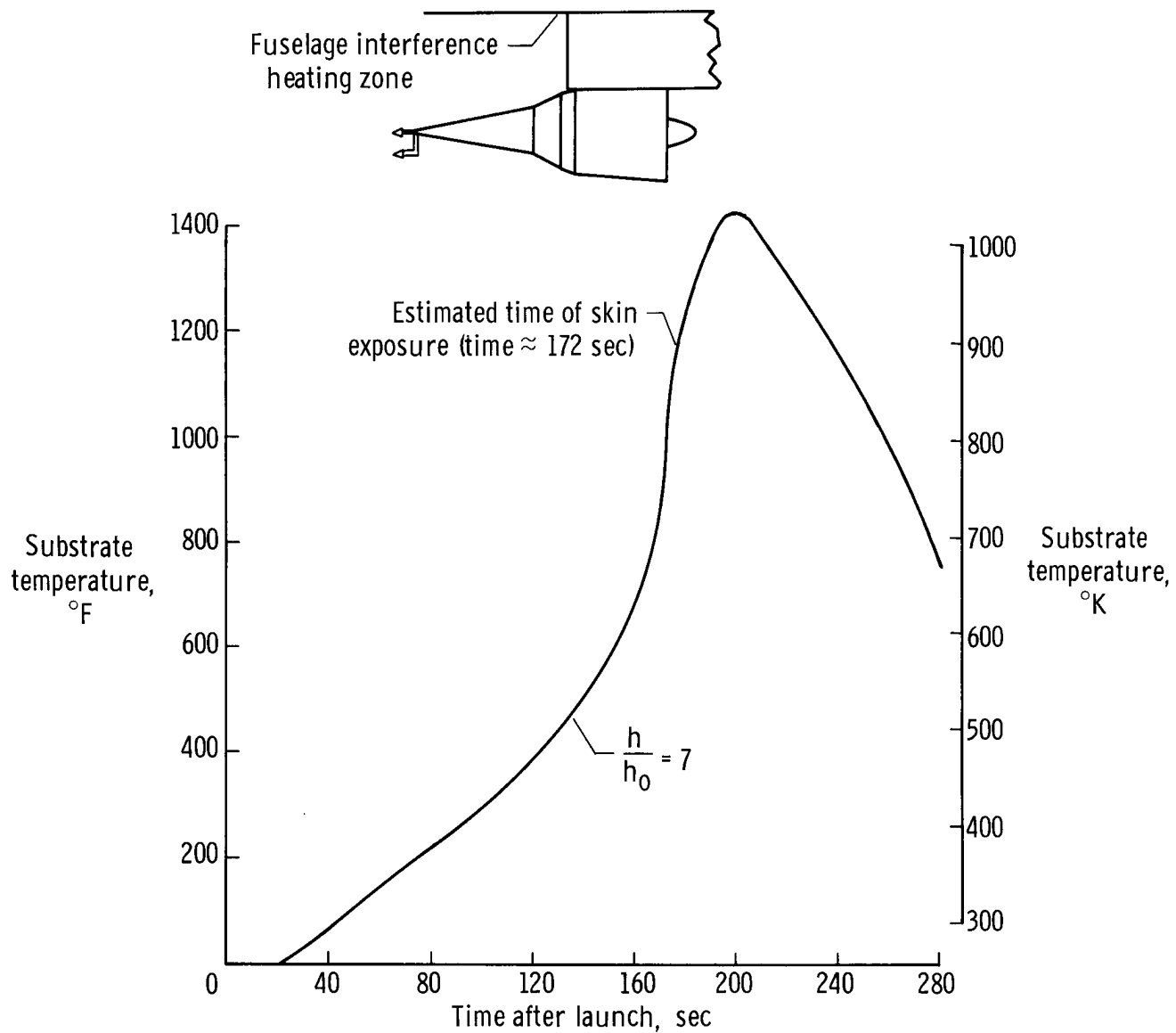
Figure 12. — Calculated substrate temperature time history of fuselage interference heating zone.
