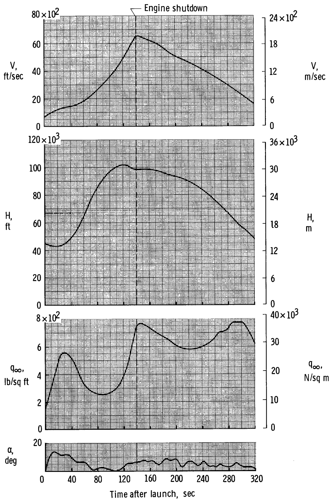
Figure 5. — History of pertinent flight parameters.
