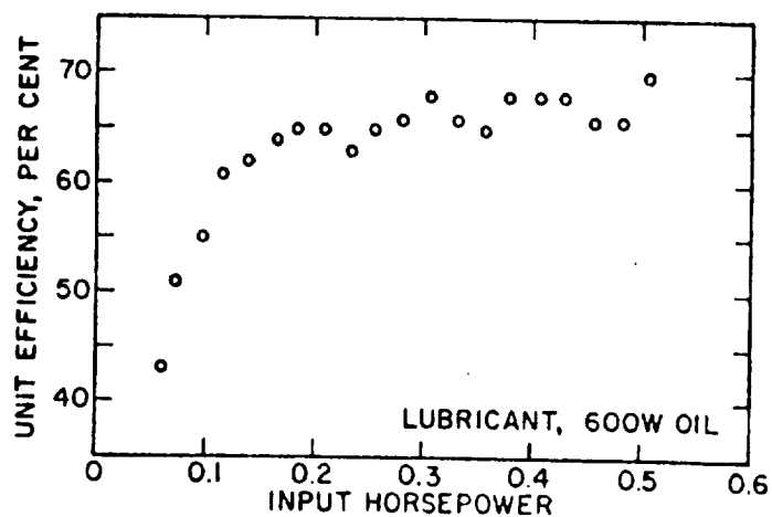
Figure 2. Oil Lubrication Efficiency Versus Input Horsepower
