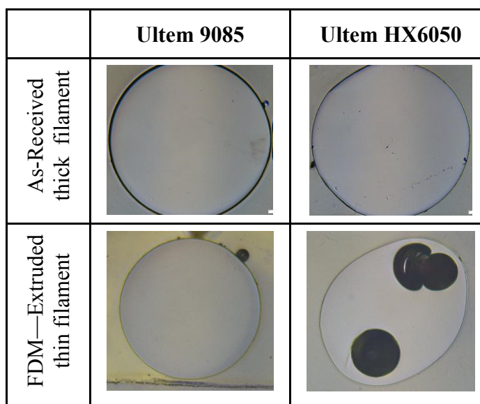
Figure 14.—Optical micrographs of Ultem 9085 and XH6050 resin filaments.
