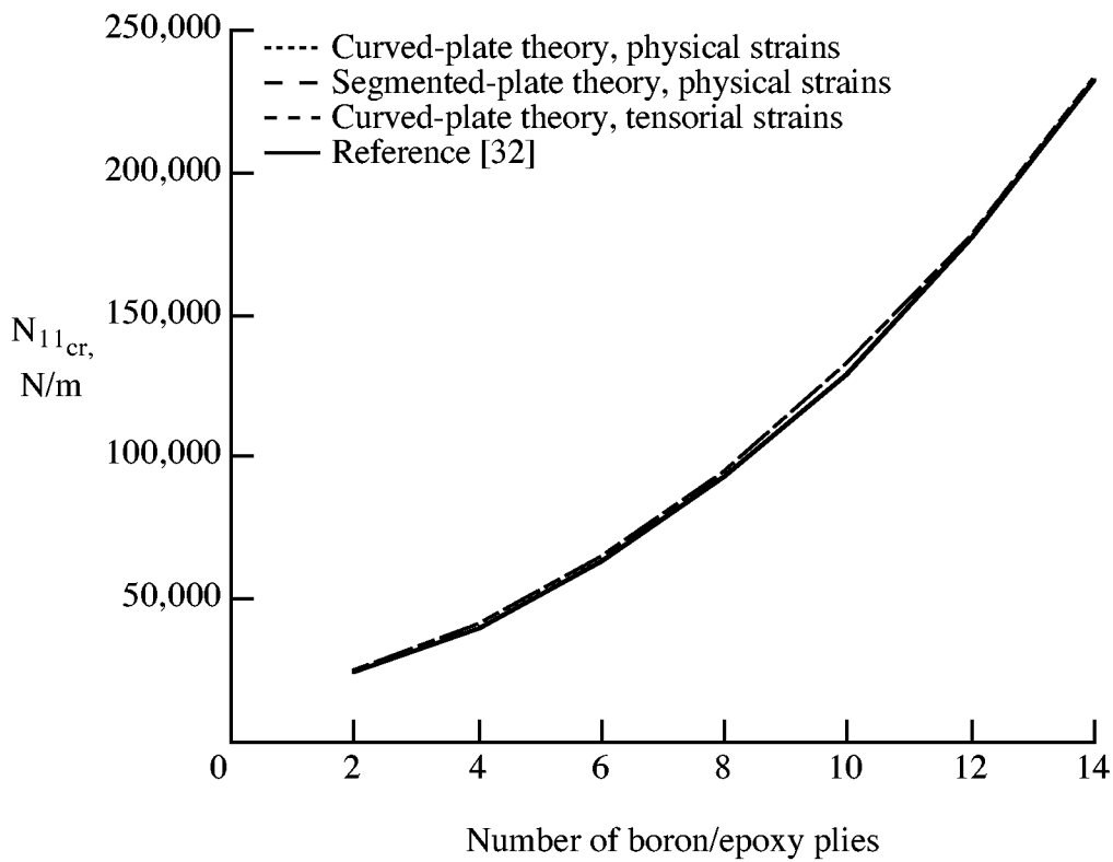
Figure 4.11 Critical value of stress resultant N_{11} for buckling of an unsymmetrically laminated aluminum and boron/epoxy (B/E) curved plate with simply supported longitudinal edges.
