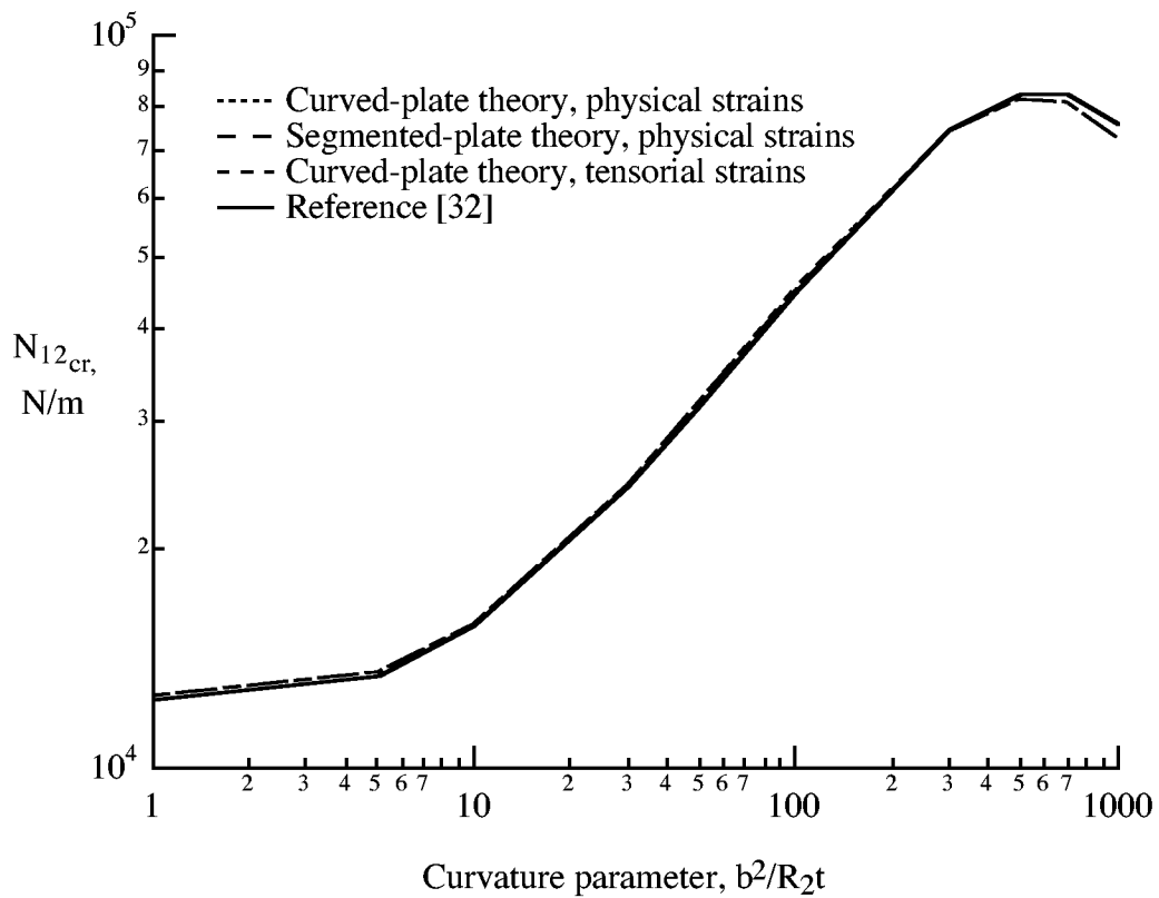
Figure 4.8 Critical value of stress resultant N_{12} for buckling of a symmetrically laminated curved plate with clamped longitudinal edges.
