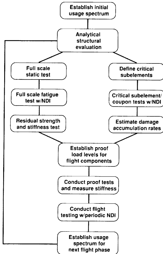
Figure 10. Application of the wear out methodology.
