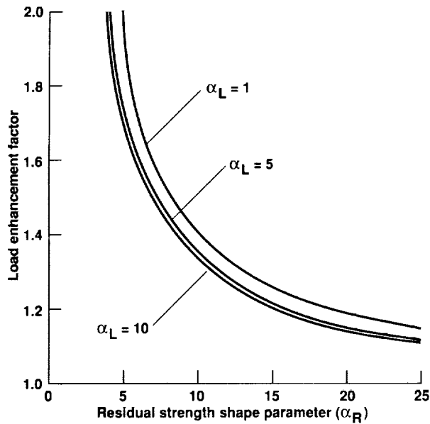
Figure 7. Load enhancement factor (required to demonstrate B-basis reliability at the end of one life) versus the residual strength shape parameter ( \alpha_R ) using a single fatigue test to one lifetime.
