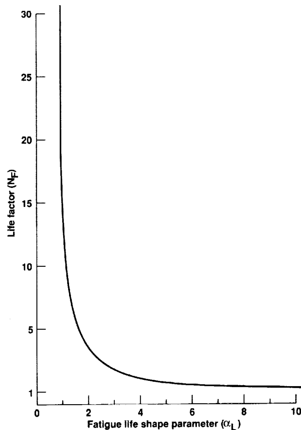
Figure 6. Life factor ( N_F ) required to demonstrate B-basis reliability at the end of one life versus fatigue life shape parameter ( \alpha_L ) using a single full scale fatigue test article.
