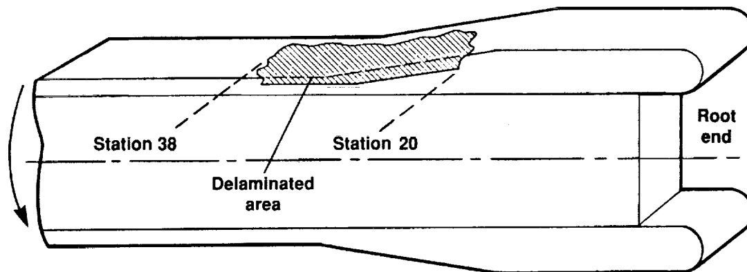
Figure 4. Delaminated region of failed flexbeam.
