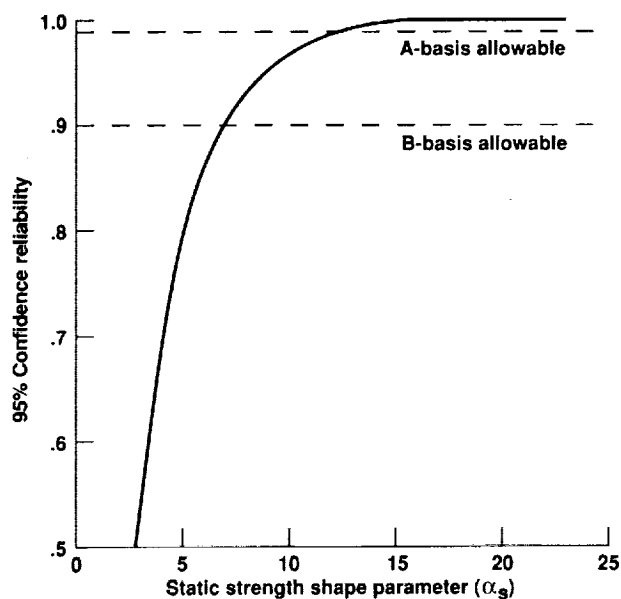
Figure 5. The 95% confidence reliability versus the static strength shape parameter ( \alpha_s ) for a single full scale static test to 150% of design limit load.
