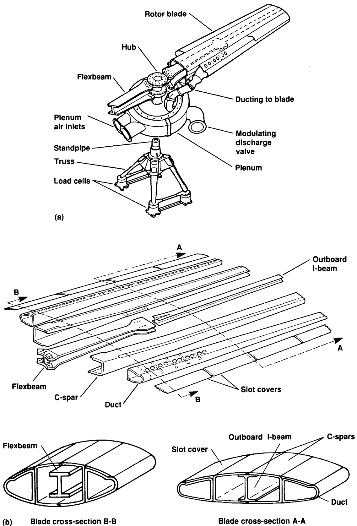
Figure 3. X-Wing rotor system. (a) Rotor system schematic; (b) major rotor blade components and cross-sections.
