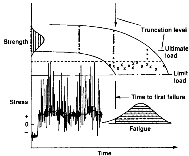
Figure 9. Wear out model showing the relation of static failure, load history, and fatigue failure (ref. 11).
