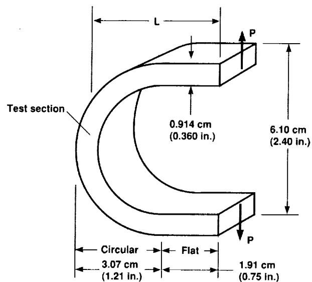
Figure 11. Curved beam interlaminar tension test coupon.
