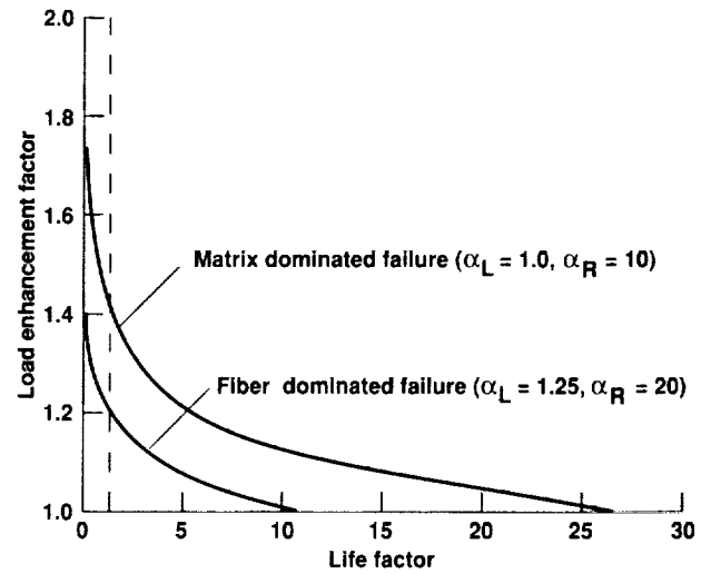
Figure 8. Possible combinations of load enhancement factor and life factor ( N_F ) (necessary to demonstrate B-basis reliability at the end of one lifetime) using a single full scale test article.
