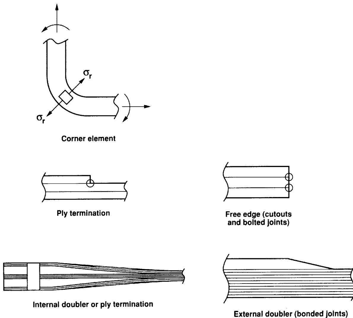
Figure 1. Sources of delamination stresses.
