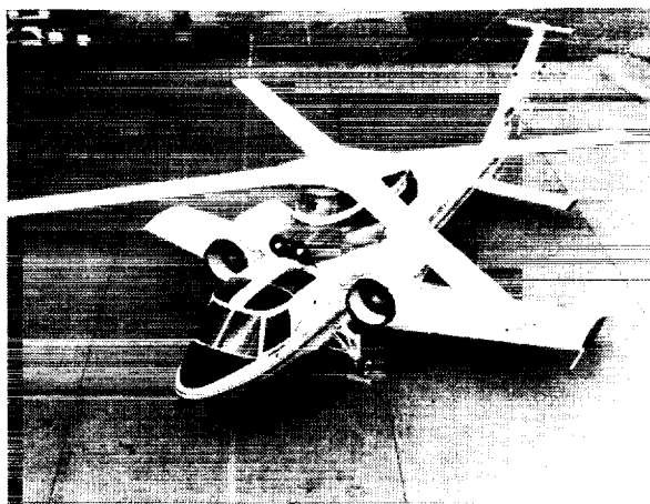
Figure 2. RSRA/X-Wing flight vehicle.
