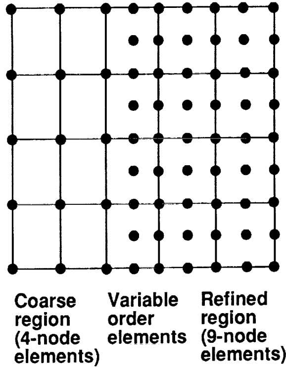
Fig. 1.3 Mesh transitioning using variable-order elements.
