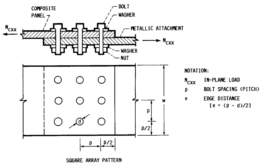
SQUARE ARRAY PATTERN FIGURE 2. - SCHEMATIC OF MULTI-BOLT COMPOSITE JOINT.
