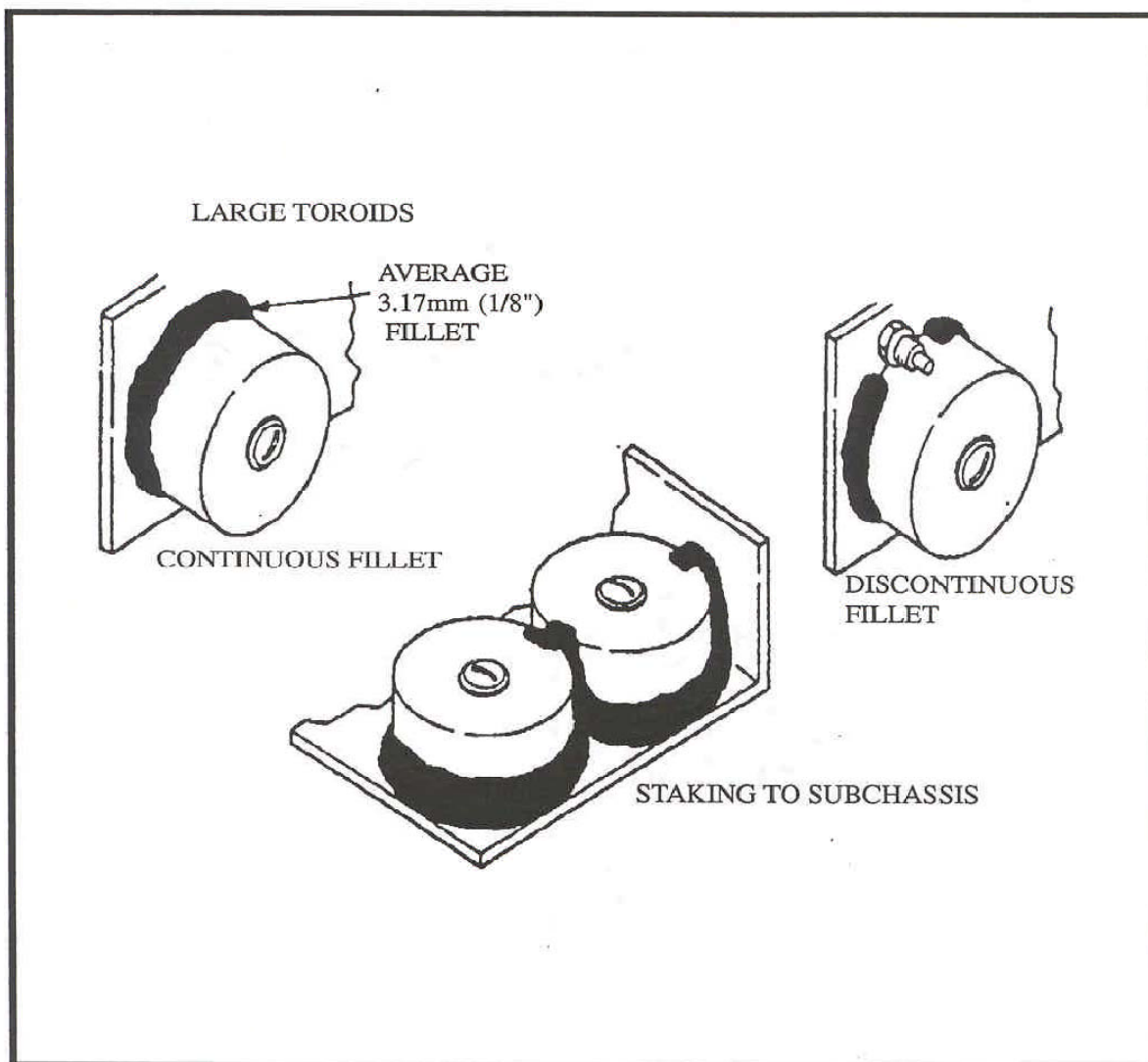
Figure 9-9: Toroid Staking
