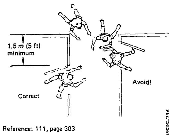
Figure 8.10.2-1. Place Door Openings Away From Traffic Congestion
