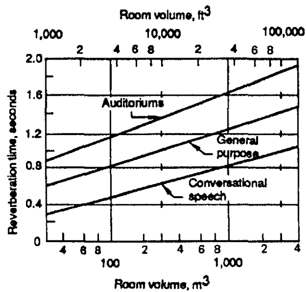
Figure 5.4.3.2.2.1-2. Preferred Reverberation Time
