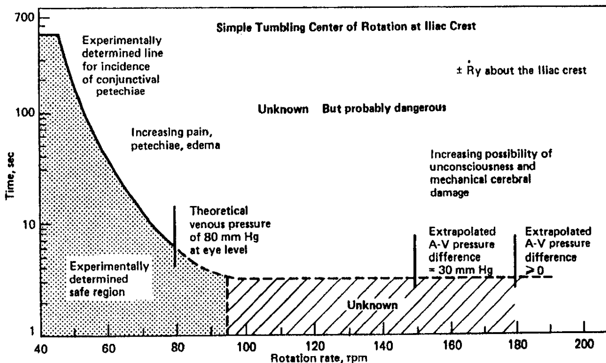
Figure 5.3.3.2. Rotational Acceleration Limits for Rotation About the Pitch Axis With No Superimposed Deceleration Field With Center of Rotation at the Iliac Crest
