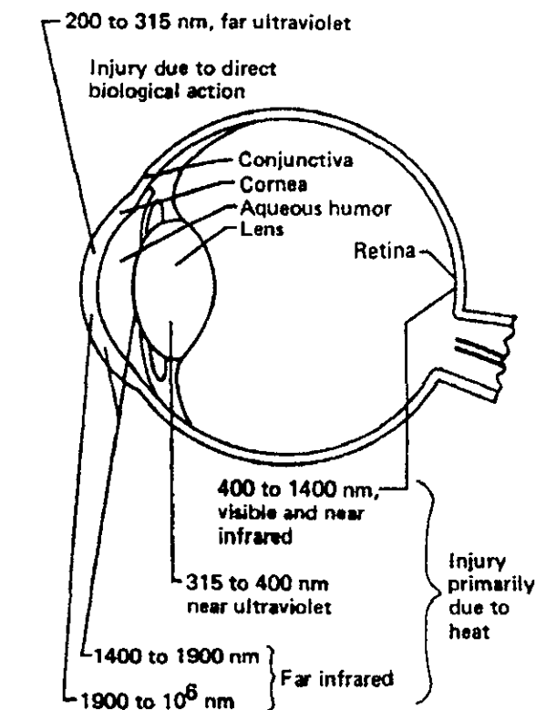
Figure 5.7.3.1.3-3. Impact of Optical Radiation on the Eye
