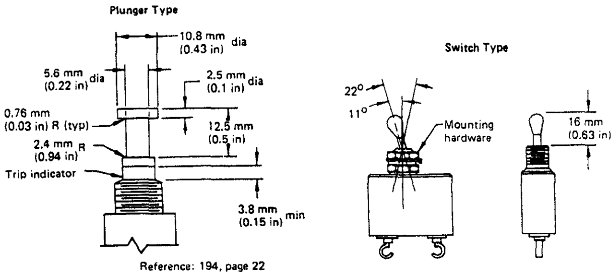
Figure 9.3.3.3.13-1. Circuit Breakers
