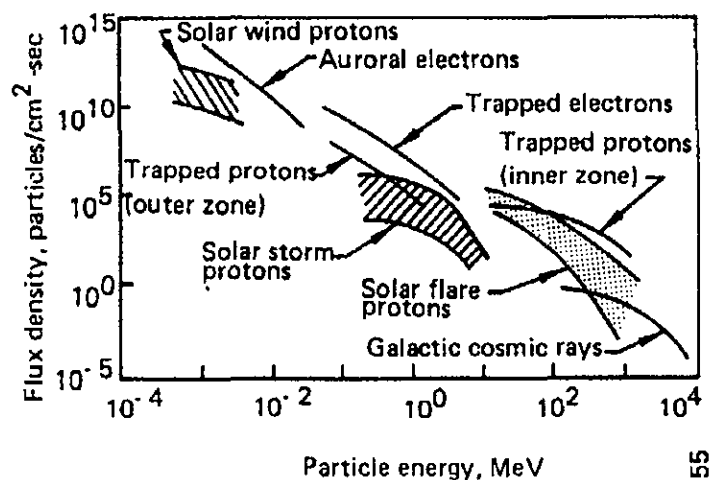
Figure 5.7.2.1.2-1. Space Radiation Environment
