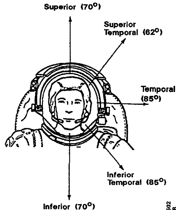
Figure 14.3.2.3.1-2 Crewmember Field of View
