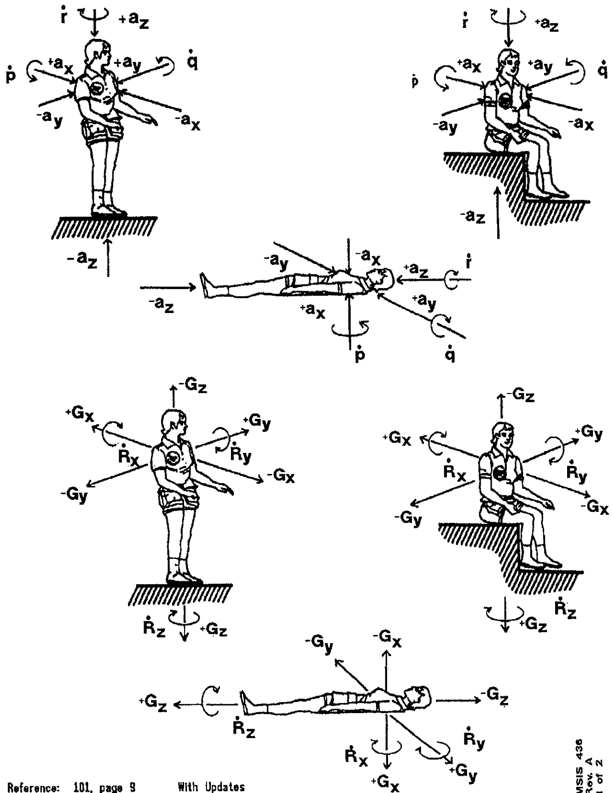
Figure 5.3.1.-1 Acceleration Environment Coordinate System Used in MSIS
