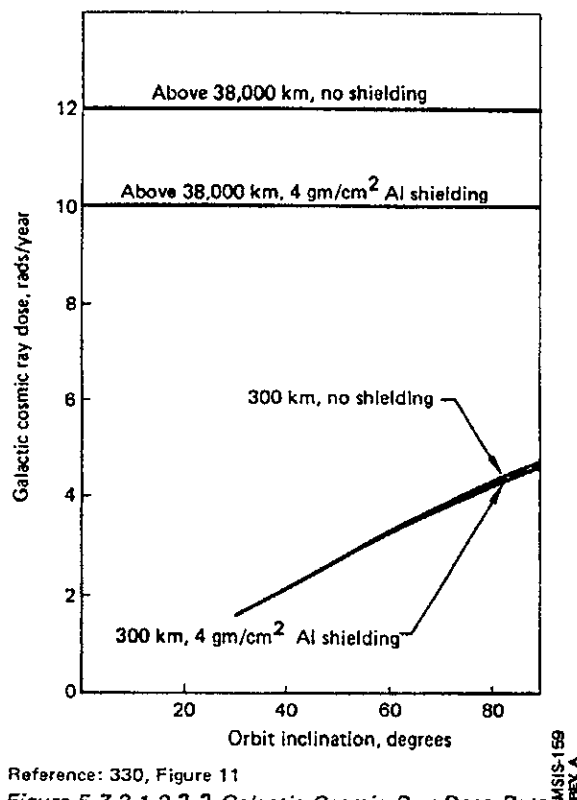
Figure 5.7.2.1.2.2-2 Galactic Cosmic Ray Dose Rate in Rads as a Function of Orbit Altitude and Inclination
