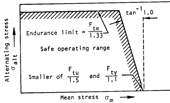
Figure 33. — Safe operating limits on blade mean stress and alternating stress.
