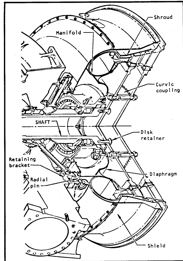
Figure 4. — Mark 10 turbine assembly (F-1 engine).
