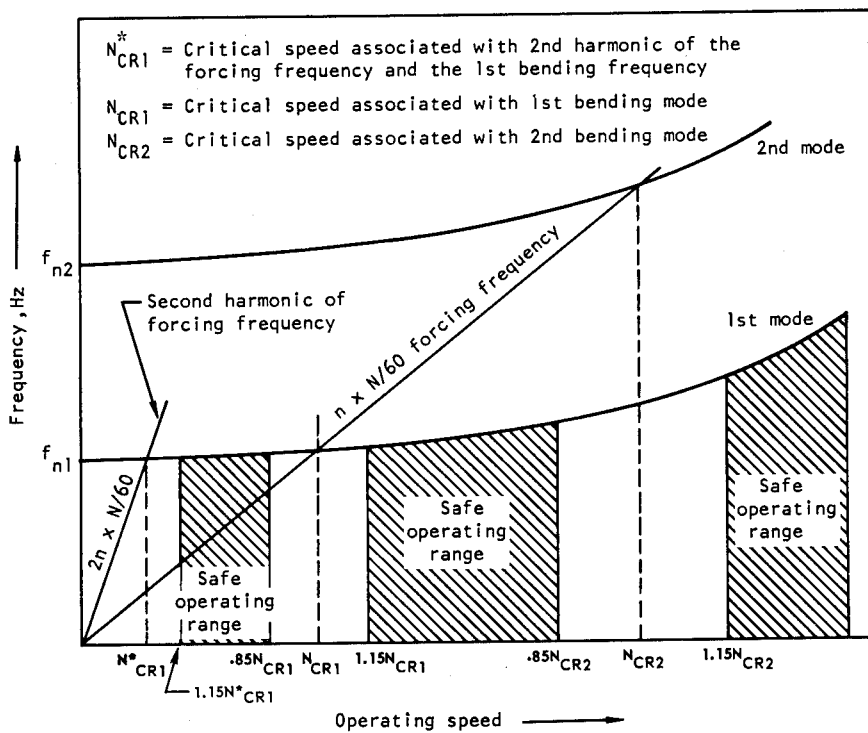
Figure 34. — Safe operating speed range for turbine blades related to critical speeds and forcing frequencies.
