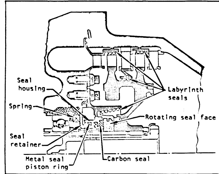
Figure 10. — RL10 A3-3 turbine assembly.
