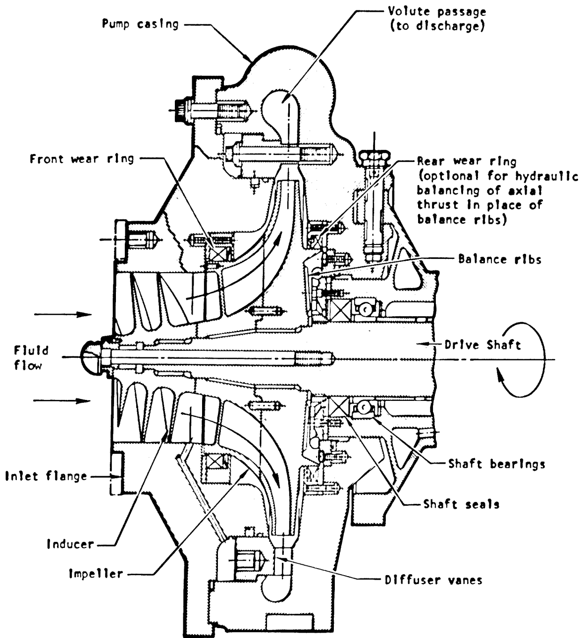
Figure 1. - Elements of a centrifugal flow pump.
