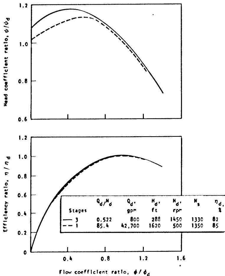
Figure 12. — Performance comparison of internal-crossover pumps differing greatly in size.
