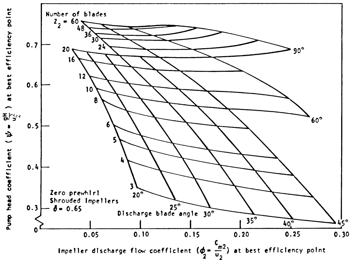
Figure 16. – Impeller blade number and discharge angle related to discharge flow coefficient and head coefficient.
