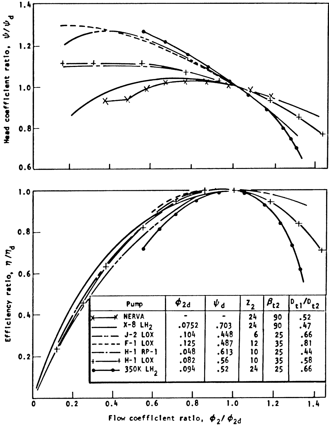
Figure 13. - Pump performance as a function of pump geometry.
