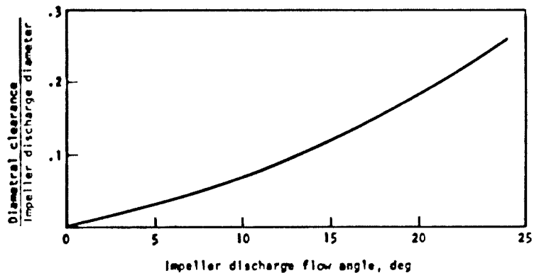
Figure 24. — Impeller-to-stator spacing as a function of discharge flow angle.
