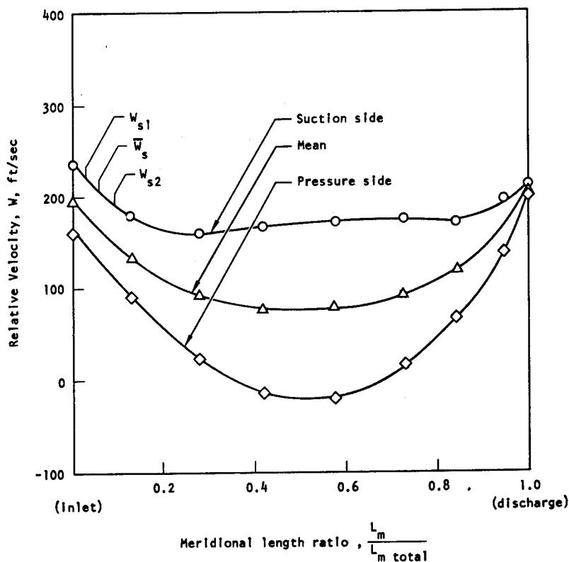
Figure 19. — Calculated relative velocities along streamlines for experimental F-1 LOX impeller with eight full blades.
