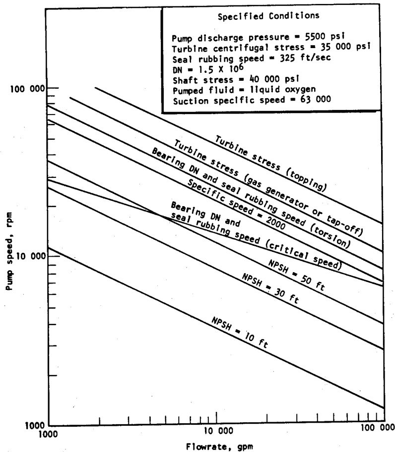
Figure 2. — Various kinds of pump speed limits illustrated for specified conditions.
