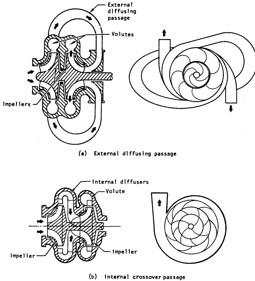
Figure 11. — Basic types of interstage flow passages.
