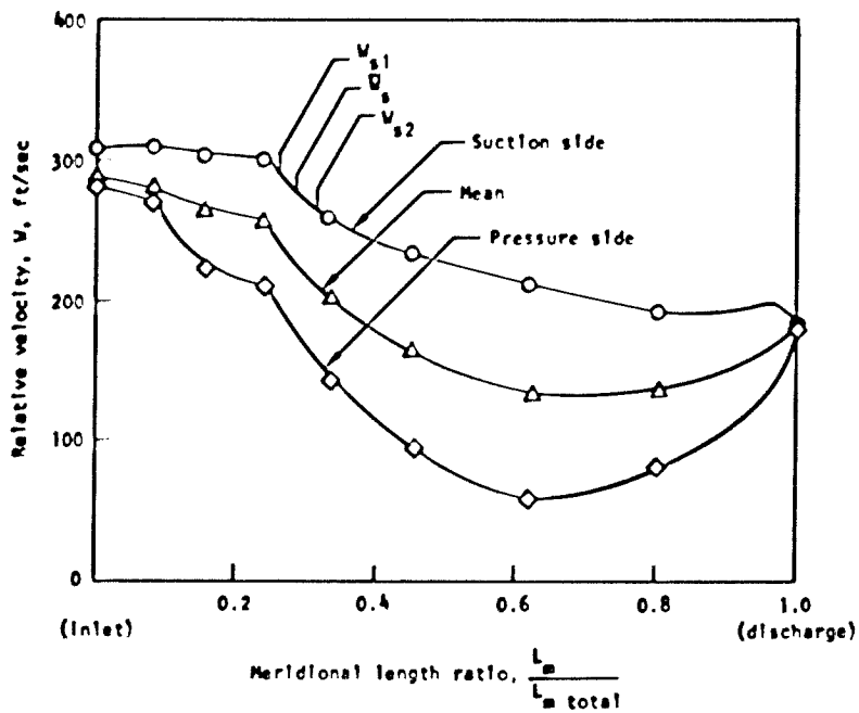
Figure 18. - Calculated relative velocities along streamlines for experimental F-1 fuel impeller with six full blades and six splitters.
