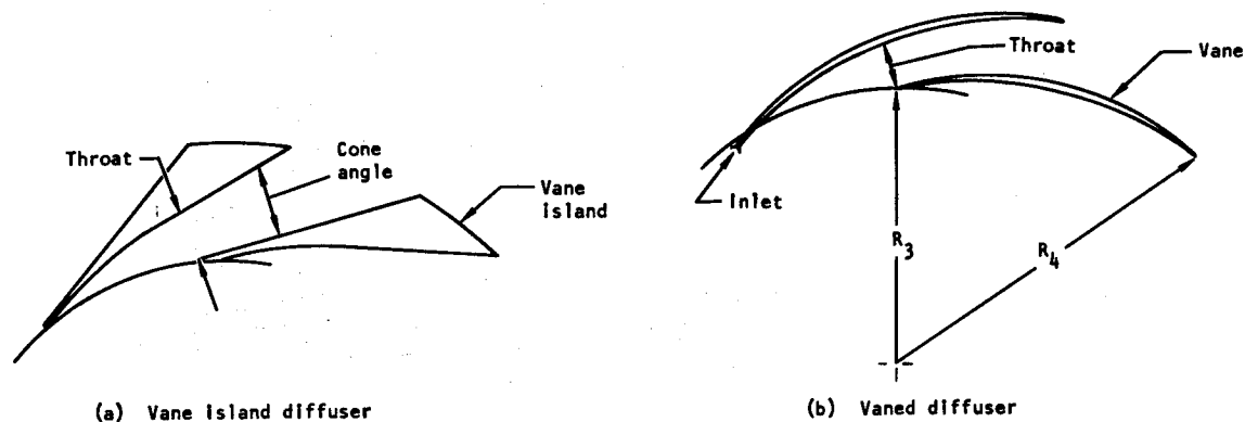
Figure 27. — Vaned diffuser designs.
