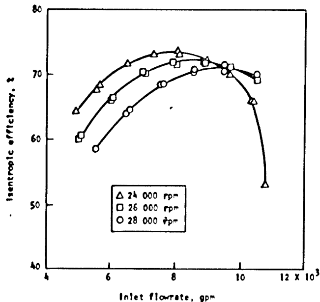
Figure 7. — Influence of speed on hydrogen-pump efficiency (J-2S).
