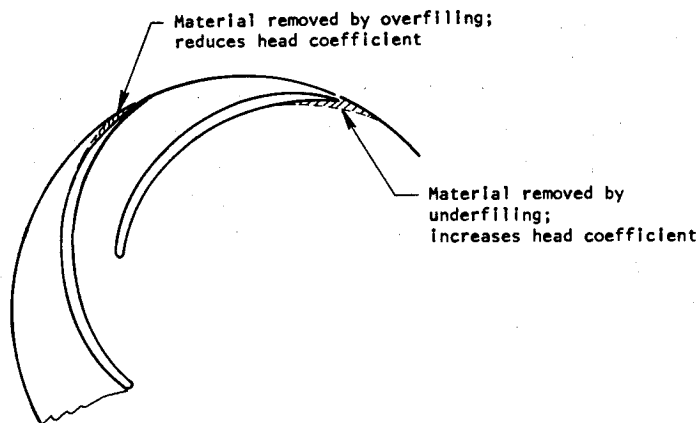
Figure 15. — Effect of filing impeller trailing edge.
