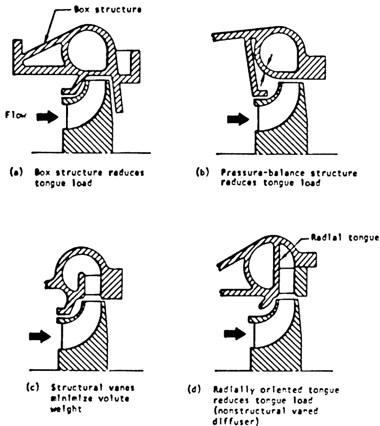
Figure 30. – Volute structural geometries.
