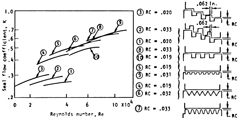
Figure 22. — Variation of seal flow coefficient with Reynolds number (various seal configurations).
