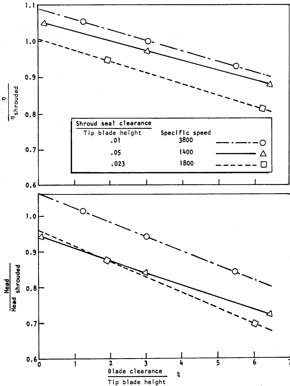
Figure 21. — Relative performance of open-face and shrouded impellers.
