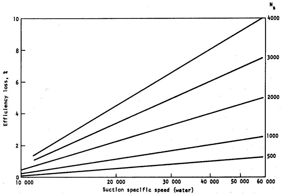
Figure 9. — Influence of suction specific speed on efficiency.
