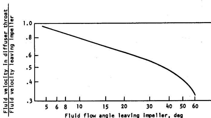
Figure 25. — Relative velocities in diffuser throat and at impeller discharge as a function of fluid flow angle.
