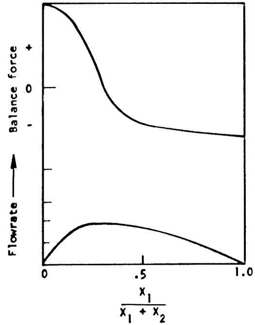
(a) Integral series-flow balance piston
