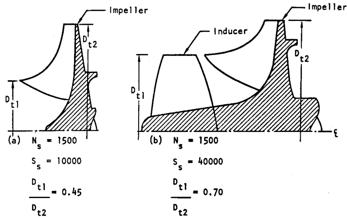
Figure 8. — Influence of suction specific speed on pump geometry.
