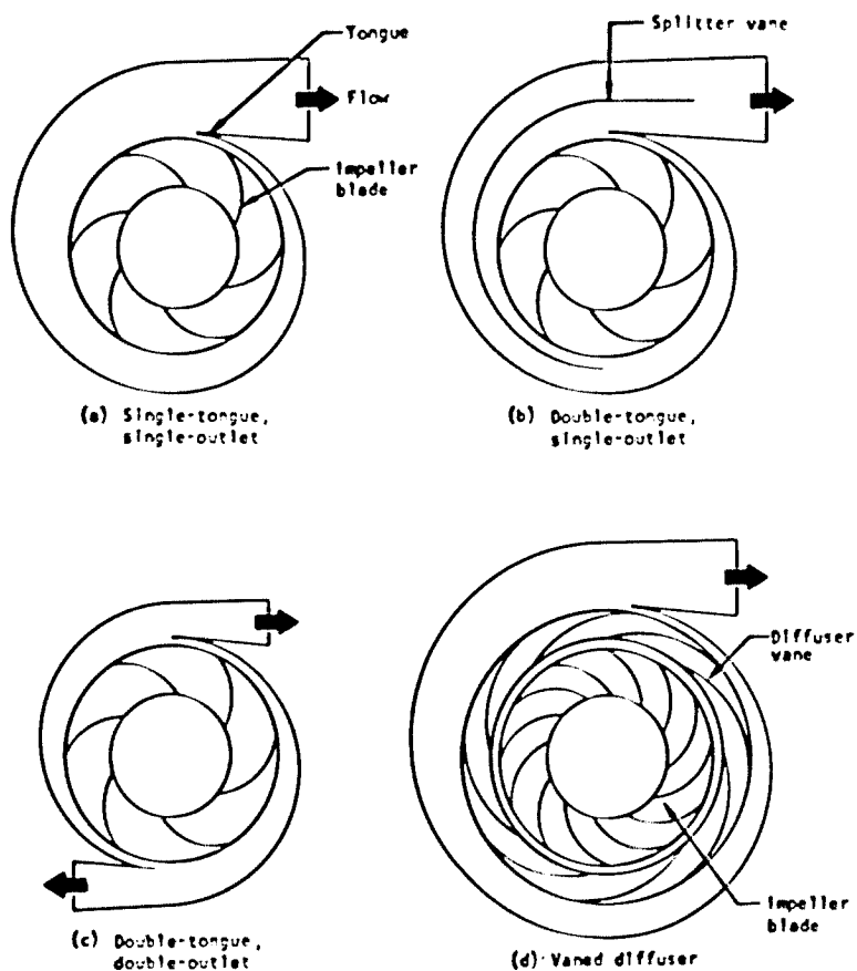
Figure 28. – Volute configurations.
