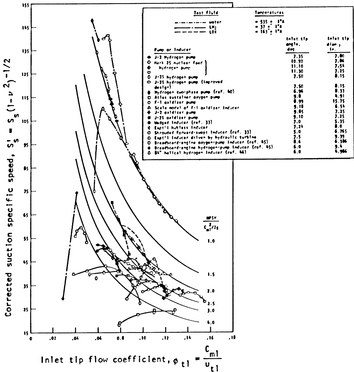
Figure 4. - Summary of empirical data on suction performance of various pumps and inducers.
