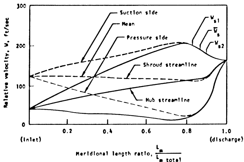
Figure 17. - Calculated relative velocities along hub and shroud streamlines for 12-gpm LF 2 -pump impeller.
