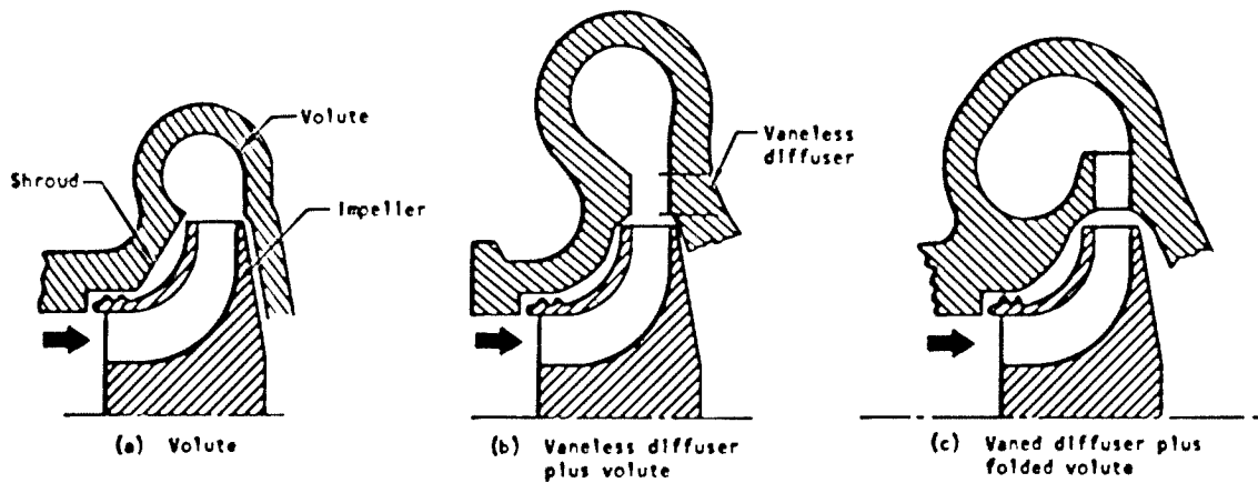
Figure 10. – Geometries for three types of diffusing systems.
