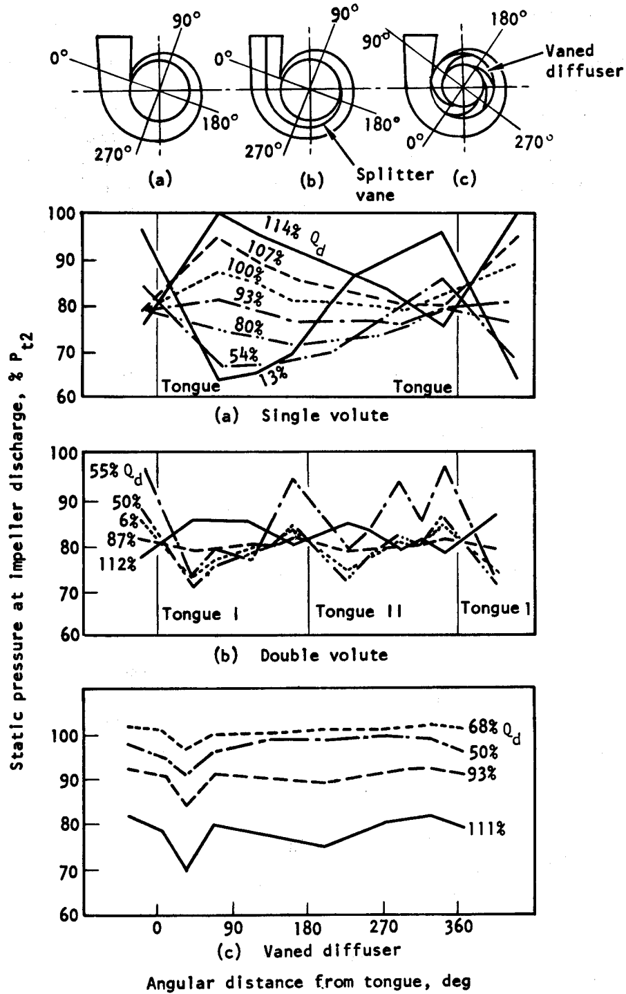
Figure 29. — Impeller discharge pressure as a function of volute design and percent design flowrate.
