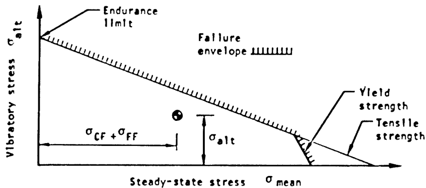
Figure 23. - Typical modified Goodman diagram.
