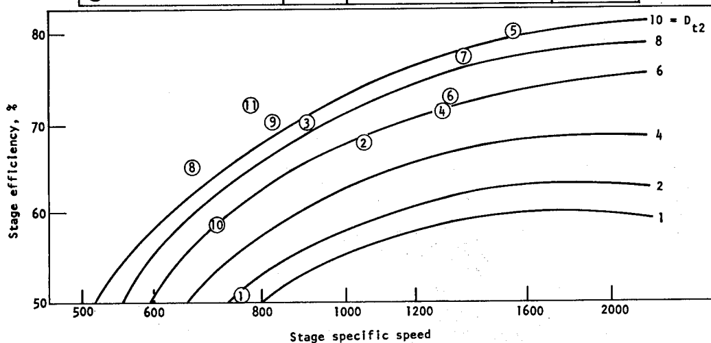
Figure 6. — Influence of pump size on efficiency.
