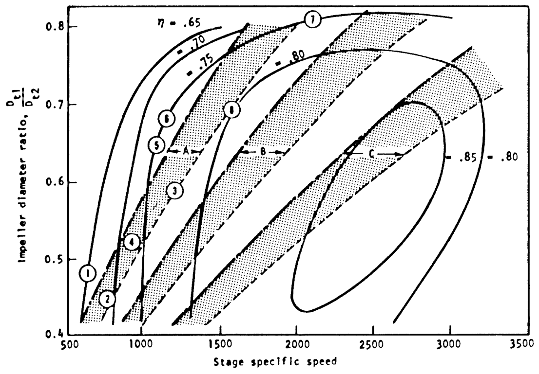
Figure 5. — Influence of impeller diameter ratio on pump performance.
