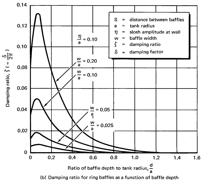
Figure 3. Ring-baffle damping in cylindrical tanks
