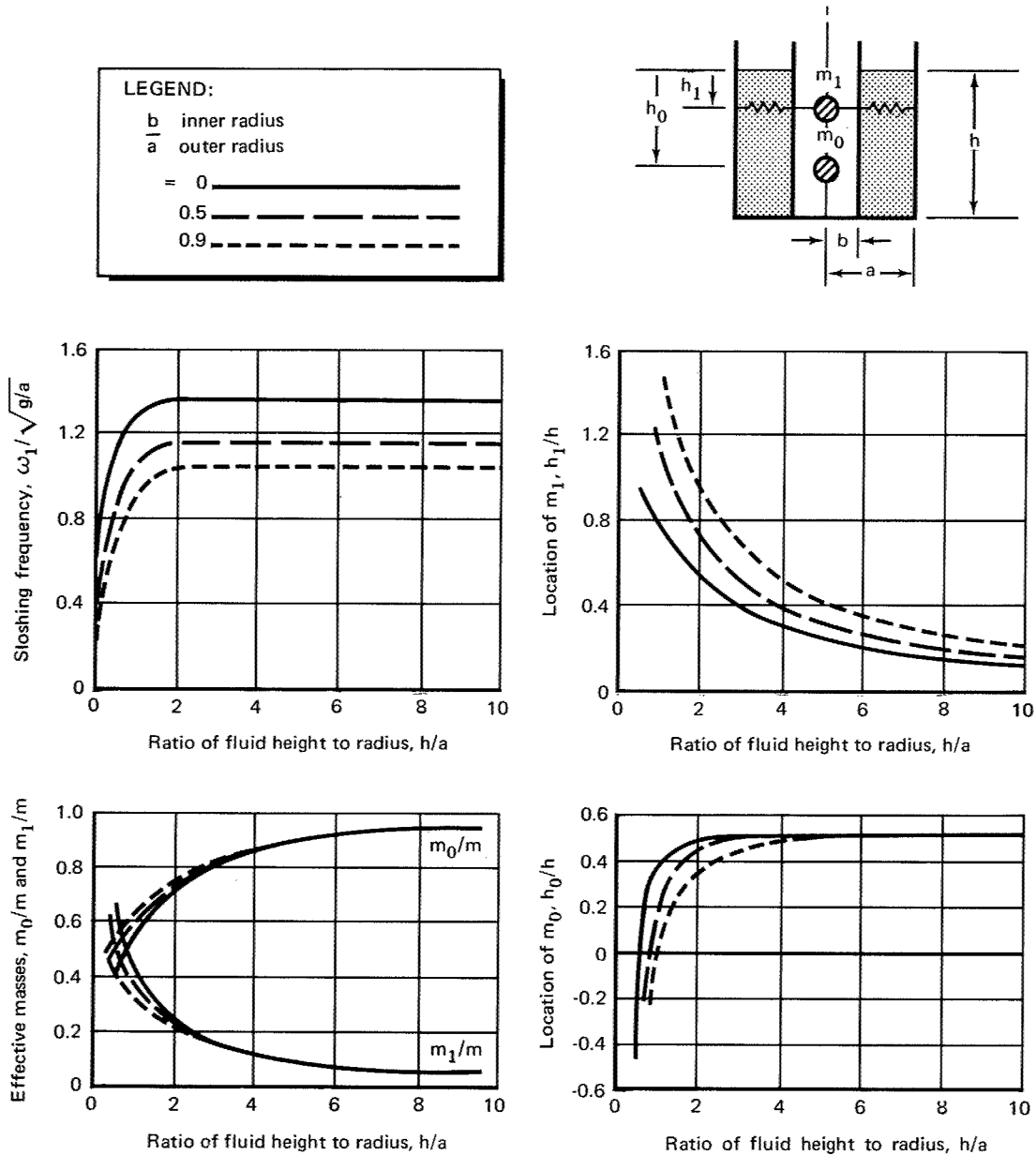
Figure 1 Frequency, effective masses, and mass attachment points for the lumped spring-mass model representation of first-mode lateral sloshing in circular cylindrical ring tanks for various ratios of inner tank radius to outer tank radius.
