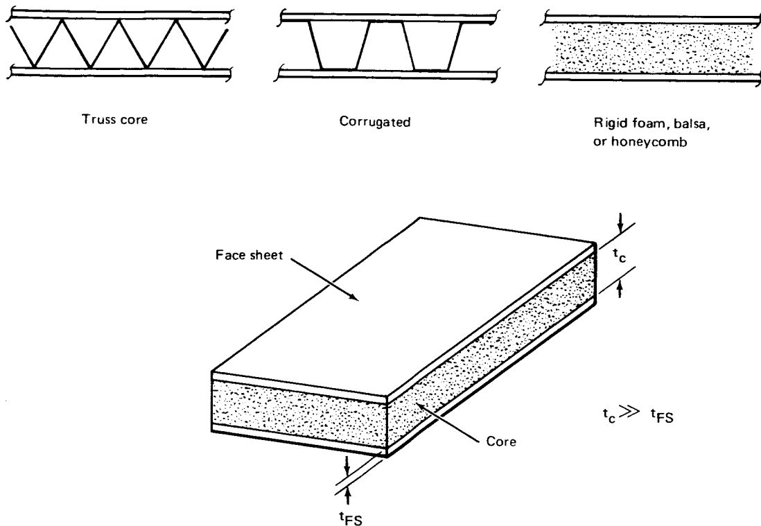
Figure 3. — Sandwich-plate construction.
