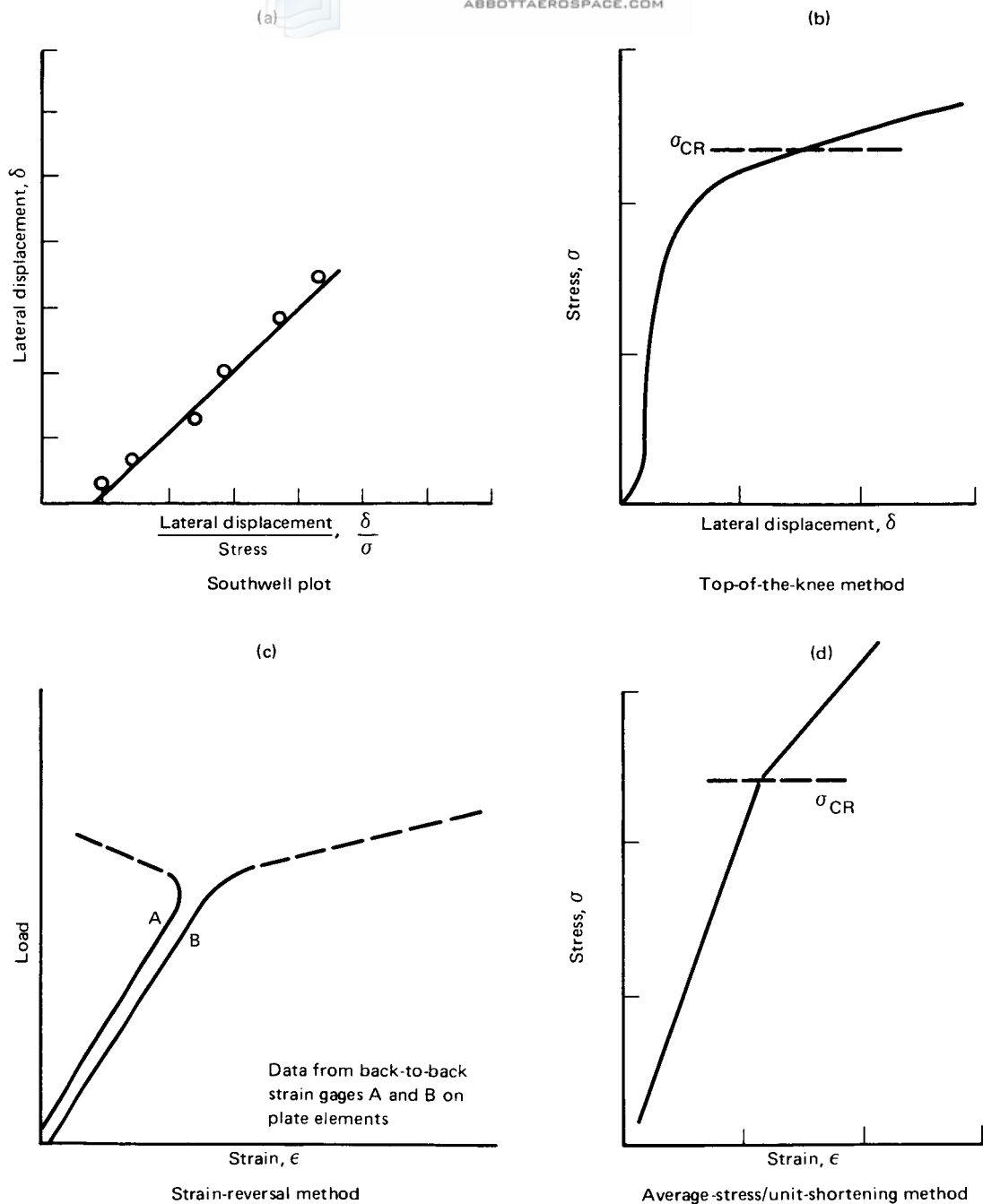
Figure 5. — Methods for identifying buckling stress from experimental data.
