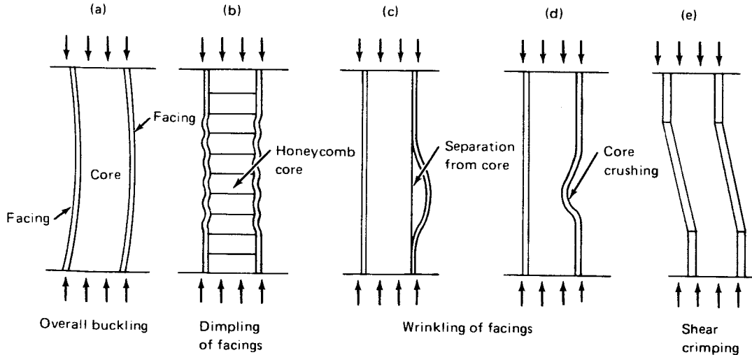
Figure 4. — Typical failure modes of sandwich plates.
