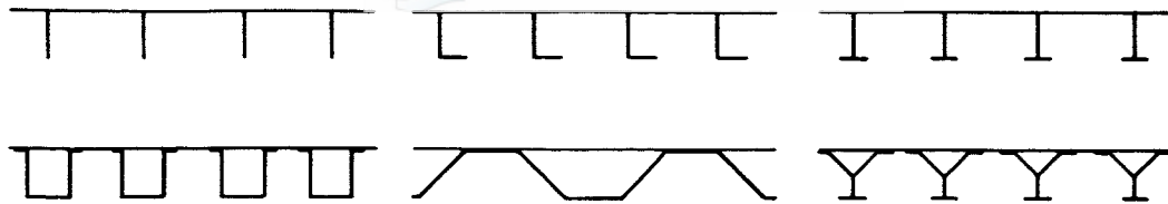
Figure 1. – Types of stiffeners used in stringer-stiffened plate construction.
