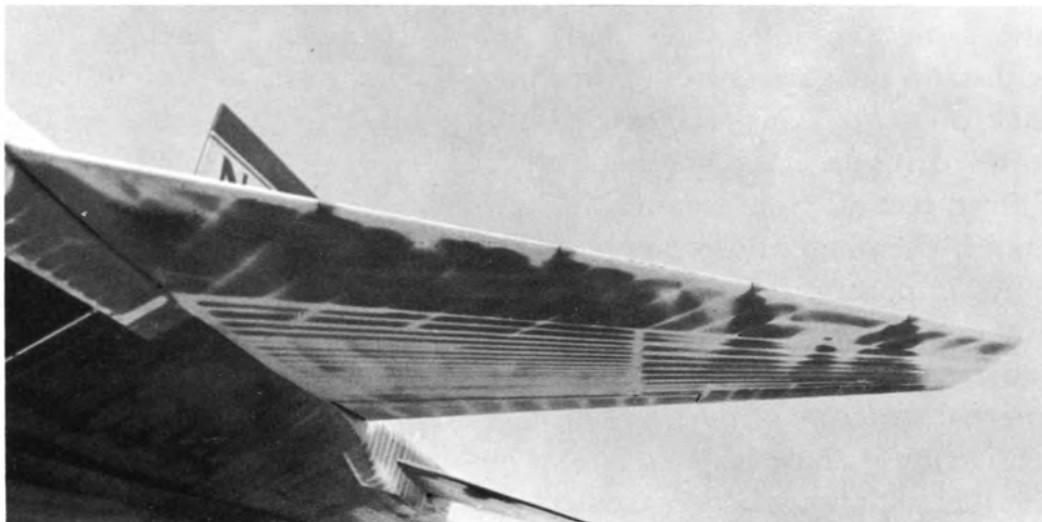
Temperature-indicating paint strikingly reveals the uneven heating to which the X-15's heat-sink wing structure was subjected during a high-heating mission. Dark areas indicate the higher temperature. Light areas reveal internal structure.
