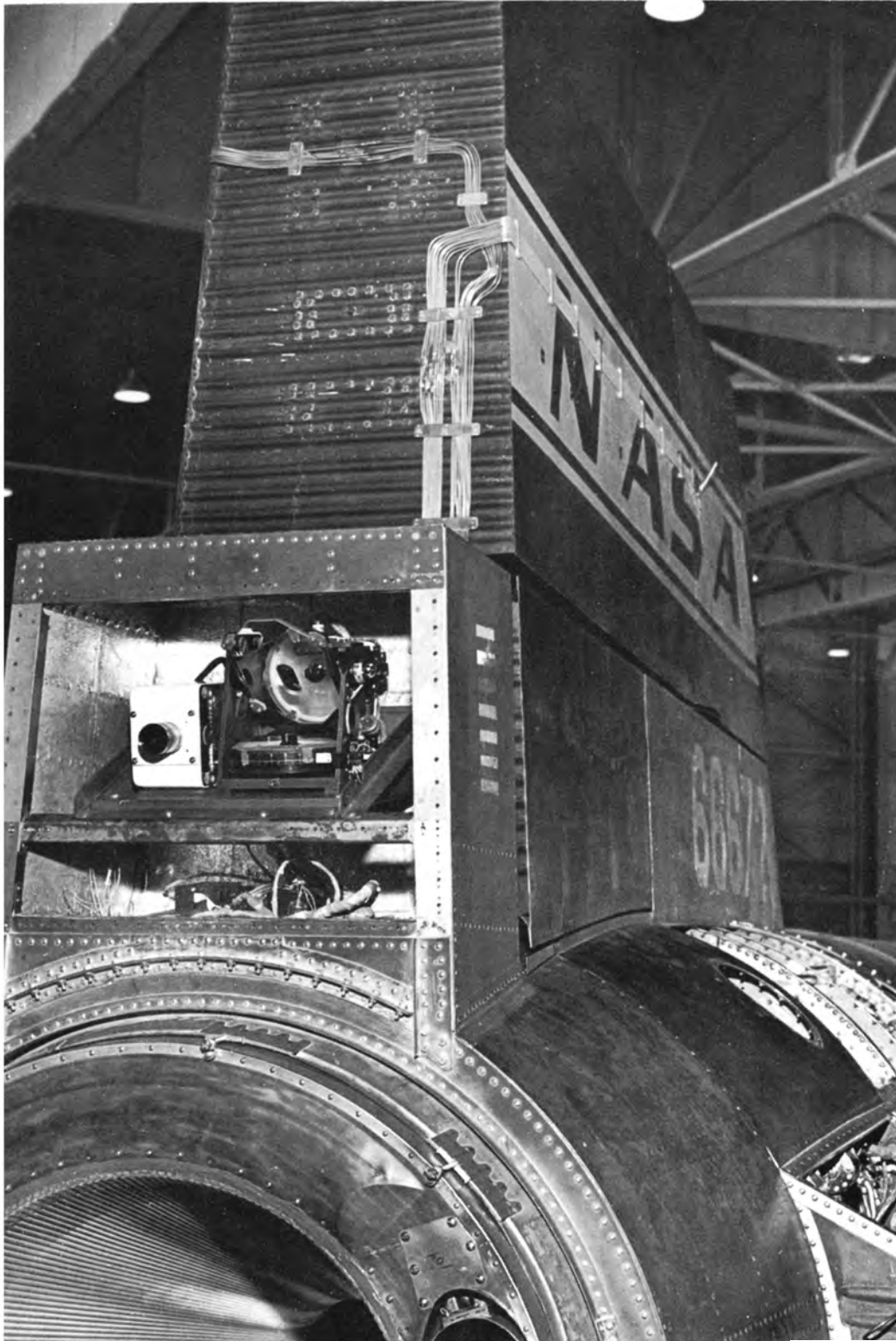
An infrared horizon-scanner, with cover plate removed, is seen here in its compartment behind the upper speed brakes of an X-15 before a research flight to high altitude. The instrument helped measure background noise for the design of satellite instruments. Those bundles of stainless-steel pressure tubes on the aft end of the upper vertical tail lead to pressure rakes on the sides of the tail.
