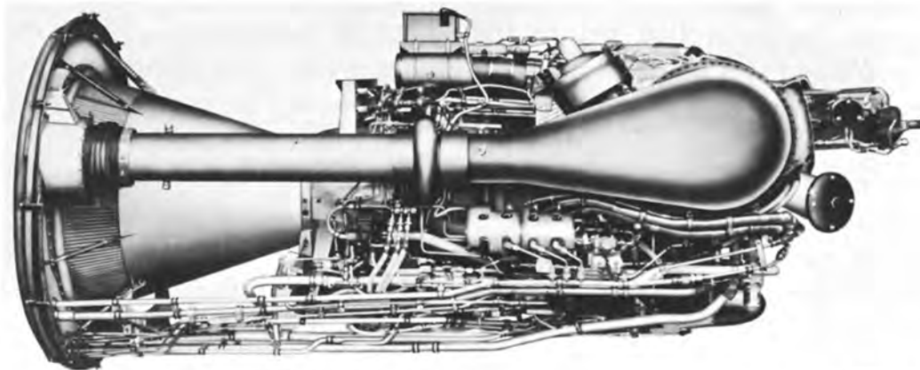
A closeup of the X-15's remarkable XLR-99 rocket engine. Its 57 000-lb. maximum thrust is equivalent at burnout to 600 000 hp. The engine can be throttled from 40-percent to 100-percent thrust. Its propellants flow at the rate of 13 000 lb. per minute at maximum thrust, exhausting the entire 18 000-lb. fuel supply in 85 seconds. The engine's nozzle diameter is 39.3 in.; its over-all length, 82 in.; its weight, 1025 lb.
