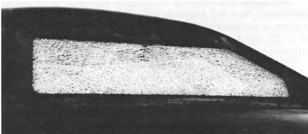
A noteworthy scar of the X-15's first flight to Mach 6 was this cracked outer panel on the right side of the windshield. Investigators found that thermal stresses higher than expected in the metal retainer holding the glass had caused the cracking.
