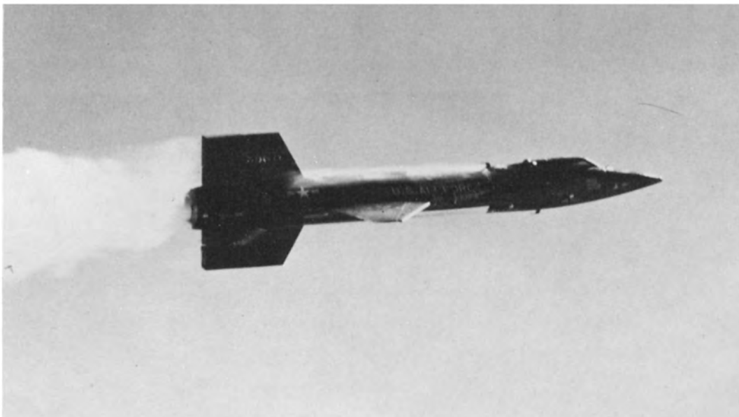
An instant or two after launch, the X-15 is seen roaring off on its own, with Inconel X skin glistening in the sun. At burnout, it will be accelerating at 4 G's, or 90 additional miles per hour every second.
