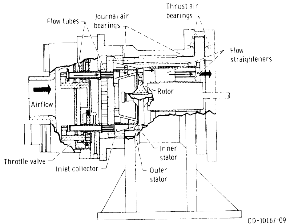
FIGURE 12-15.—Airbrake dynamometer.
