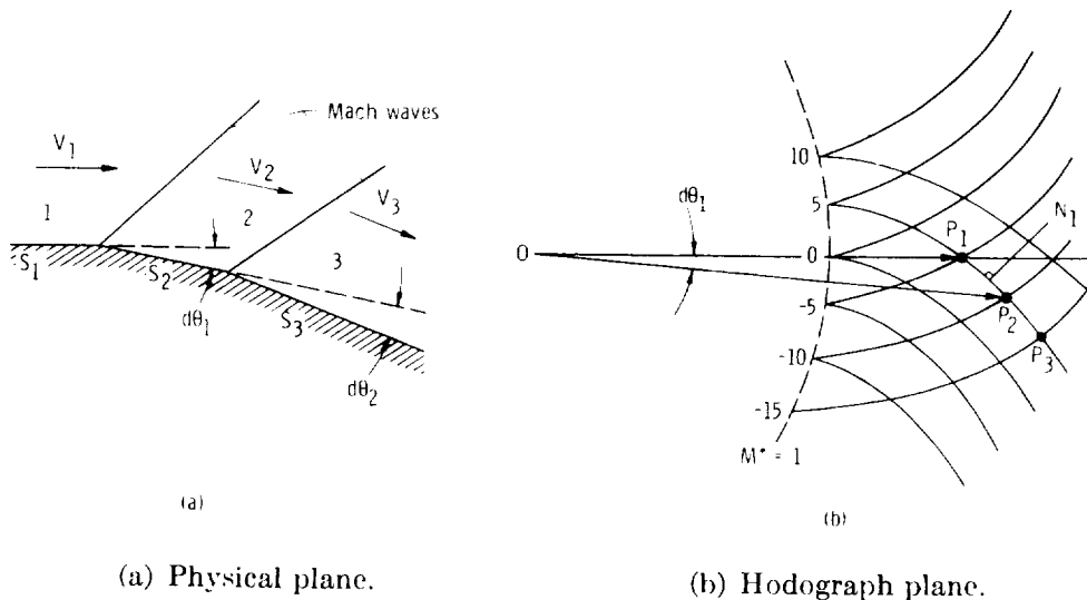
FIGURE 9-7.—Flow along convex wall.
