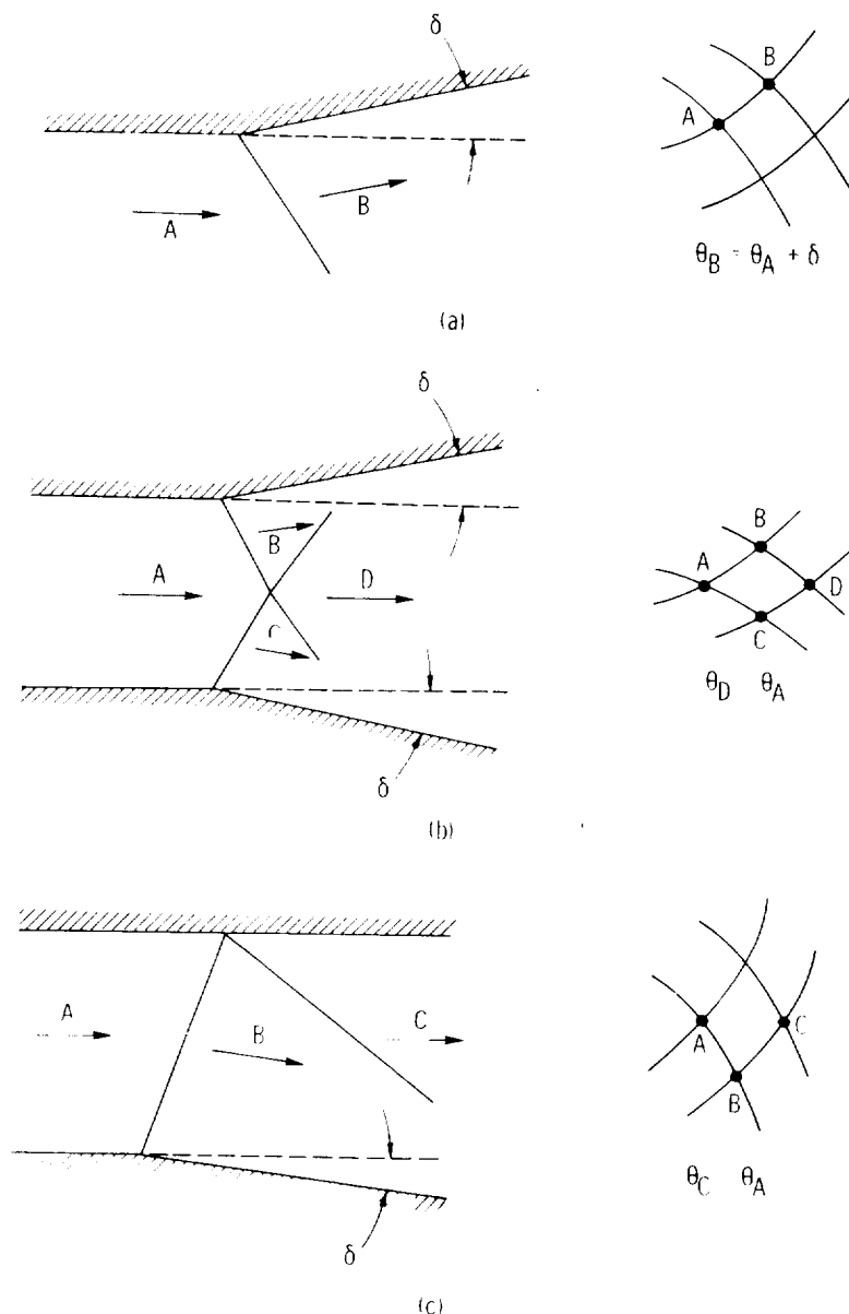
(a) Weak expansion wave. (b) Intersection of expansion waves. (c) Reflection of an expansion wave from a solid boundary. FIGURE 9-10.—Elementary flow solutions.
