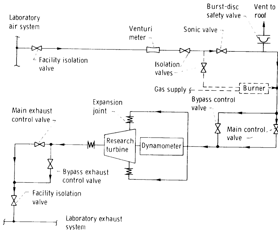
FIGURE 12-1.—Flow schematic of a turbine test facility.
