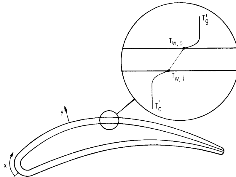
FIGURE 11-1.—Simplified one-dimensional model.
