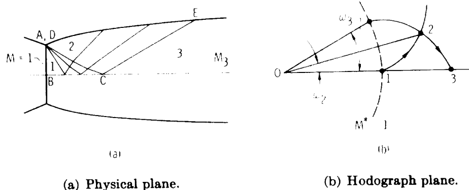
FIGURE 9-12.—Nozzle with sharp-edged throat.
