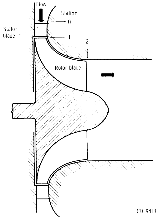
FIGURE 10-1.—Schematic cross section of radial-inflow turbine.
