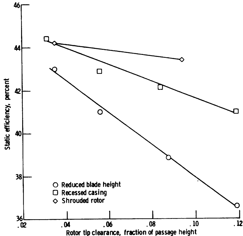
FIGURE 8-5.—Effect of tip-clearance configurations on turbine efficiency. (Data from ref. 4.)
