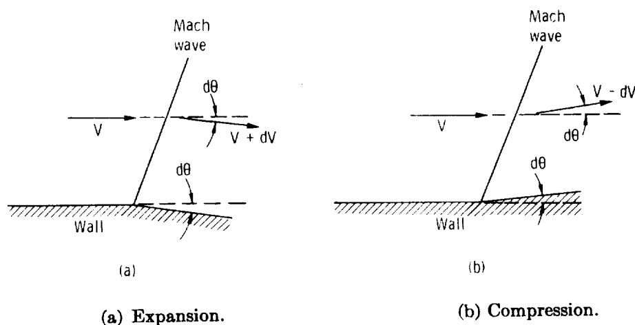
FIGURE 9-1.—Weak expansion and compression waves.
