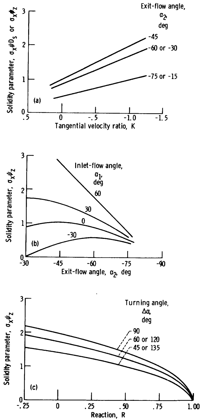
(a) Effect of tangential-velocity ratio and exit-flow angle. (b) Effect of exit- and inlet-flow angles. (c) Effect of reaction and turning angle. FIGURE 4-2.—Effect of velocity diagrams on solidity.
