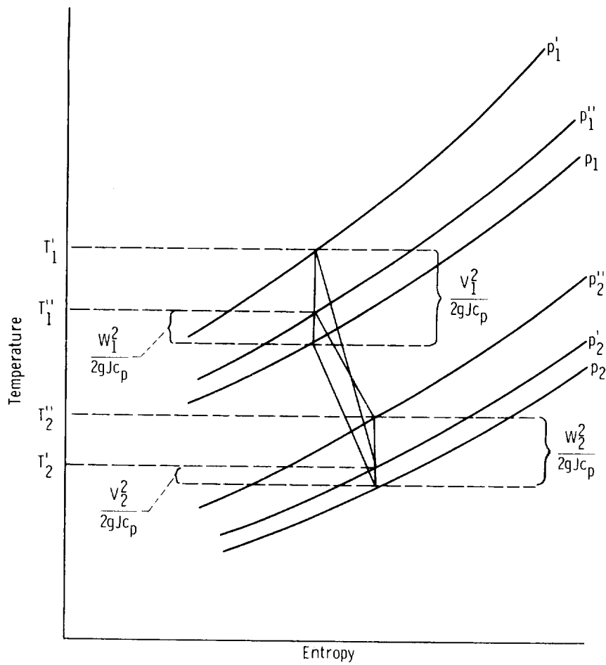
FIGURE 10-4.—Temperature-entropy diagram for a radial-inflow turbine rotor.
