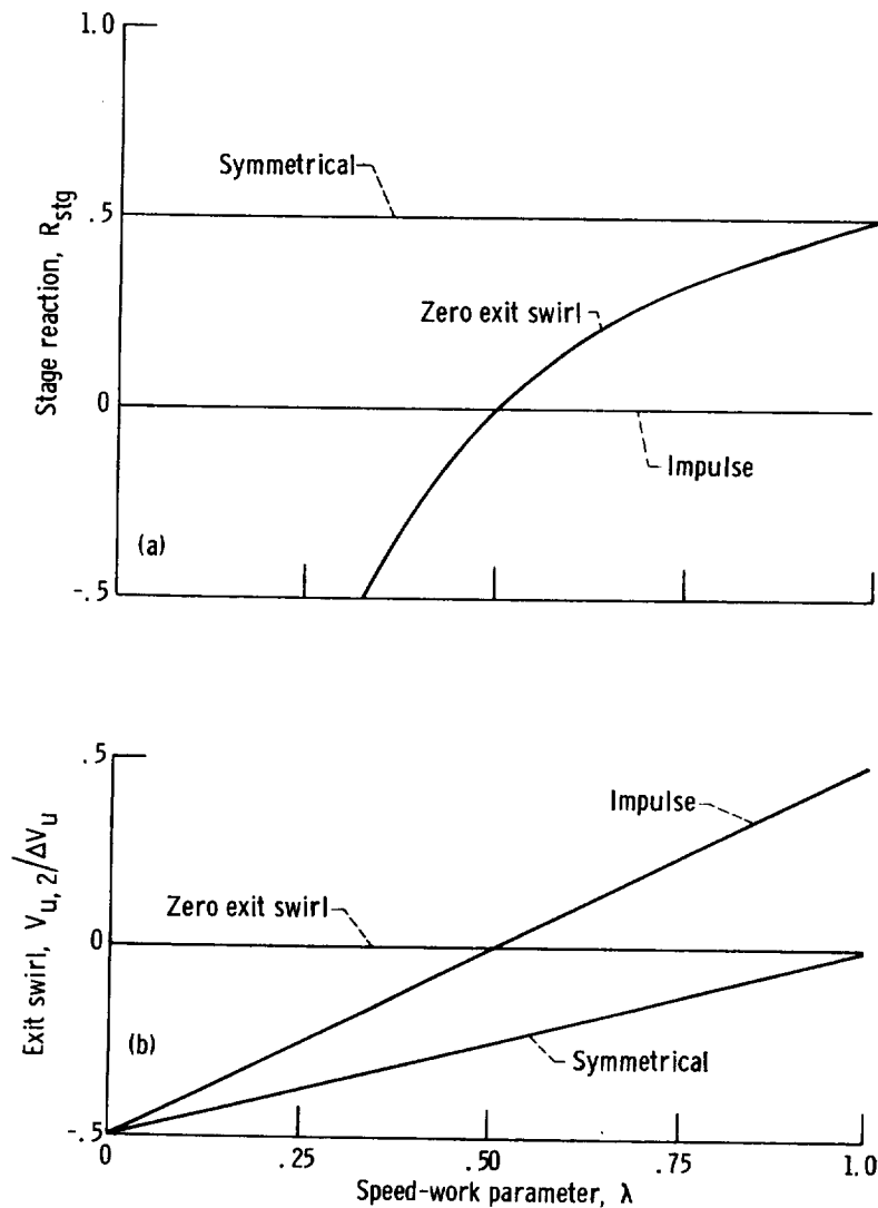
FIGURE 3-3.—Effects of speed-work parameter and velocity-vector diagram type on reaction and exit swirl.
