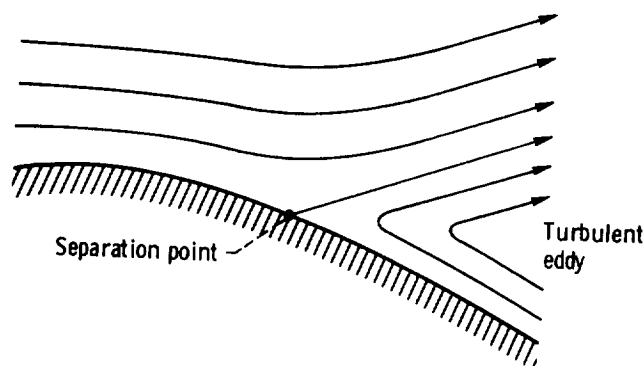
FIGURE 6-3.—Boundary-layer separation.
