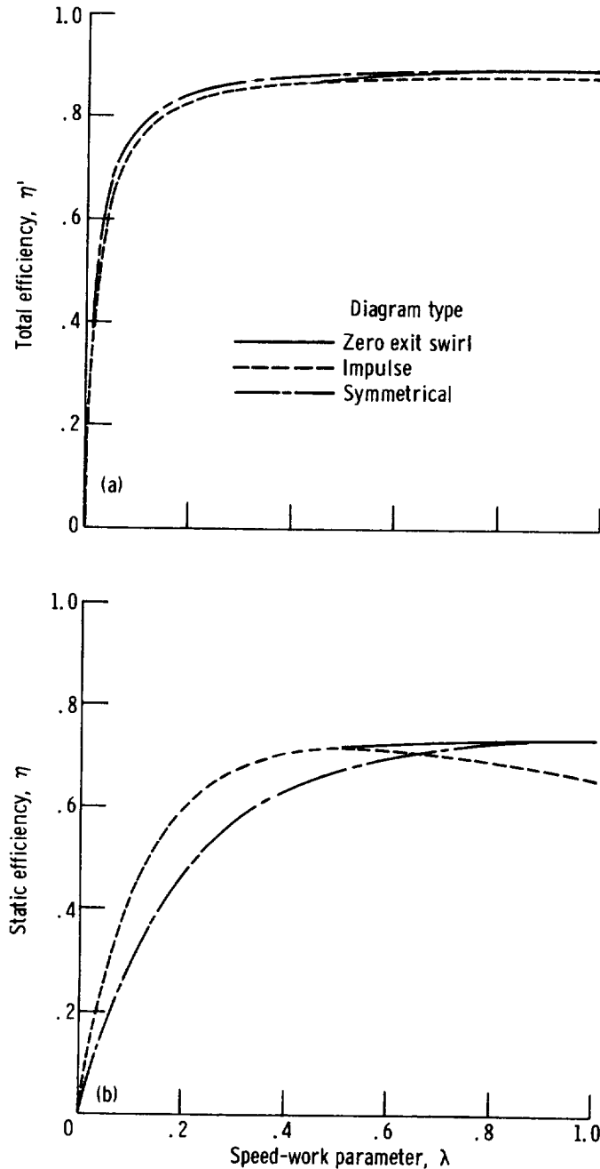
FIGURE 3-4.—Effects of speed-work parameter and velocity-vector diagram type on efficiency. (Curves from ref. 2.)
