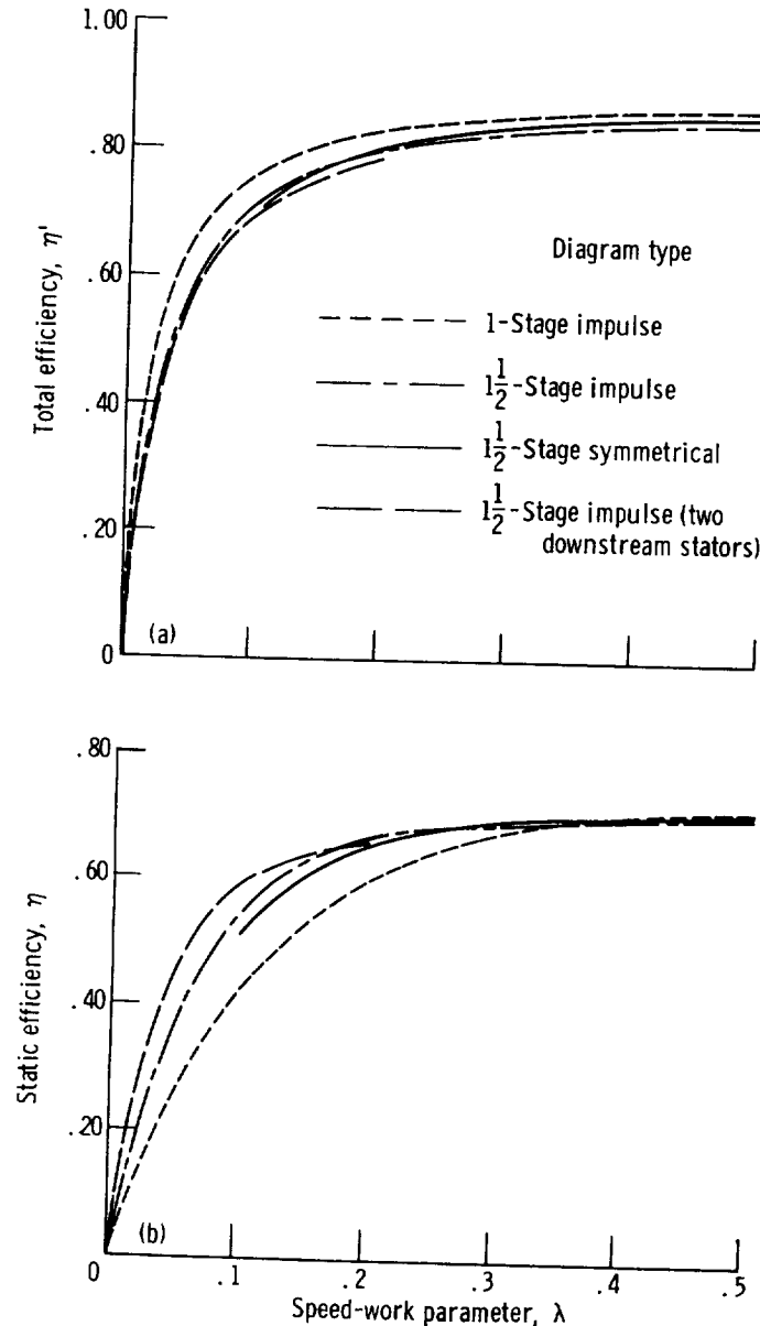
FIGURE 3-6.—Effect of downstream stator on efficiency. (Curves from ref. 3.)
