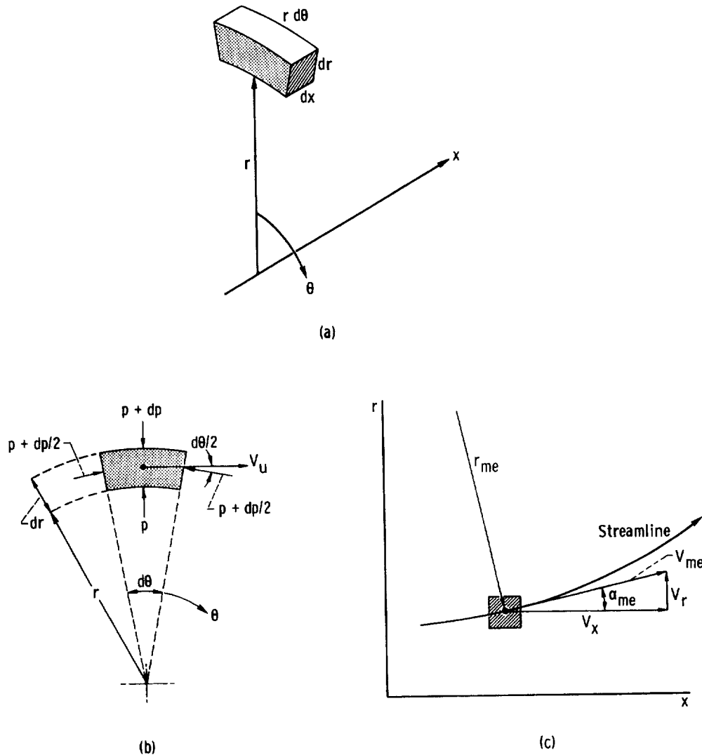
(a) Element of fluid in turbine flow field. (c) Meridional plane ( r-x ). (b) Rotation plane ( r-\theta ). FIGURE 3-10.—Radial equilibrium factors.
