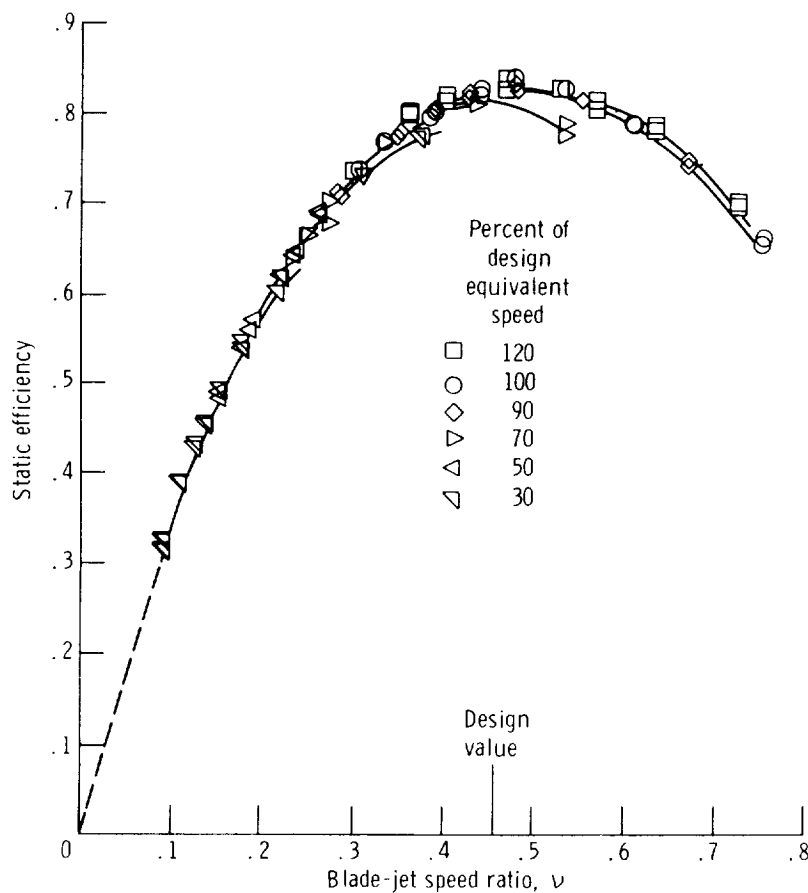
FIGURE 12-21.—Variation of efficiency with blade-jet speed ratio.
