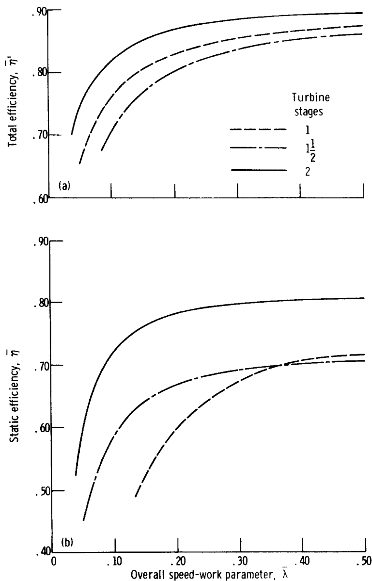
FIGURE 3-7.—Comparison of efficiencies of 1-, 1½-, and 2-stage turbines. (Curves from ref. 4.)
