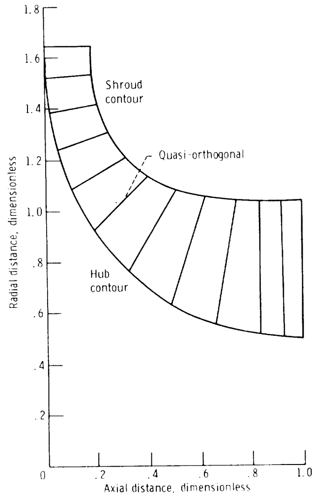
FIGURE 10-18.—Meridional section through radial-inflow turbine.
