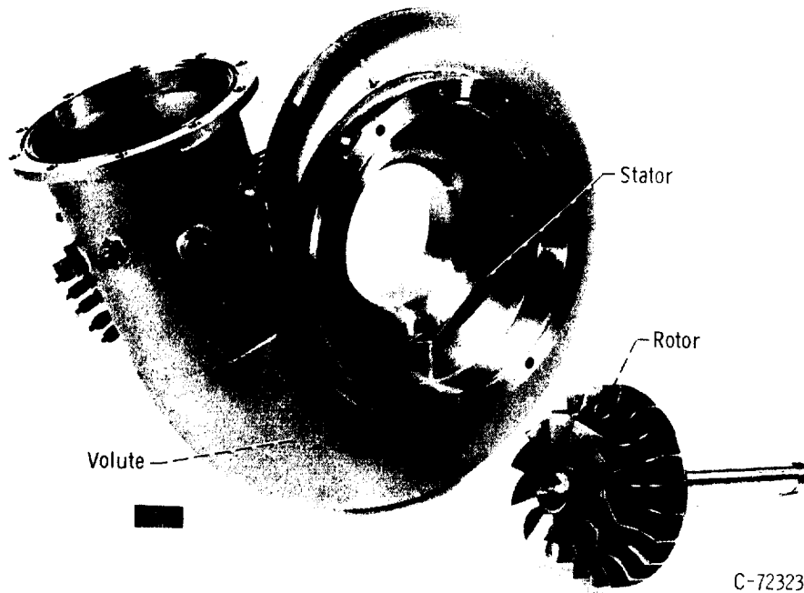
FIGURE 10-2.—Radial-inflow turbine.
