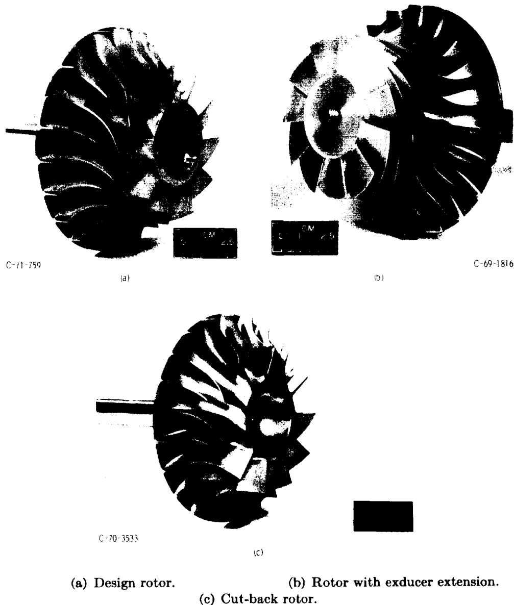
FIGURE 10-14.—Rotor configurations used in specific-speed study of reference 8.
