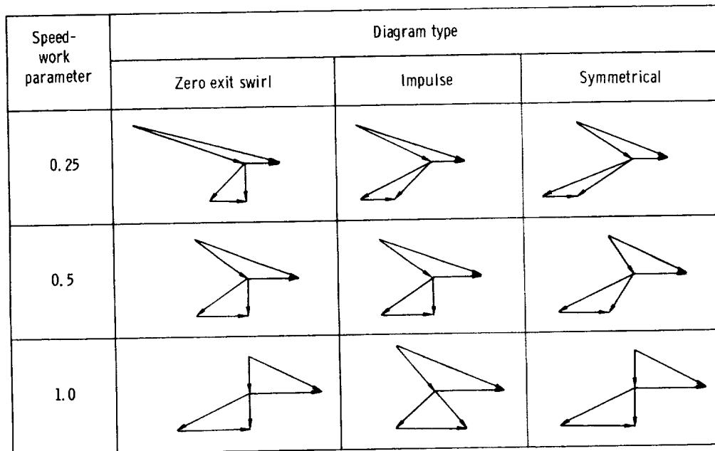
FIGURE 3-2.—Effects of speed-work parameter and diagram type on shape of stage velocity-vector diagram.
