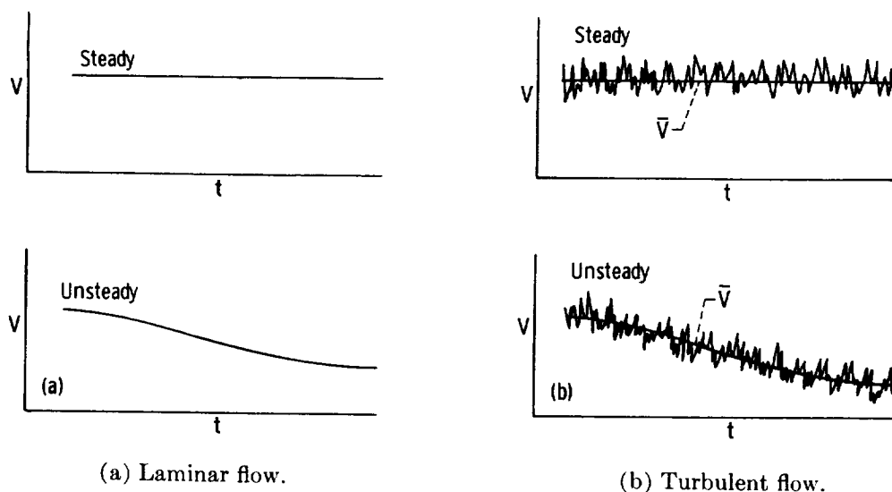
FIGURE 6-2.—Variation of velocity with time at a point.
