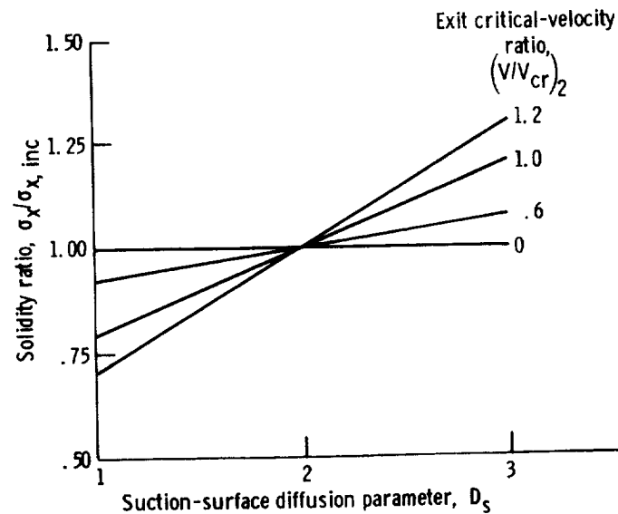
FIGURE 4-3.—Effect of compressibility on axial solidity.
