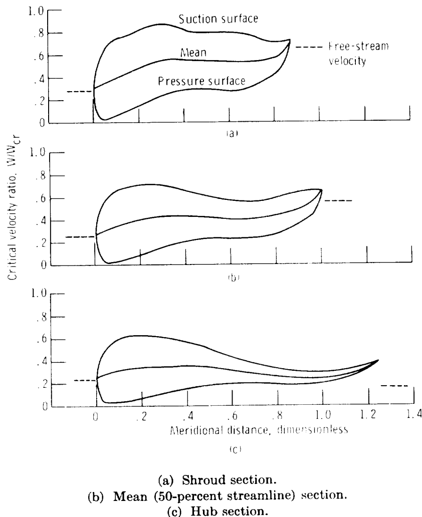
FIGURE 10-20.—Rotor-blade surface-velocity distributions from stream-function solution.
