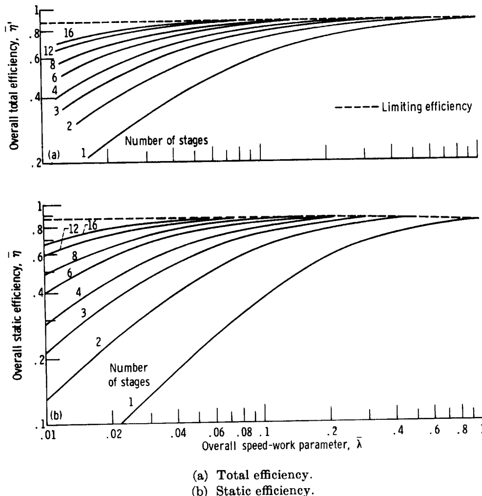
FIGURE 3-9.—Overall efficiency characteristics. (Curves from ref. 6.)
