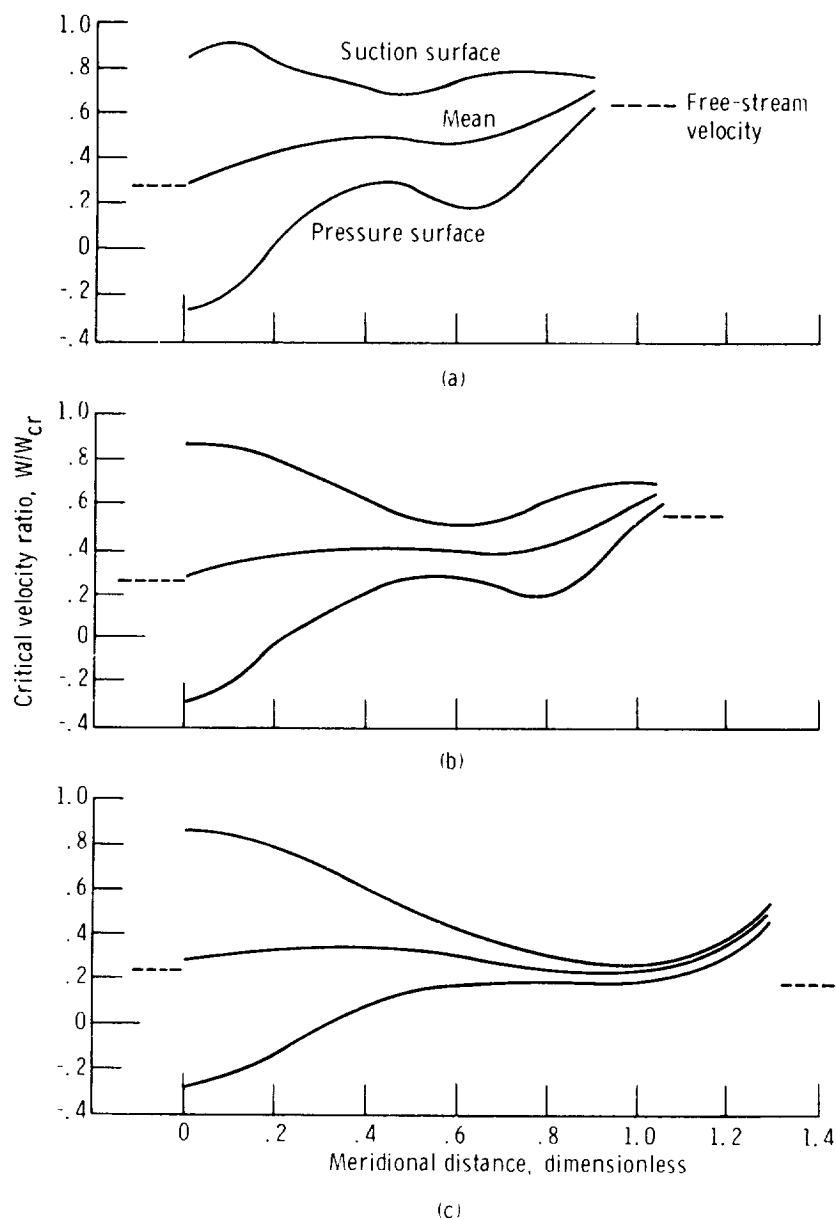
(a) Shroud section. (b) Mean (50-percent streamline) section. (c) Hub section.
