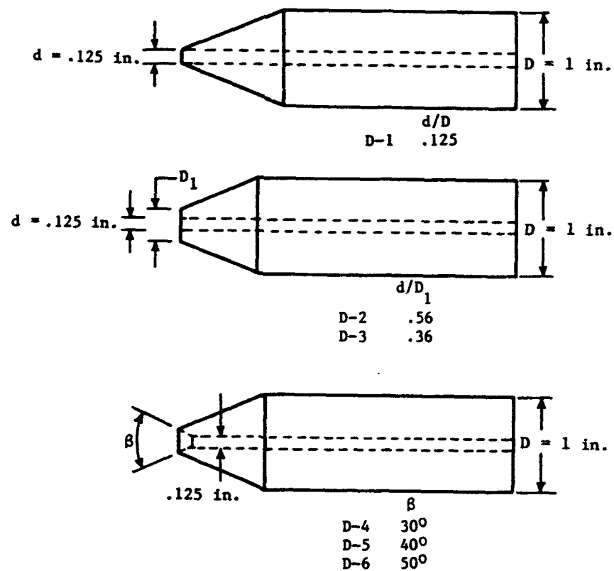
(e) Series D - 45° conical nose.
