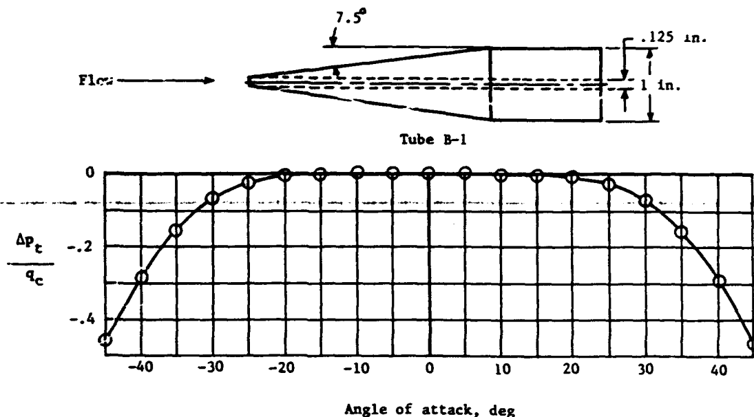
(a) 15° conical-nose tube.
