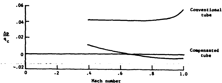
(a) F-104 airplane. (Adapted from ref. 4.)
