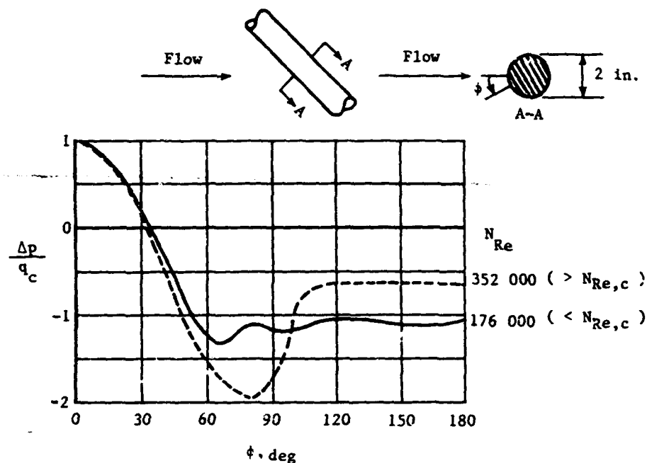
Figure 6.9.- Pressure distribution around a cylinder at an angle of attack of 45° and a Mach number of 0.2. The two pressure distributions are for flow conditions below and above the critical Reynolds number N_{Re,c} at which flow separation occurs. (Adapted from ref. 7.)
