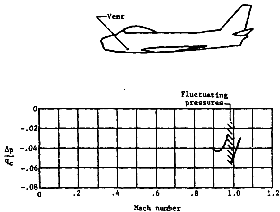
Figure 7.19.- Variation of static-pressure error of a fuselage-vent installation in transonic speed range. (Adapted from ref. 11.)
