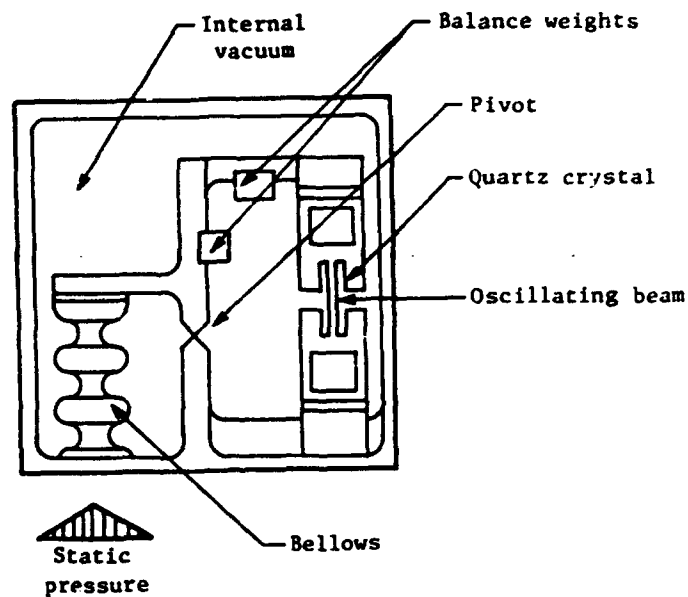
(a) Absolute-pressure transducer.
