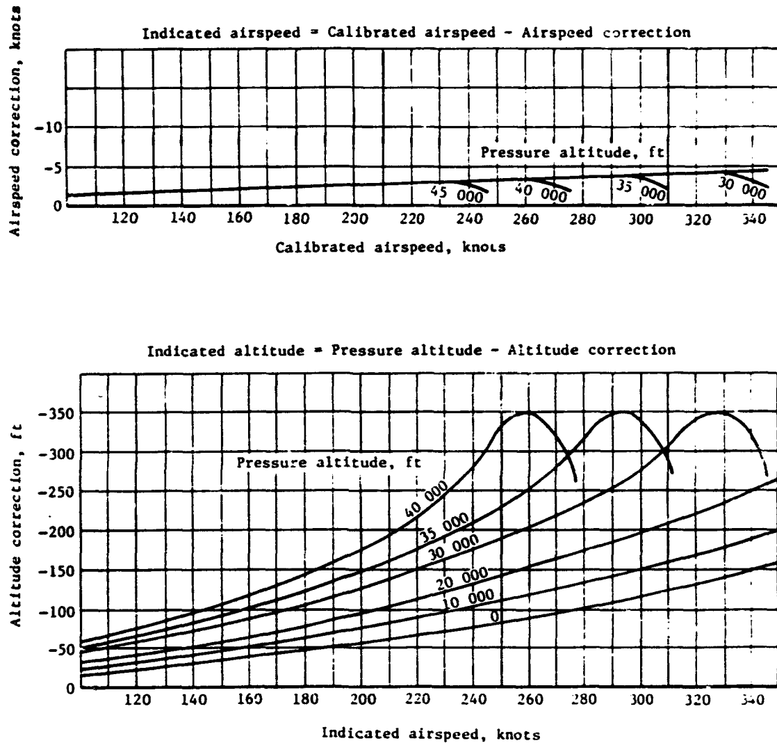
Figure B1.- Flight-manual correction charts for the airspeed and altitude errors of the static-pressure installation of an airplane. These correction charts are used to determine the indicated airspeed and indicated altitude at which the airplane should fly to achieve a desired calibrated airspeed and pressure altitude.
