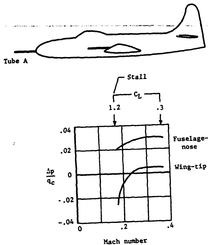
Figure 7.13.- Variation of static-pressure errors of wing-tip and fuselage-nose installations of same boom length. (Adapted from ref. 8.)
