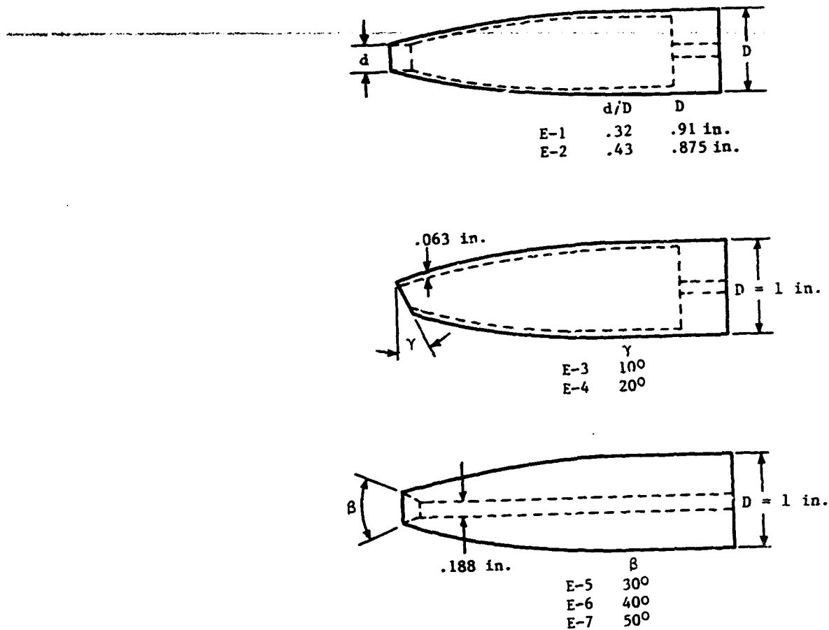
(f) Series E - ogival nose.
