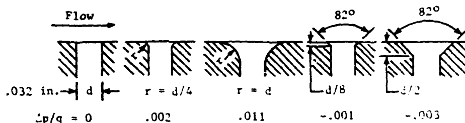
(b) Effect of orifice edge shape. Error \pm 0.001 and angled edge shapes referred to error of square-edge orifice.
