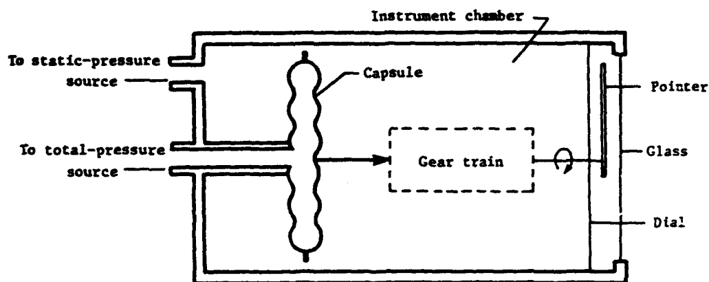
(b) Differential-pressure capsule. For an increase in total pressure inside the capsule, the capsule deflects in the direction indicated by the large arrow.
