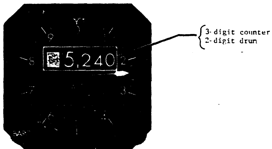
Figure 11.10.- Counter-drum-pointer servoed altimeter. (Courtesy of Harowe Systems, Inc.)
