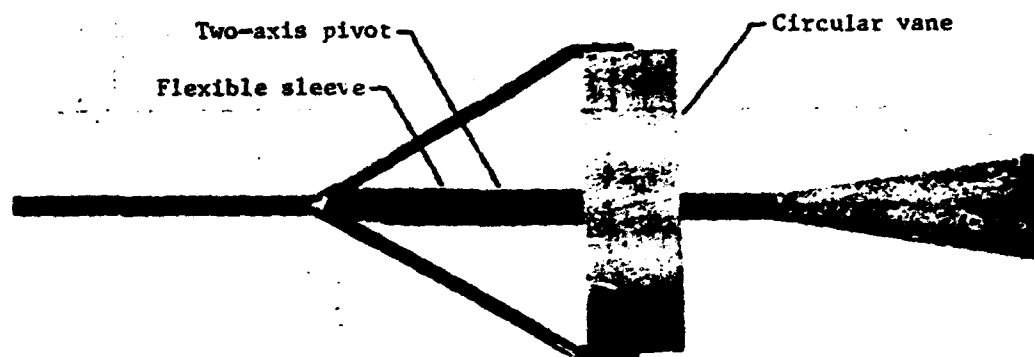
(b) Swiveling total-pressure tube.
