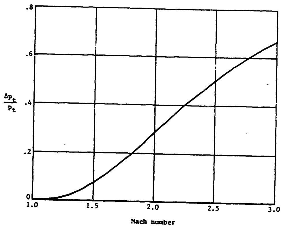
Figure 4.2.- Total-pressure loss through a normal shock wave.
