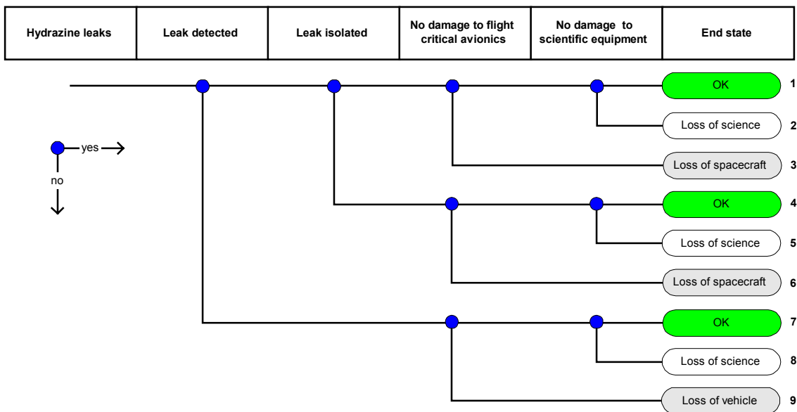
Figure 3-7: Event Tree for the Hydrazine Leak
