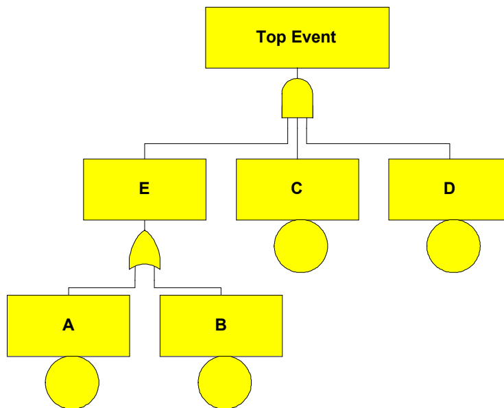
Figure 6-9: Typical Fault Tree Structure
