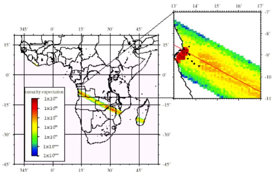
Figure 14-11: Casualty Expectation Distribution in Re-entry Accidents
