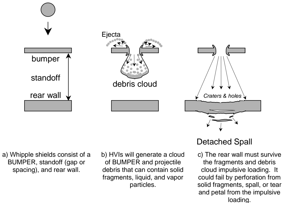
Figure 4.6-6. Whipple shield.
