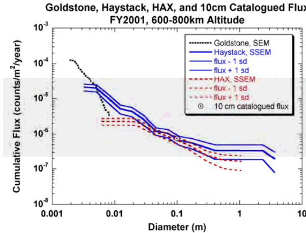
Figure 4.4-23. Cumulative Flux.
