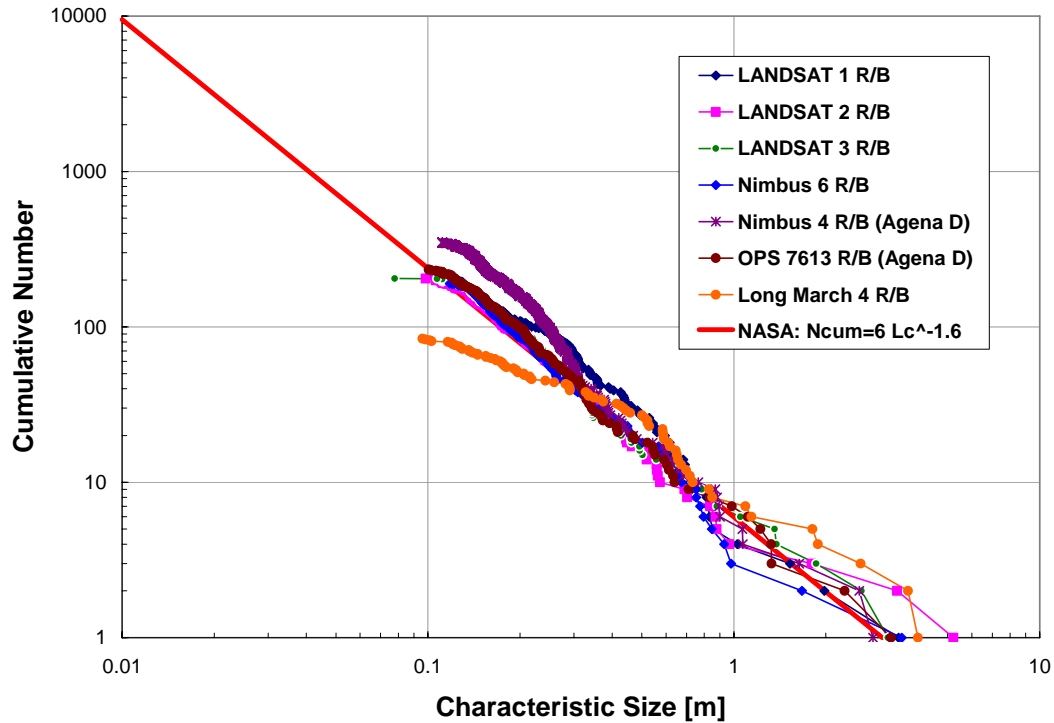
Figure 4.5-25. Sample debris size distributions from seven upper stage explosions, as derived from SSN data.
