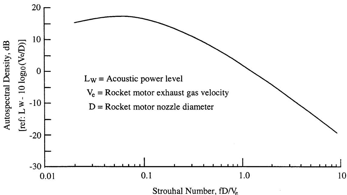
FIGURE 3.5. Normalized Autospectrum for Acoustic Power Generated by Rocket Engines/Motors.
