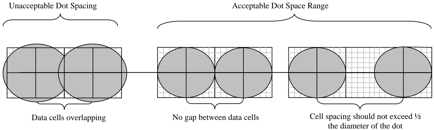
Figure 20—Proper Dot Pen Spacing
