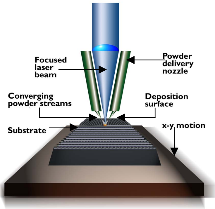
Figure 9—Schematic Illustration of the LENS Process
