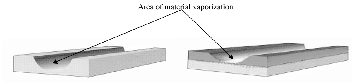
Figure 32—Laser Engraving Applied Directly to a Surface (left) and to a Surface Coating (right)
