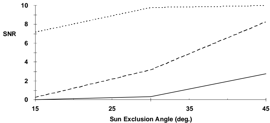
Figure 3-19. SNR increase due to particulate contamination.
