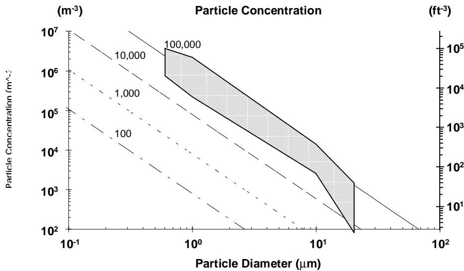
Figure 4-6. Prelaunch shuttle access platform air cleanliness.
