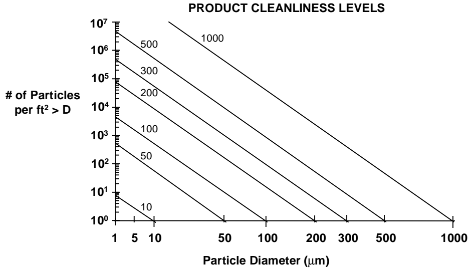
Figure 3-7. MIL STD 1246C surface particle cleanliness levels.
