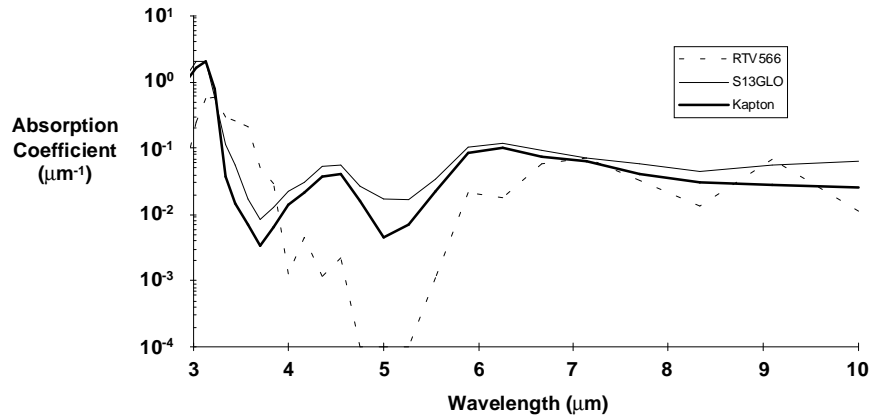
Figure 2-7. Absorptance profile of specific contaminants in the infrared.
