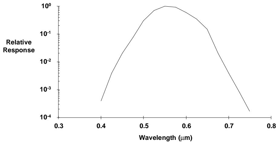
Figure 4-3. Response of the human eye to colors.
