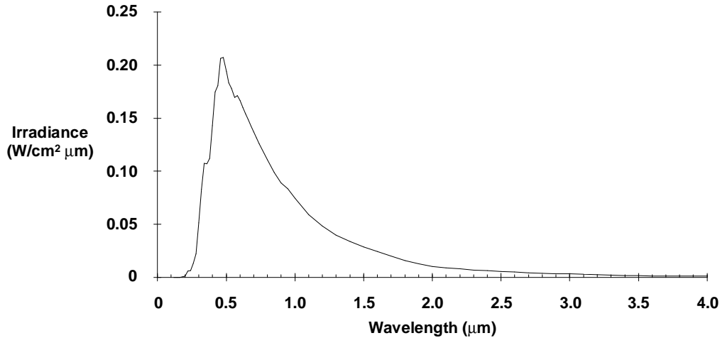
Figure 2-2. Solar flux as a function of wavelength.
