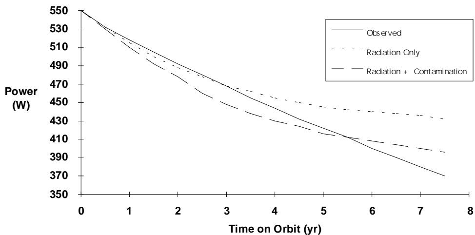
Figure 2-18. Evidence of photochemically deposited contamination on GPS Block I.
