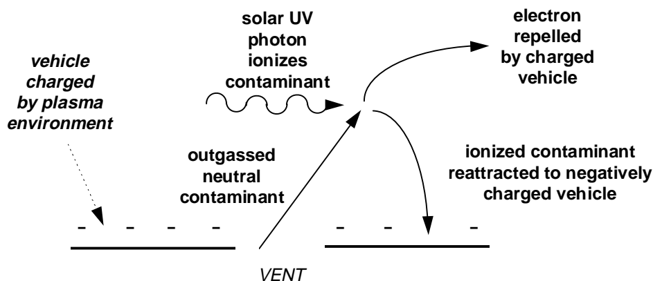
Figure 2-14. Electrostatic reattraction of ionized contaminants.
