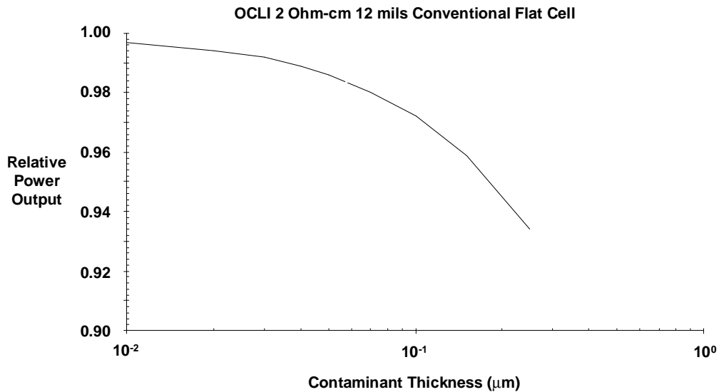
Figure 2-12. Effect of contamination on solar cell output.
