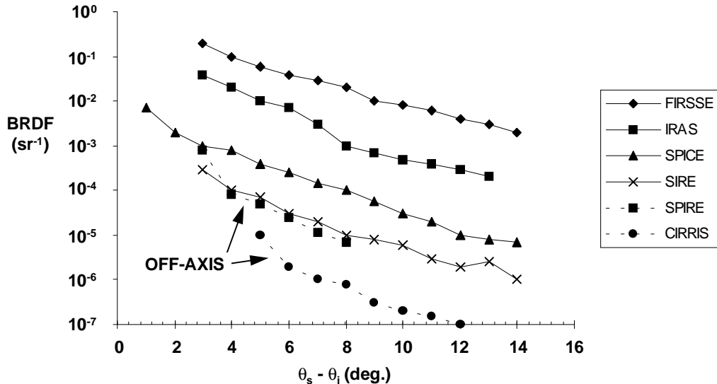
Figure 3-6. BRDF measurements for selected space sensors.
