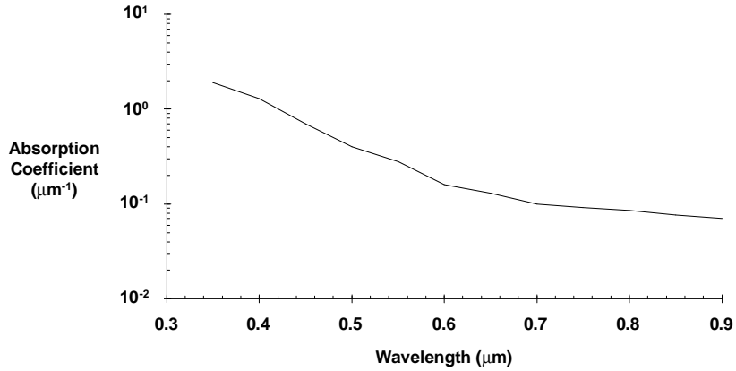
Figure 2-6. Absorptance profile of “typical” spacecraft contaminants in the visible.
