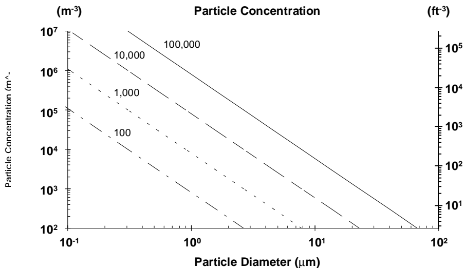
Figure 3-14. FED STD 209E air quality classifications.
