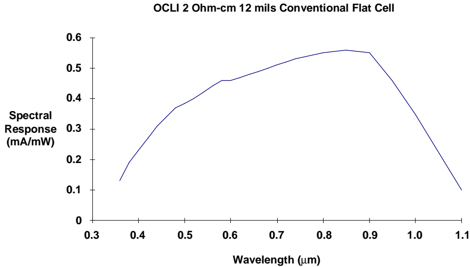
Figure 2-11. A typical solar cell response curve.
