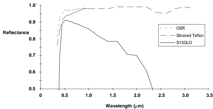
Figure 2-5. Reflectance values for three typical spacecraft thermal control materials.
