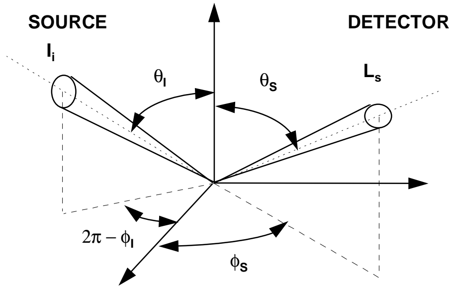
Figure 3-5. BRDF geometry.
