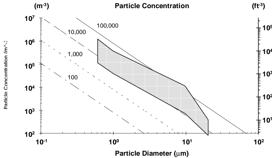
Figure 4-7. Prelaunch shuttle bay air cleanliness.
