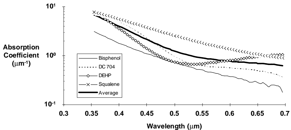
Figure 2-20. Absorbance profile of photochemically deposited films.
