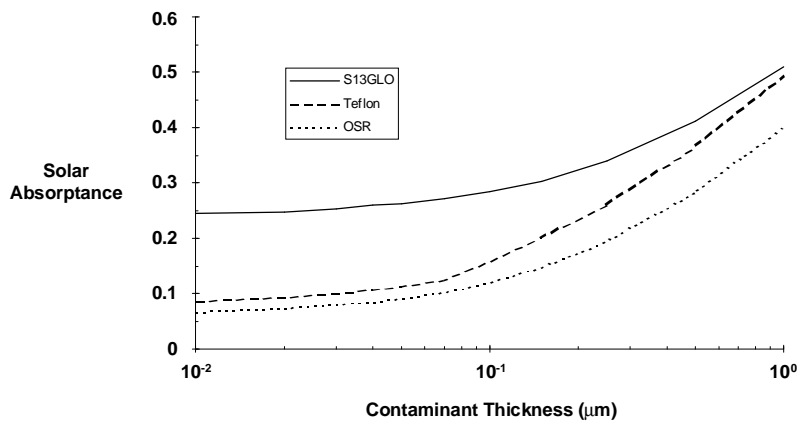
Figure 2-8. Solar absorptance as a function of contaminant thickness.
