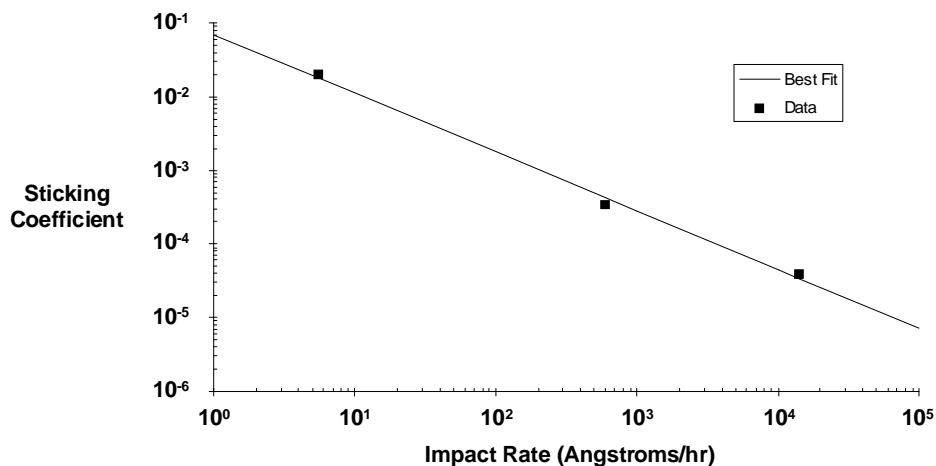
Figure 2-19. Photochemical deposition absorption ratio vs. impact rate.
