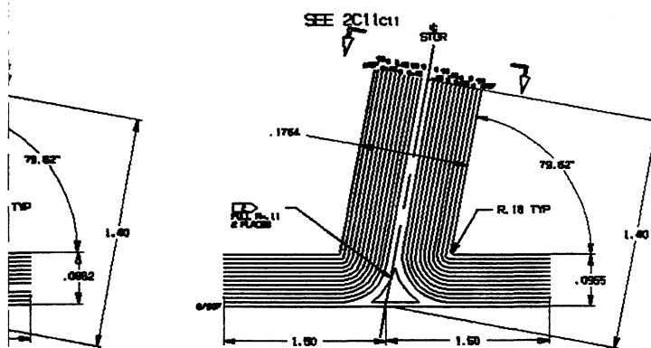
TYPICAL SECT (STA 1571 TO STA 1622) (FOR DETAIL -201) SCALE: NONE
