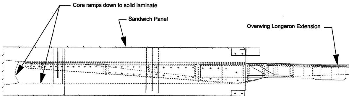
Figure 4-27. Overwing Longerons Installation
