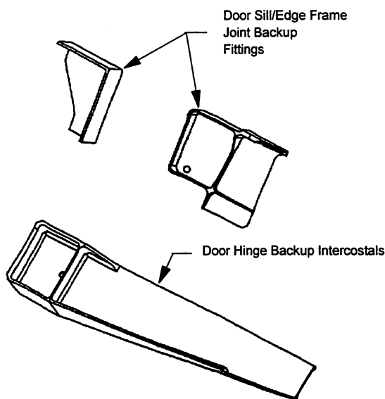
Figure 4-10. Typical Family B Metallic Fittings
