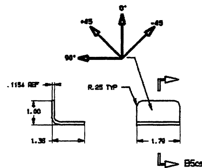
DETAIL -20 SCALE:1/1
