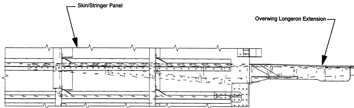
Figure 4-15. Overwing Longeron Extension Installation
