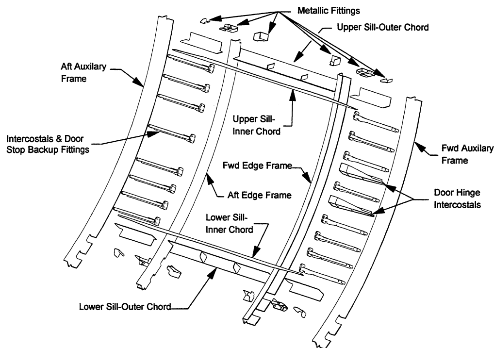
Figure 4-9. Door Surround Structure Assembly
