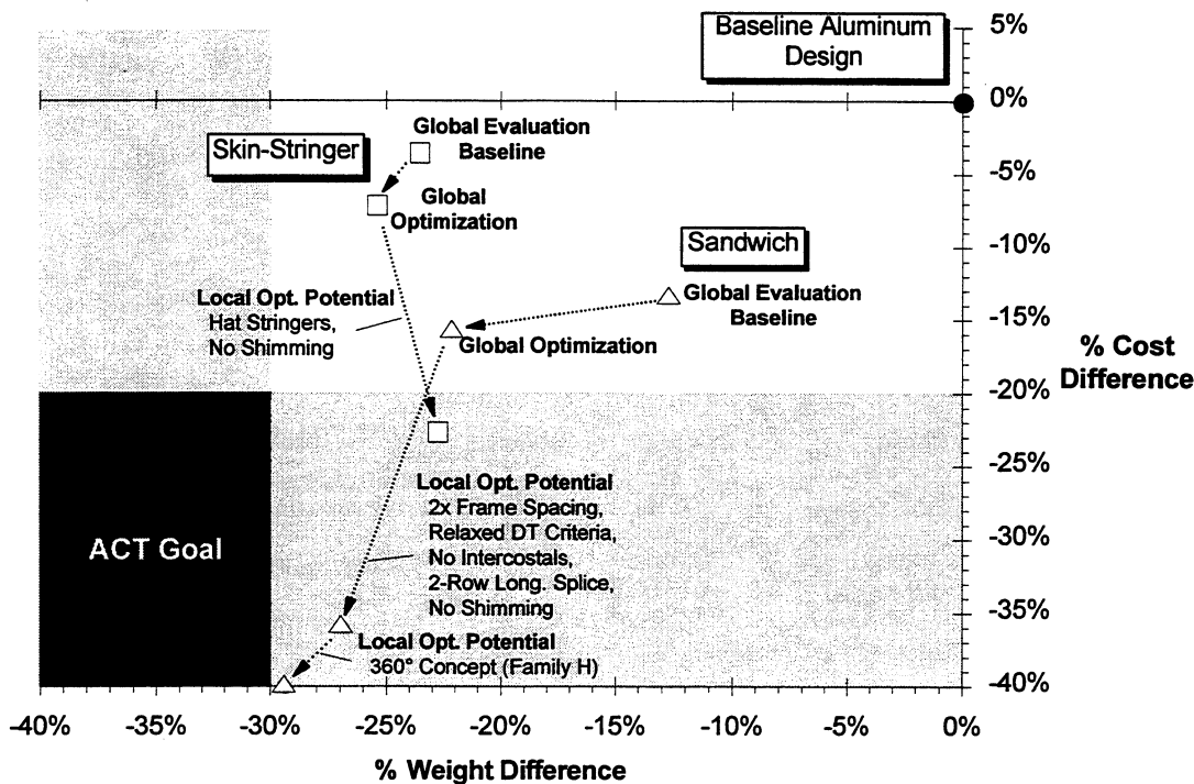
Figure 5-3. Results of Side Panel Global Optimization Trades
