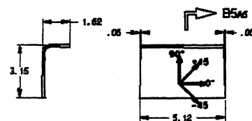
DETAIL-3 SCALE:1/2
