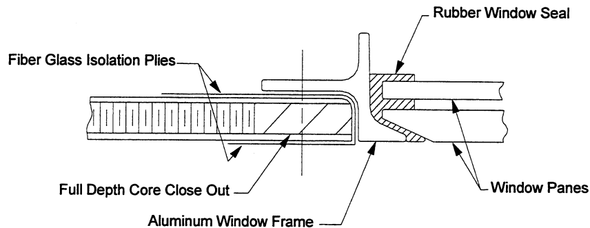
Figure 4-23. Window Reinforcement Structure
