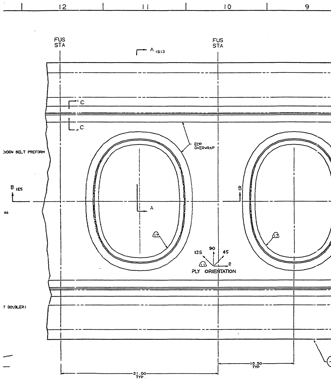
VIEW LOOKING OUTBD, LHS
