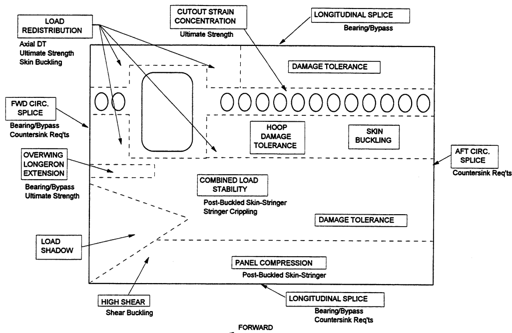
Figure 4-2. Skin/Stringer Critical Design Drivers
