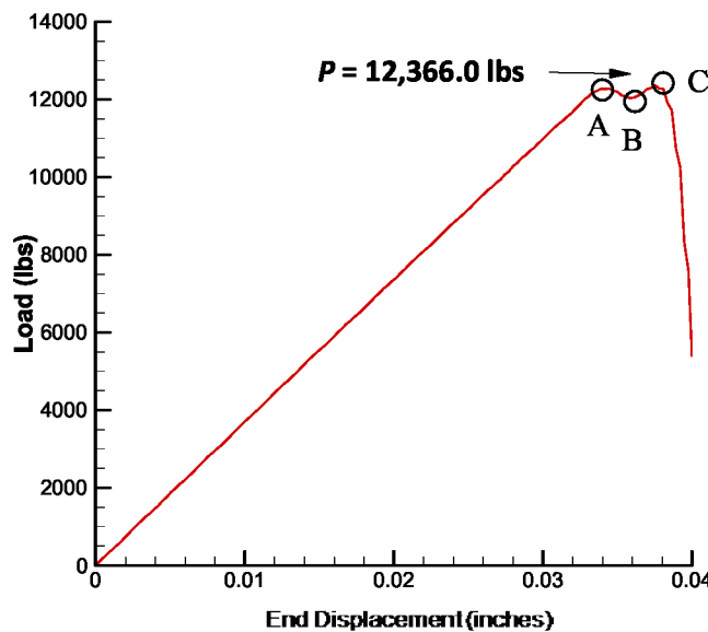
Figure 3.19. Load versus end displacement of a [45_4/90_4/-45_4/0_4]_8 laminate with a 0.25-inch-diameter hole (curve smoothened).
