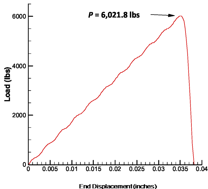
Figure 3.25. Load versus end displacement of a [45_2/90_2/-45_2/0_2]_s laminate with a 0.25-inch-diameter hole (curve smoothened).
