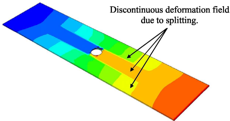
Figure 3.12. Axial deformation in the 0° plies due to splitting.
