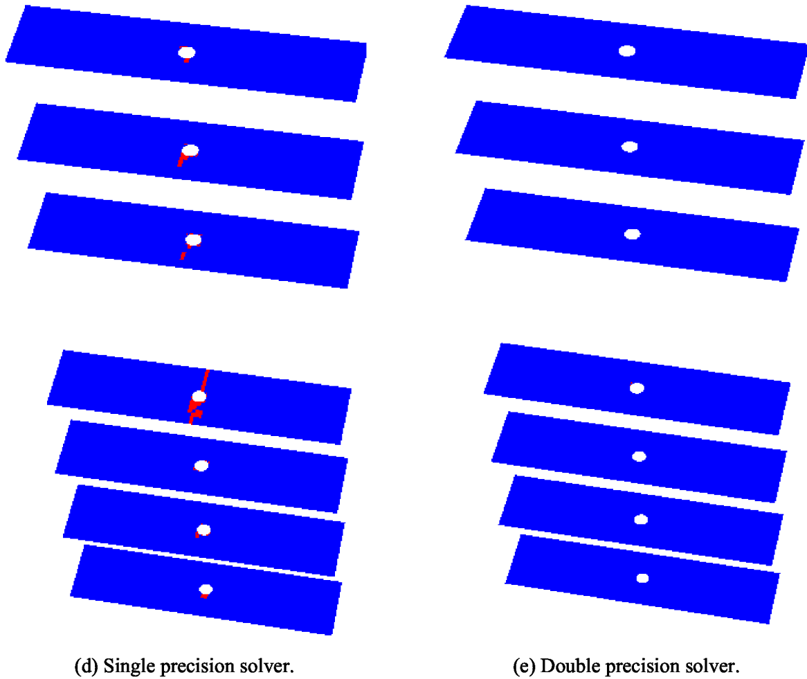
Figure 3.40 (continued). End displacement of 0.0344 inches; fiber damage obtained using (d) single precision and (e) double precision solver for all layers.
