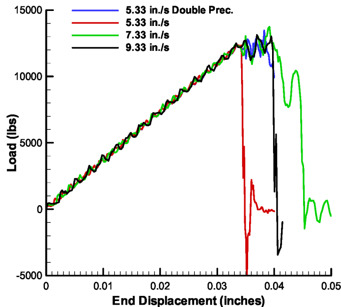
Figure 3.29. Load versus end displacement of a [45_4/90_4/-45_4/0_4]_s laminate with a 0.25-inch-diameter hole (curves smoothened).
