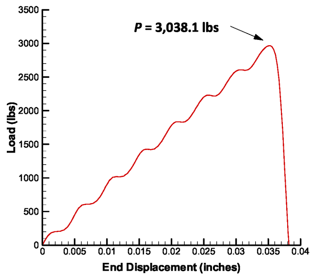
Figure 3.27. Load versus end displacement of a [45/90/-45/0]_s laminate with 0.25-inch-diameter hole (curves smoothed).
