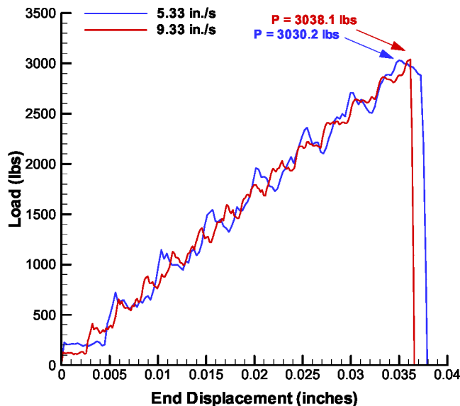
Figure 3.43. Load versus end displacement of a [45/90/-45/0]_s laminate with a 0.25-inch-diameter hole.
