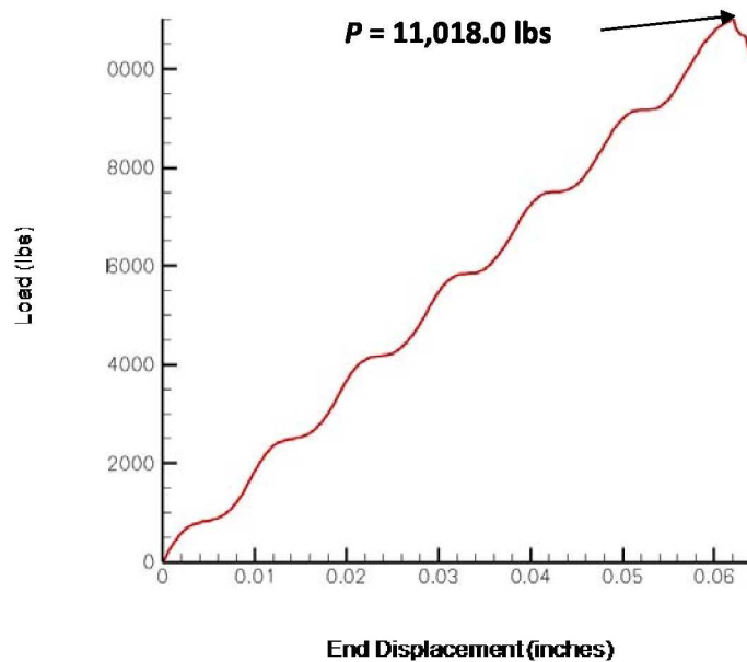
Figure 3.14. Load versus end displacement of a [45_2/90_2/-45_2/0_2]_s laminate with a 0.5-inch-diameter hole (curve smoothened).
