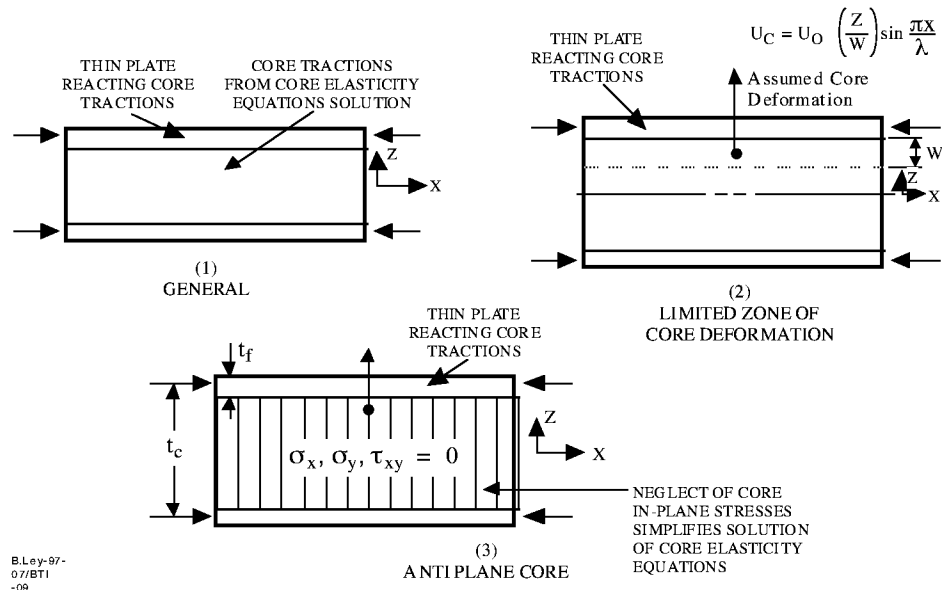
Figure 7. Summary of Facesheet Wrinkling Mathematical Models
