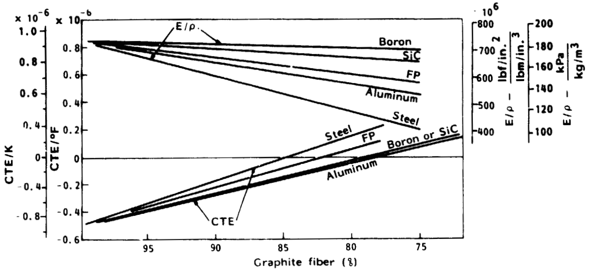
Figure 5. - Effect of replacing GY70 fiber with other selected fibers in a unidirectional laminate.
