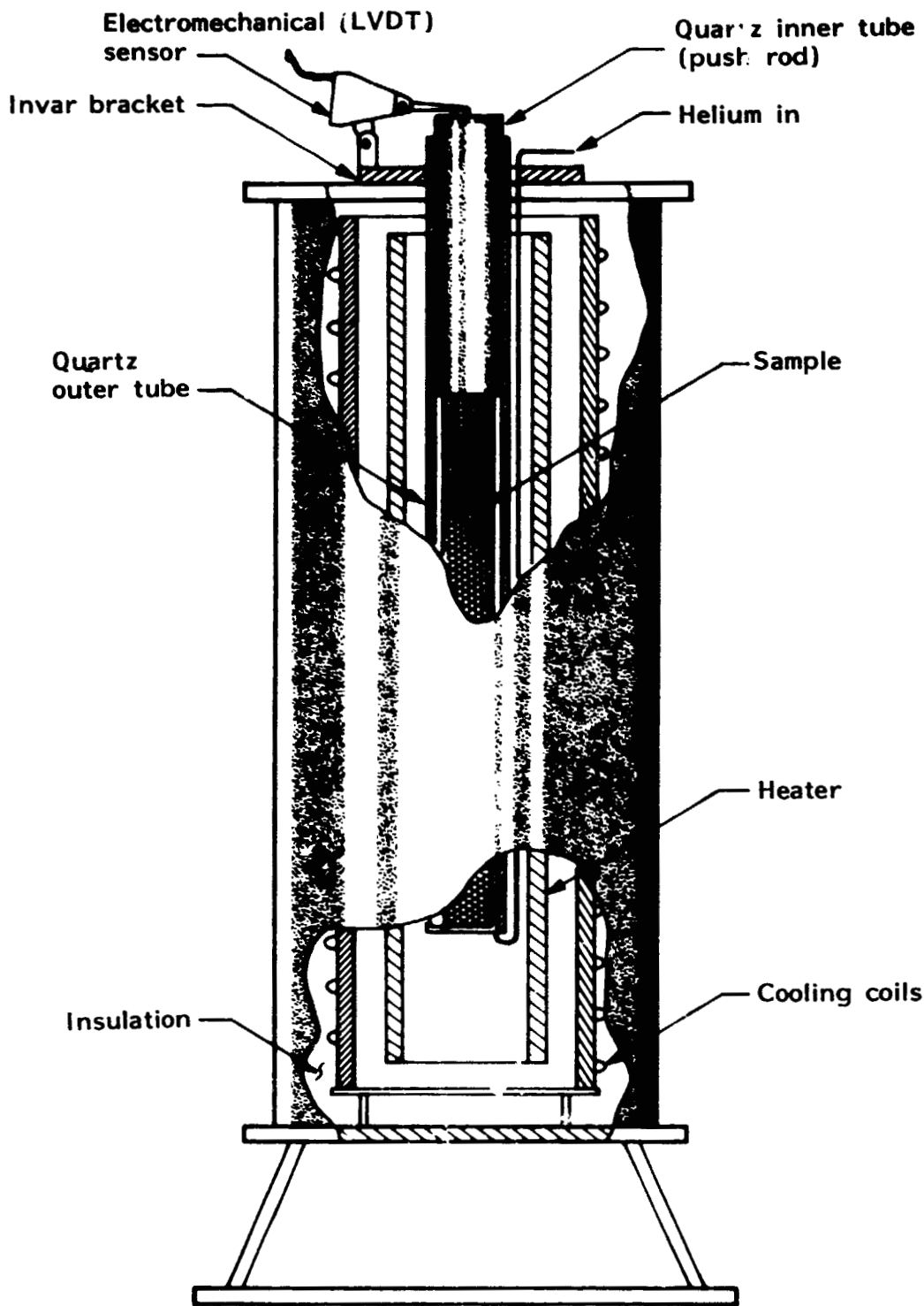
Figure 9. - Electromechanical dilatometer.
