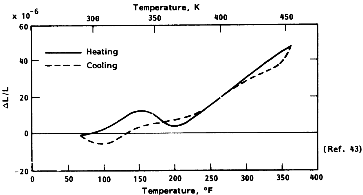
Figure 14. - Thermal expansion of Thornel 300/Narmco 5208 tape (0° fiber direction).
