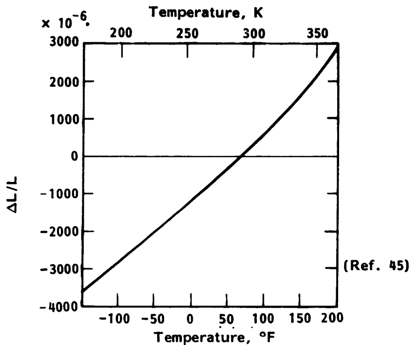
Figure 27. - Thermal expansion of HMS/CE339 unidirectional tape (90° fiber direction).
