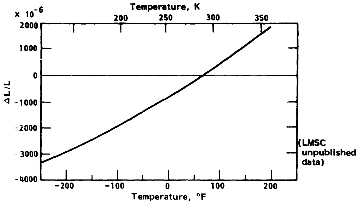
Figure 21. - Thermal expansion of unidirectional HTS-2/3501-5A tape (90° fiber direction).
