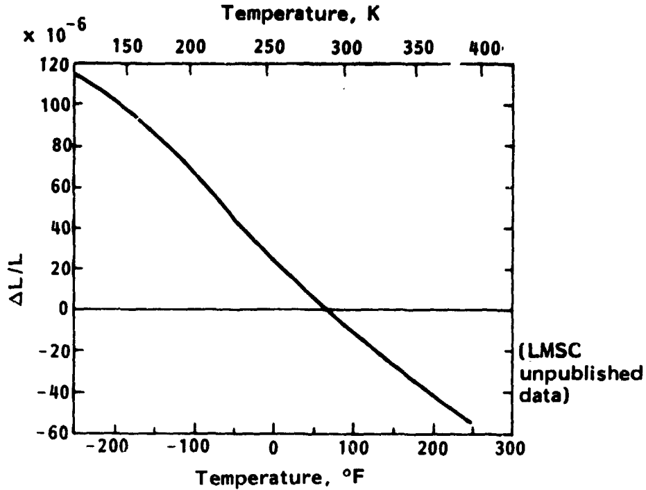
Figure 33. - Thermal expansion of unidirectional Thornel-50 (Pan)/F263 tape (0° fiber direction).
