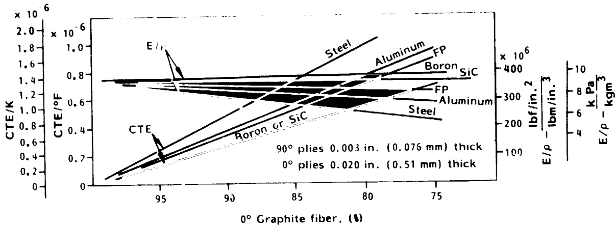
Figure 8. - Effect of replacing 0° VSB-32 fiber with other selected fibers in a (90/0/90) layup.
