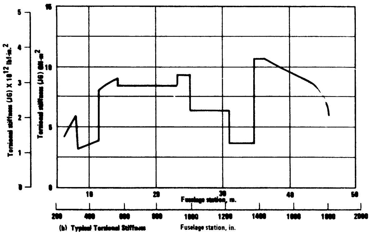
Figure 3. - Typical fuselage stiffnesses for a wide-bodied aluminum aircraft.
