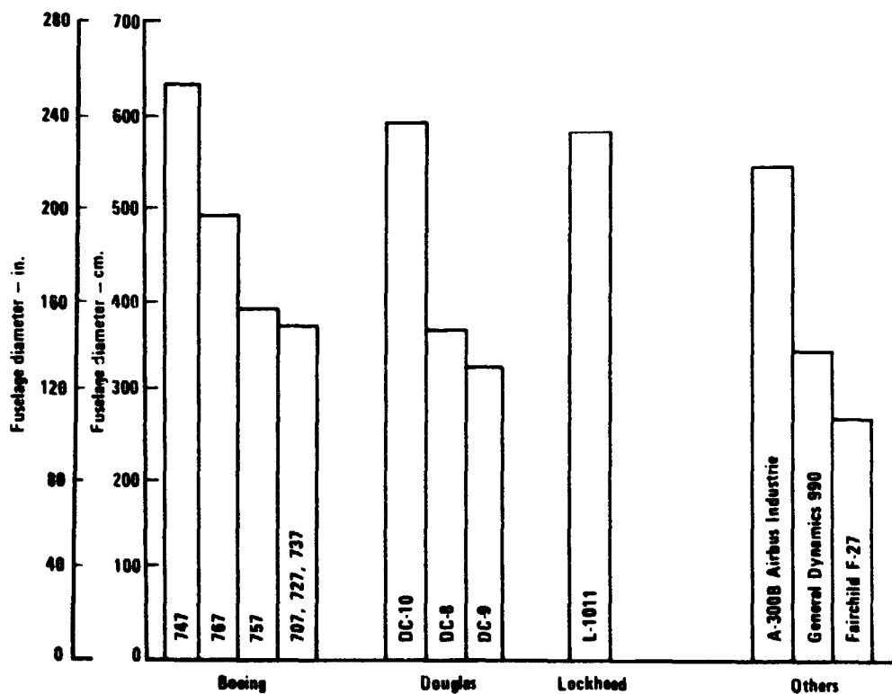
Figure 2. - Fuselage diameters for commercial transport aircraft.
