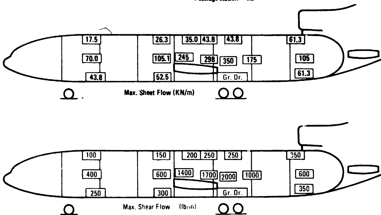
Figure 14. - Maximum limit load intensities in fuselage shell.
