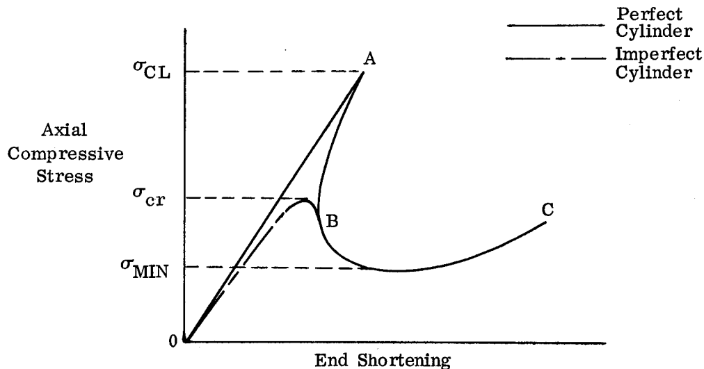
Figure 4.1-1. Equilibrium Paths for Axially Compressed Circular Cylinders
