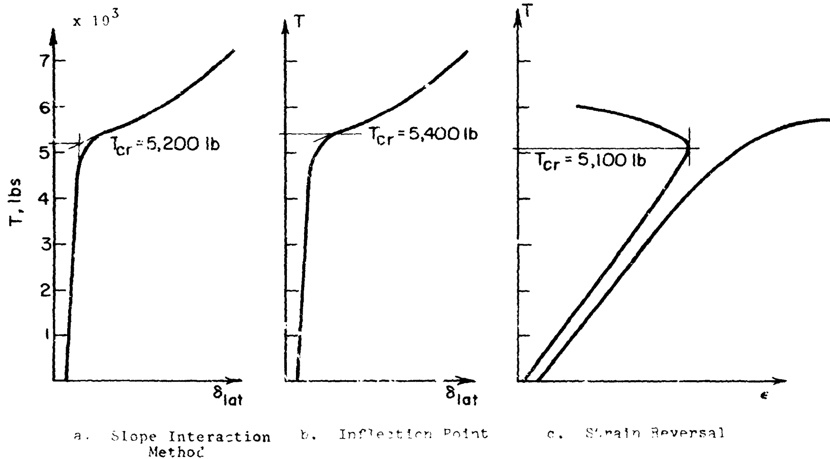
FIGURE 15 - Criteria for Defining Critical Buckling Load Applied to Test Data for Unperforated Plate.
