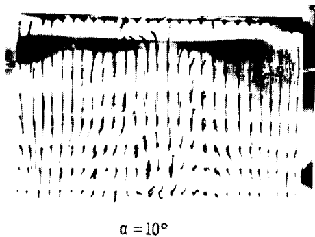
Figure 21.- Oil flow pattern of single-element airfoil illustrating tunnel sidewall effects in 6 x 28-inch TT.
