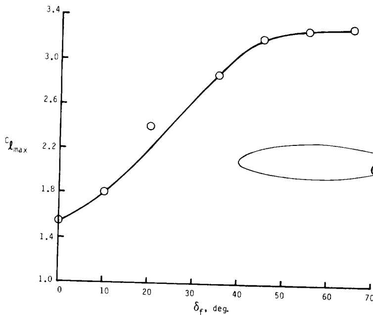
Figure 6.- Maximum lift coefficients for NACA 65 3 -118 airfoil equipped with double-slotted flap. ( R = 6 \times 10^6 )
