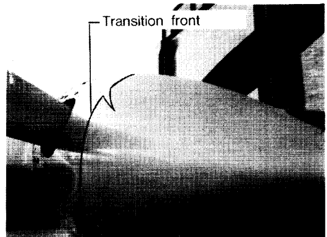
Figure 5.- Natural laminar flow on the propeller spinner of the Cessna P210 airplane (ref. 1).
