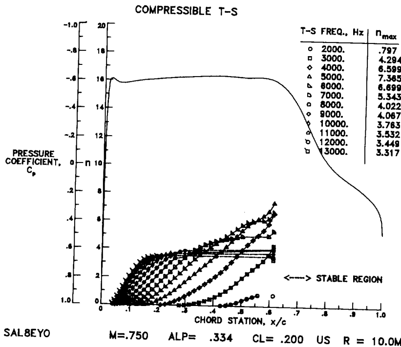
Figure 19.- Calculated inviscid pressure distribution and the compressible logarithmic amplification of various TS disturbance frequencies for the upper surface of the SAL8EY0 airfoil at design.
