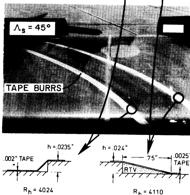
Figure 13. Transition visualization on swept shaped steps on T-34C NLF glove flight experiments.
