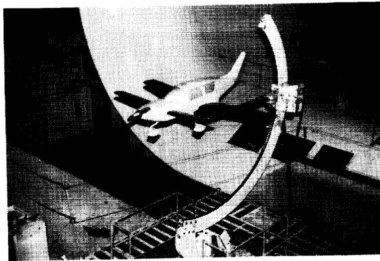
Figure 17.- Canard, tractor configuration mounted in the 30- by 60-Foot Wind Tunnel.
