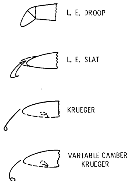
Figure 7.- Mechanical high-lift leading-edge devices.
