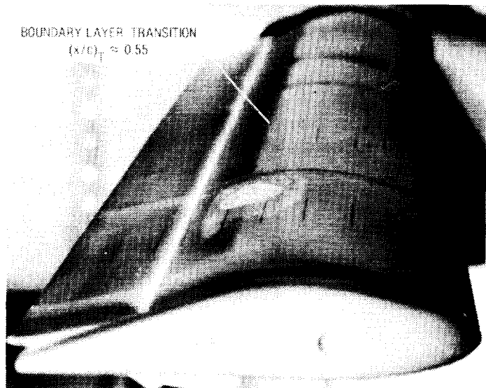
(b) Canard.
