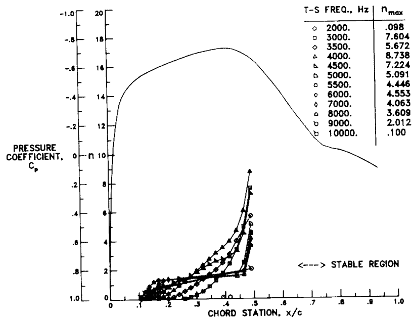
Figure 16.- Calculated three-dimensional pressure distribution and the compressible logarithmic amplification of various TS disturbance frequencies for the upper surface of the F-14 NASA glove.
