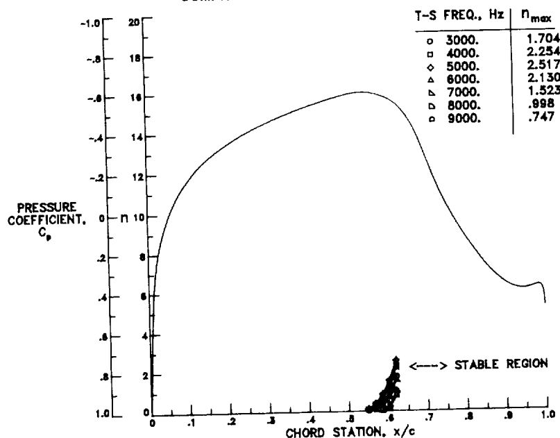
Figure 21.- Calculated inviscid pressure distribution and the compressible logarithmic amplification of various TS disturbance frequencies for the lower surface of the SAL8EY0 airfoil at design.
