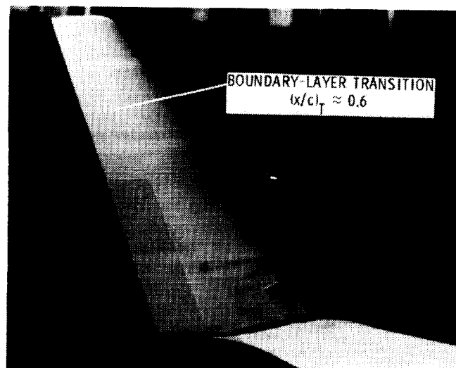
(c) Winglet.
