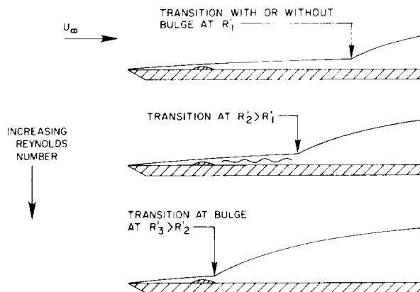
Figure 2. Effects of two-dimensional surface imperfection on laminar flow.
