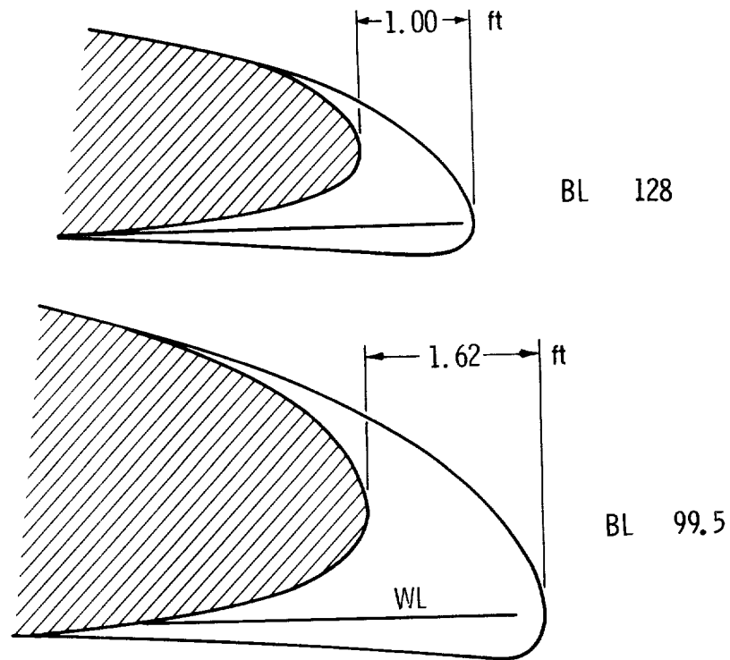
(b) Leading-edge droop.
