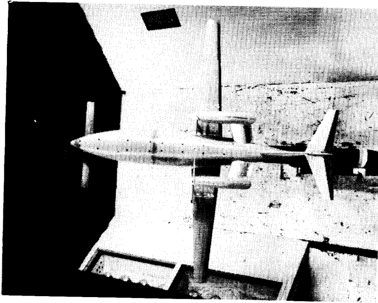
Figure 41.- Photograph of three-surface over-the-wing propeller configuration.
