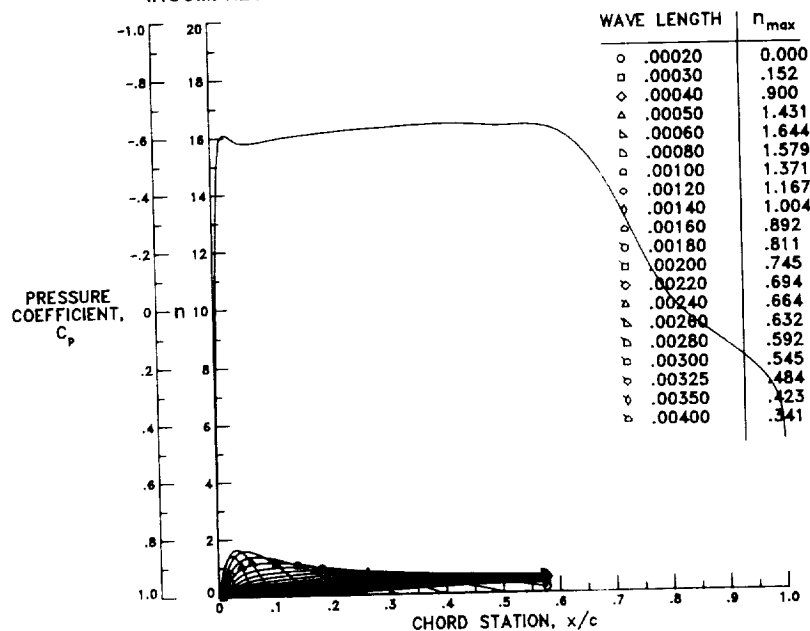
Figure 20.- Calculated inviscid pressure distribution and the incompressible logarithmic amplification of various crossflow disturbance wavelengths for the upper surface of the SAL8EY0 airfoil at design.
