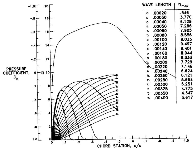
Figure 17.- Calculated three-dimensional pressure distribution and the incompressible logarithmic amplification of various crossflow disturbance wavelengths for the upper surface of the F-14 NASA glove.
