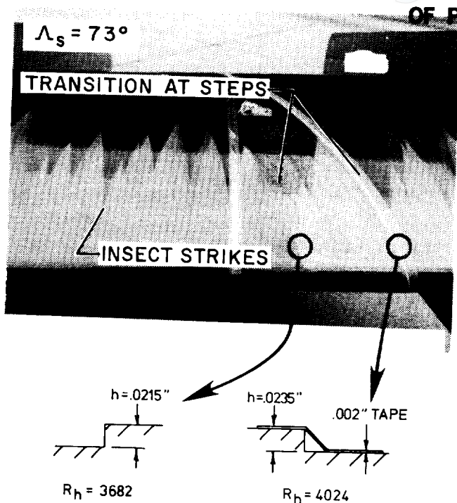
Figure 12. Transition visualization on swept shaped steps on T-34C NLF glove flight experiments.
