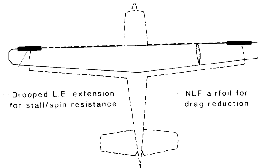
Figure 29.- Leading-edge droop modification applied to advanced wing design.
