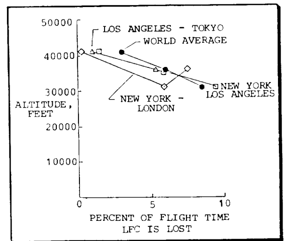
Figure 16.- Cloud particle impact on laminar flow loss from GASP data base analysis.
