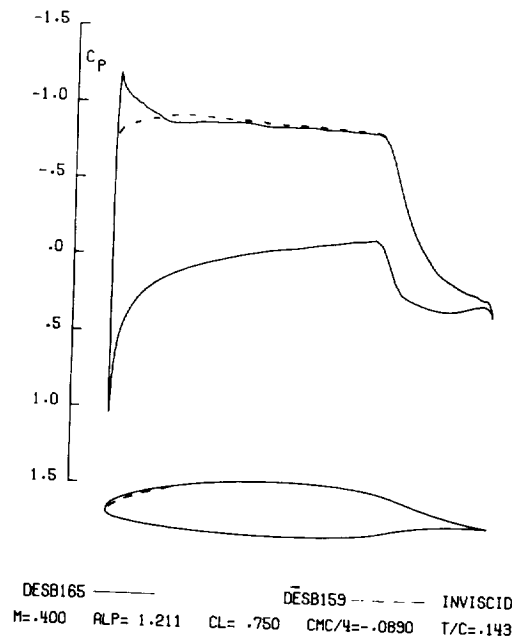
Figure 8.- Comparison of inviscid pressure distributions of DES165 airfoil with the DES159 airfoil at the climb condition.
