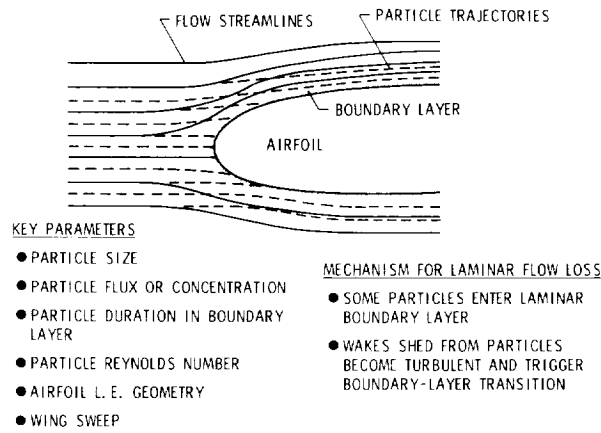
Figure 17.- Ice particle penetration and breakdown of the laminar boundary layer.
