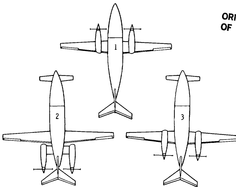
Figure 38.- Plan views of three-surface and conventional configurations.
