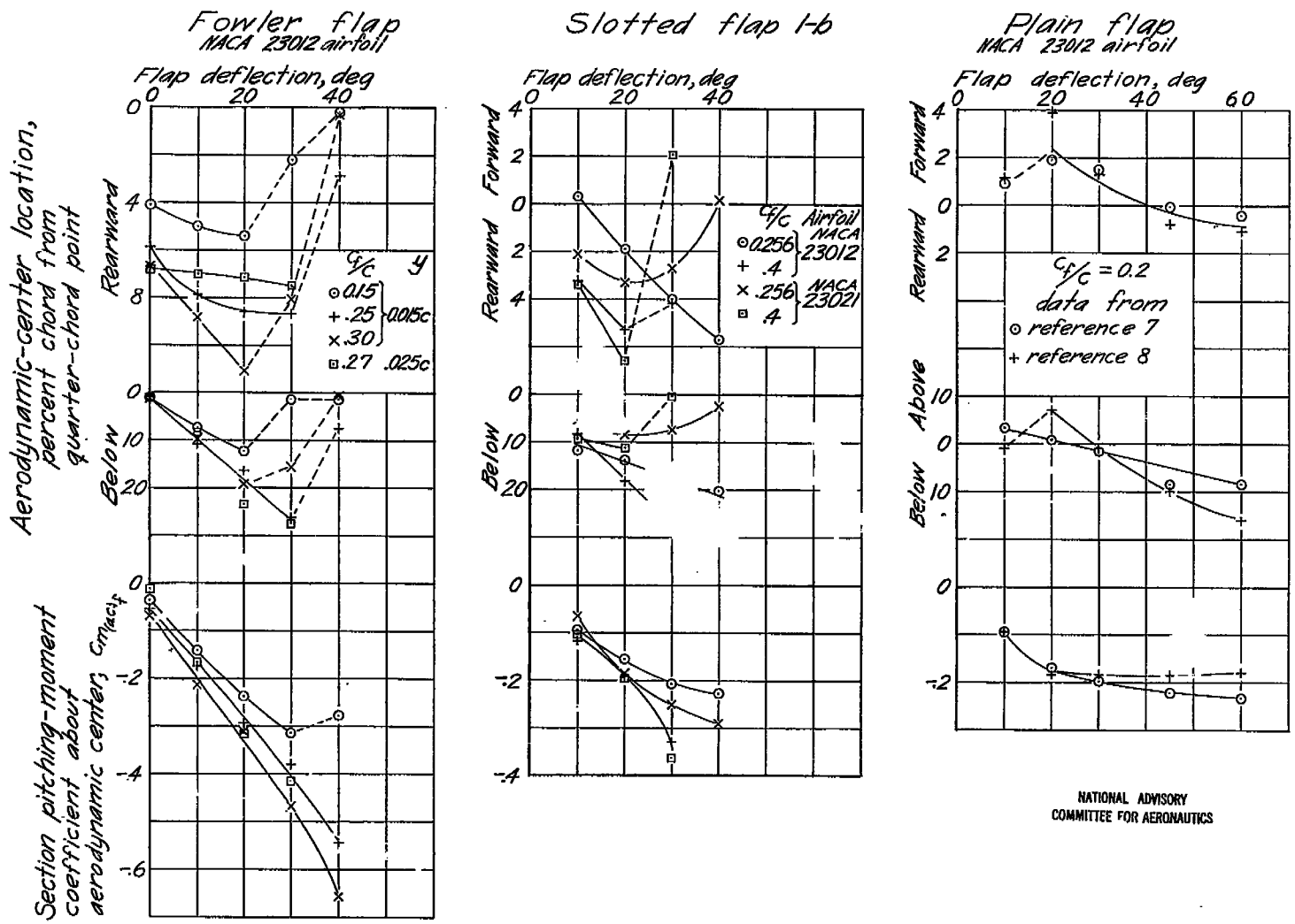
(a) Effect of various flap types on NACA 23012 airfoil.
