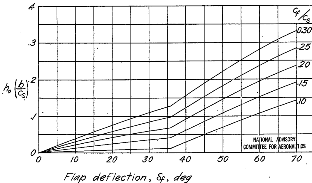
Figure 12.- Downward displacement of wake origin as a function of flap deflection. (Data from reference 5.)
