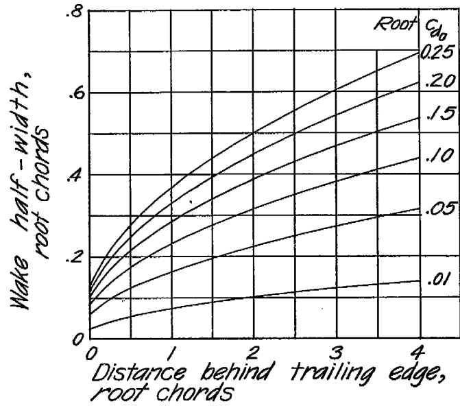
(a) Variation of wake width with distance from trailing edge.
