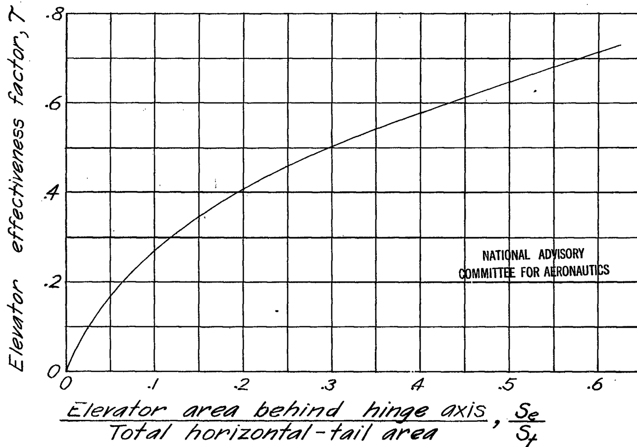
Figure 2.- Variation of elevator effectiveness factor \tau with ratio of elevator area behind hinge axis to total horizontal-tail area. (From reference 2.) \tau = \frac{dC_{N_t}/d\delta_e}{dC_{N_t}/da_t} .
