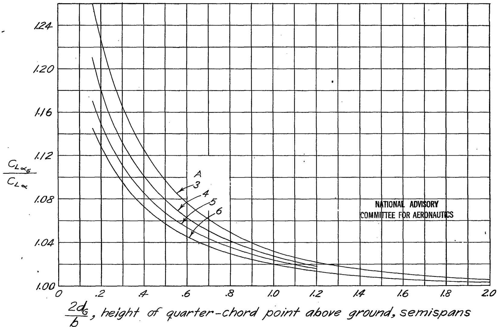
Figure 6.- Ground effect on lift-curve slope.
