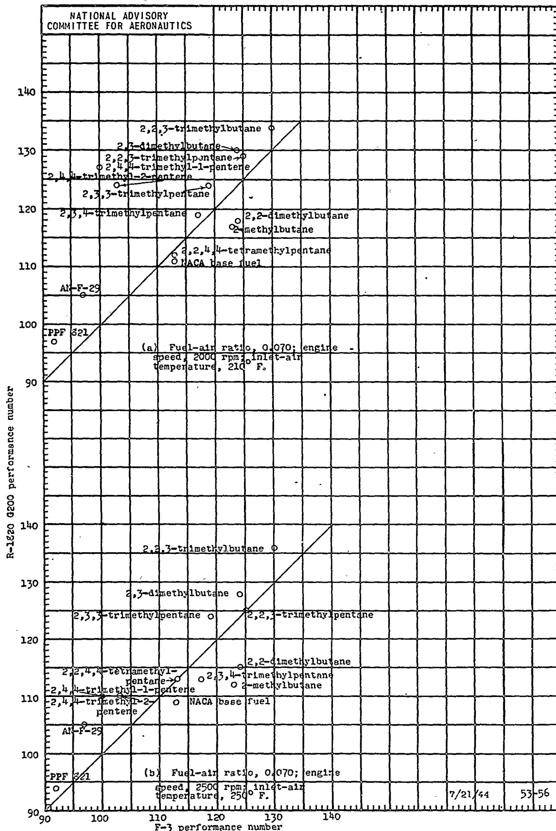
Figure 15. - Comparison of fuel blend ratings with F-3 ratings. Wright R-1820 G200 cylinder; compression ratio, 7.3; spark advance, 20° B.T.C.; cooling air adjusted at 140 bmep and 0.10 fuel-air ratio to give a rear spark-plug-bushing temperature of 365° F.
