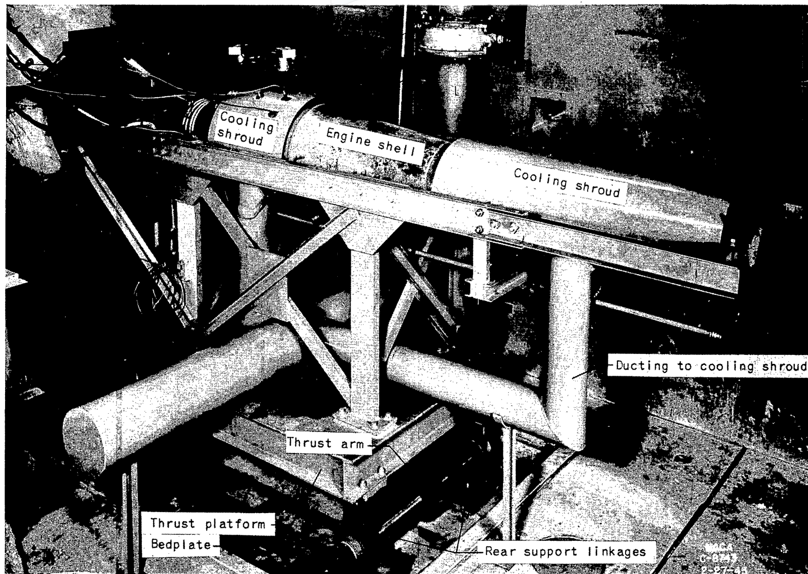
Figure 5. - Test installation of 22-inch-diameter pulse-jet engine.
