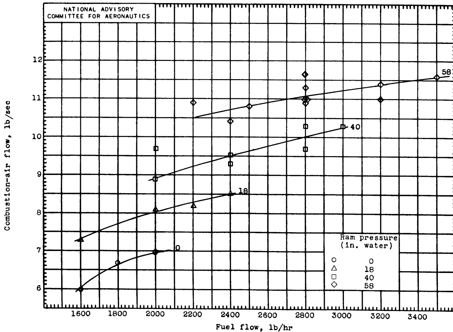
Figure 8.- Variation of combustion-air weight flow with fuel flow for the test simulated ram pressures.
