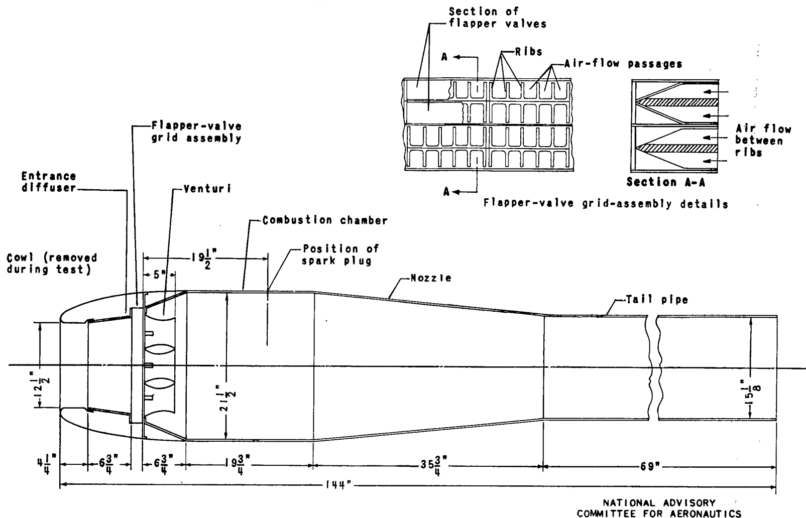
Figure 1. - Details of 22-inch-diameter pulse-jet engine.
