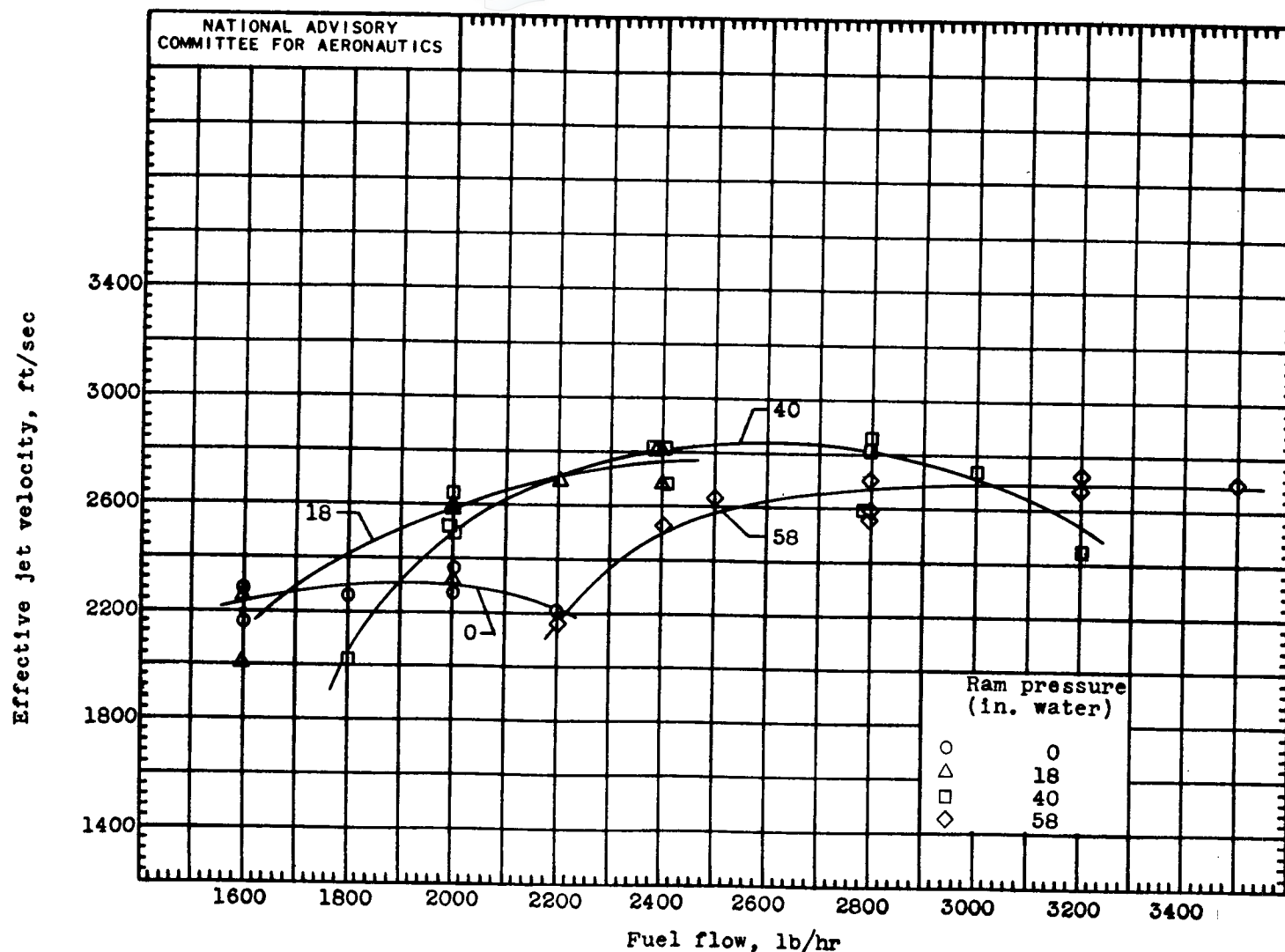
Figure 9.- Variation of effective jet velocity with fuel flow for the test simulated ram pressures.
