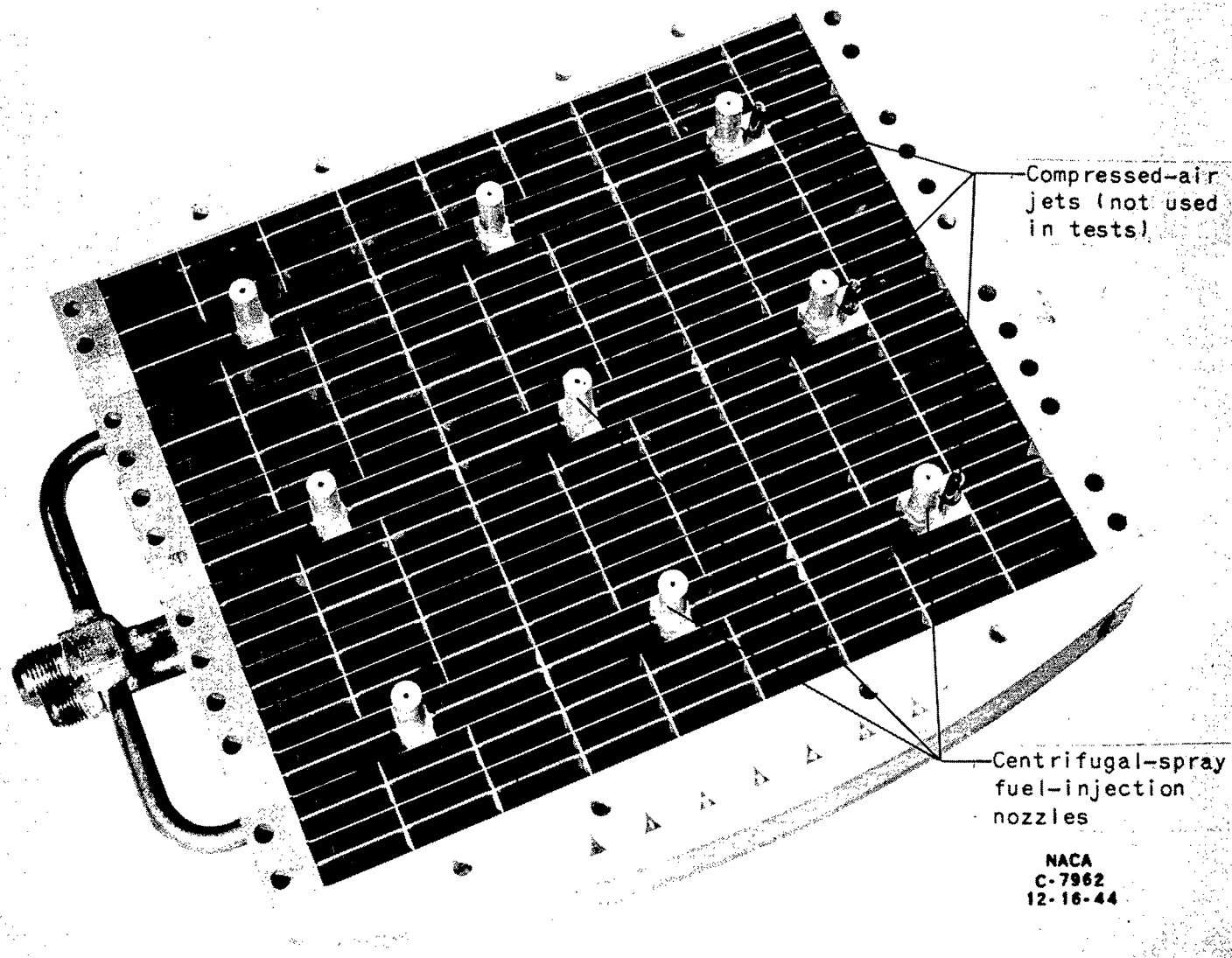
Figure 2. - Rear view (downstream face) of flapper-valve grid assembly.
