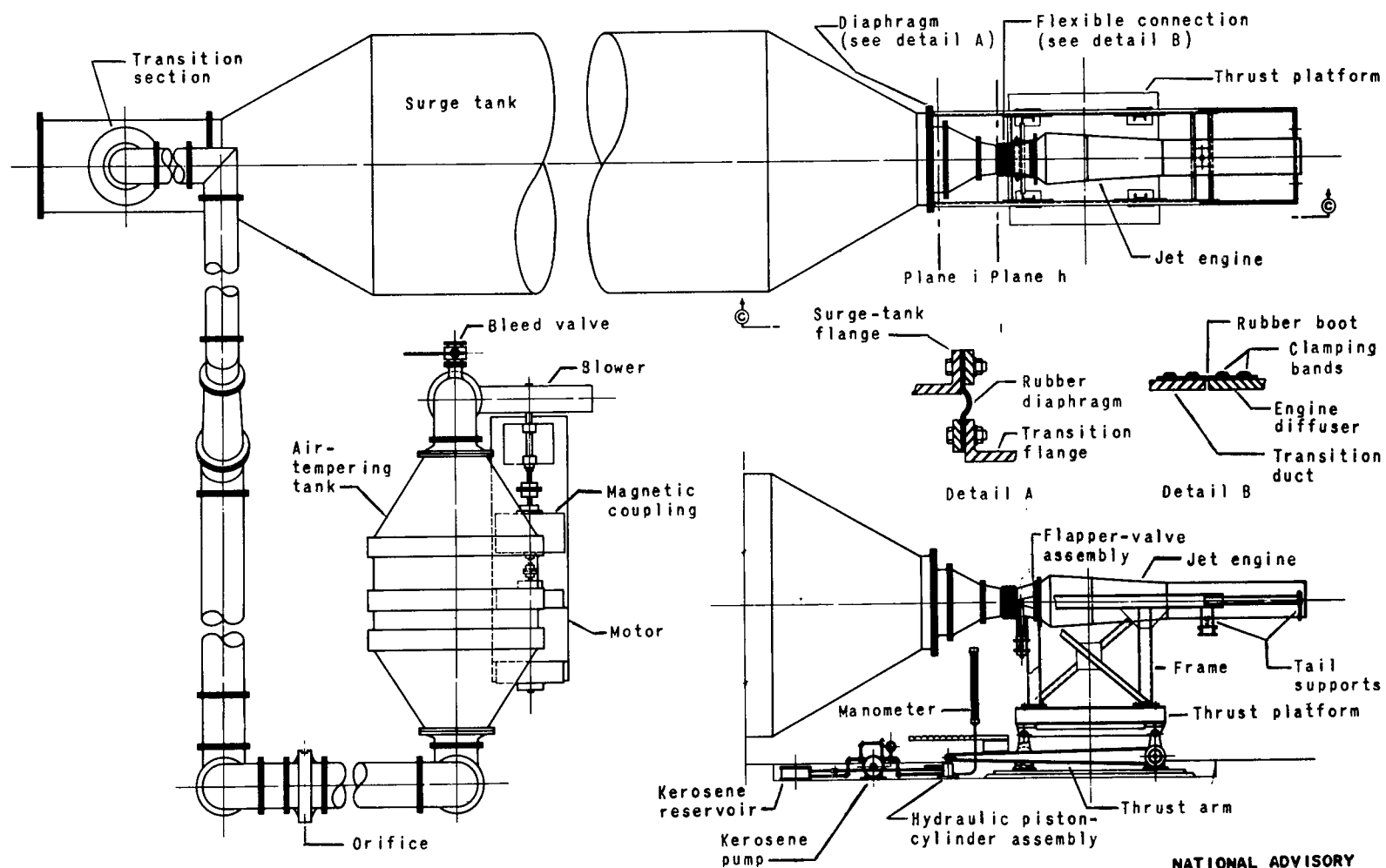
Figure 4. - Schematic diagram of test installation of 22-inch-diameter pulse-jet engine.
