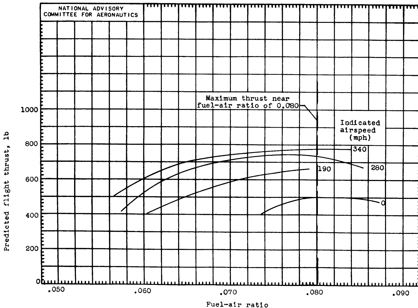
Figure 12. - Variation of predicted flight thrust (excluding external drag) with fuel-air ratio for the various simulated flight speeds. (Sea-level operation in approximately NACA air.)
