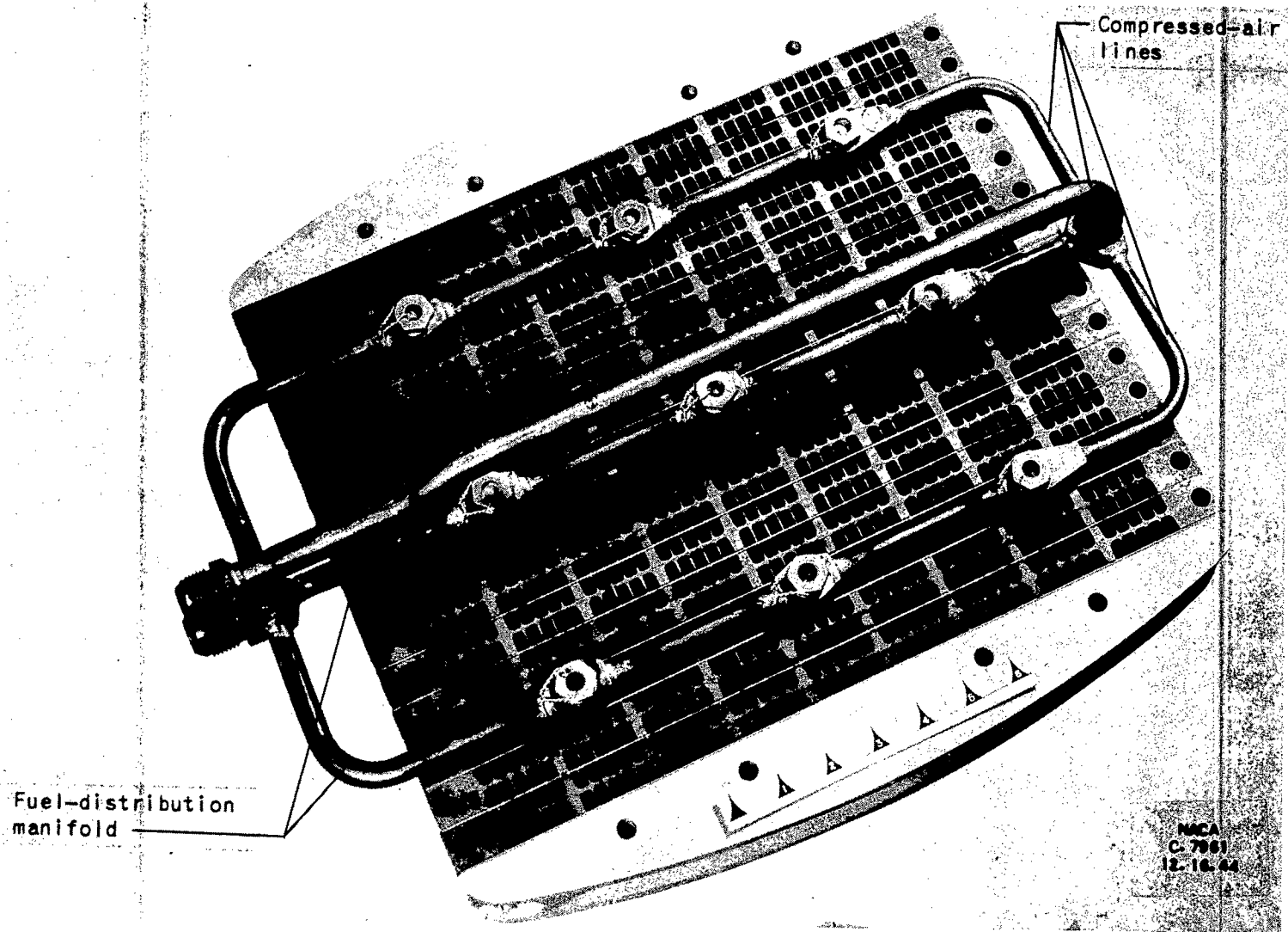
Figure 3. - Front view (upstream face) of flapper-valve grid assembly.
