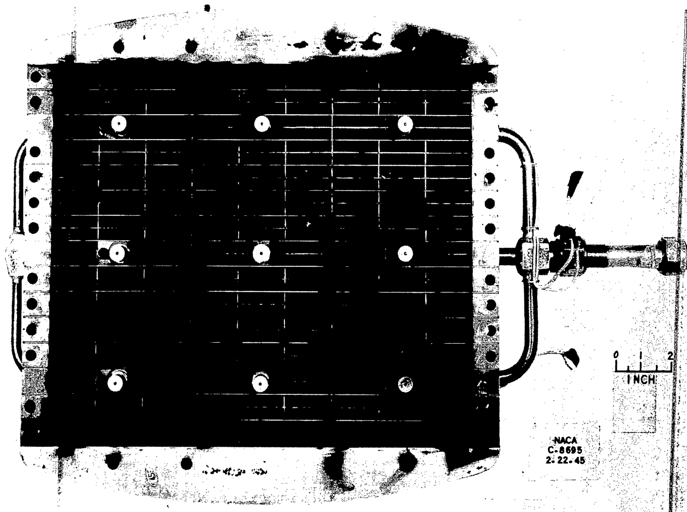
Figure 19. - Flapper-valve grid assembly after 30 minutes of operation.
