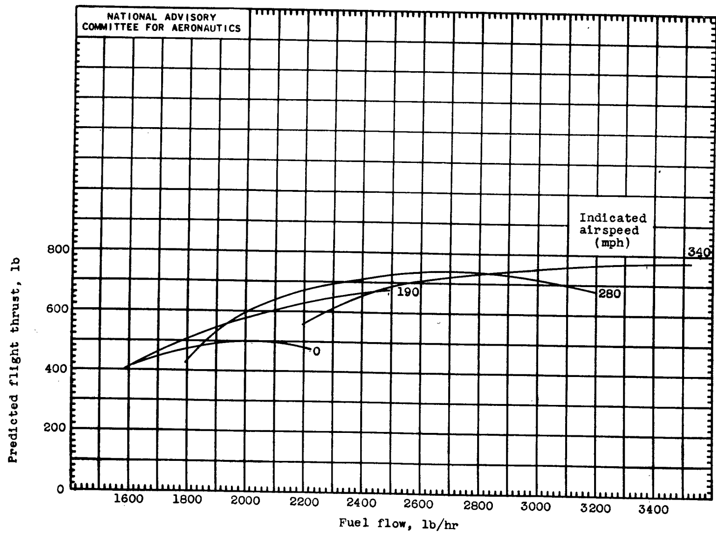
Figure 11. - Variation of predicted flight thrust (excluding external drag) with fuel flow for the various simulated flight speeds. (Sea-level operation in approximately NACA air.)
