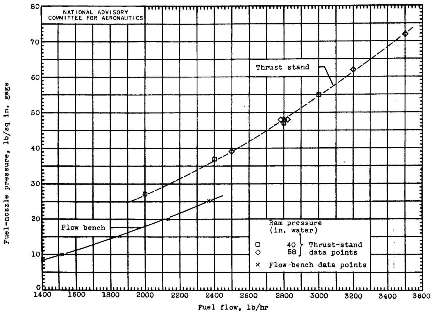
Figure 17.- Variation of fuel-nozzle pressure with fuel flow showing difference of thrust-stand data (obtained during operation) from the flow-bench calibration.
