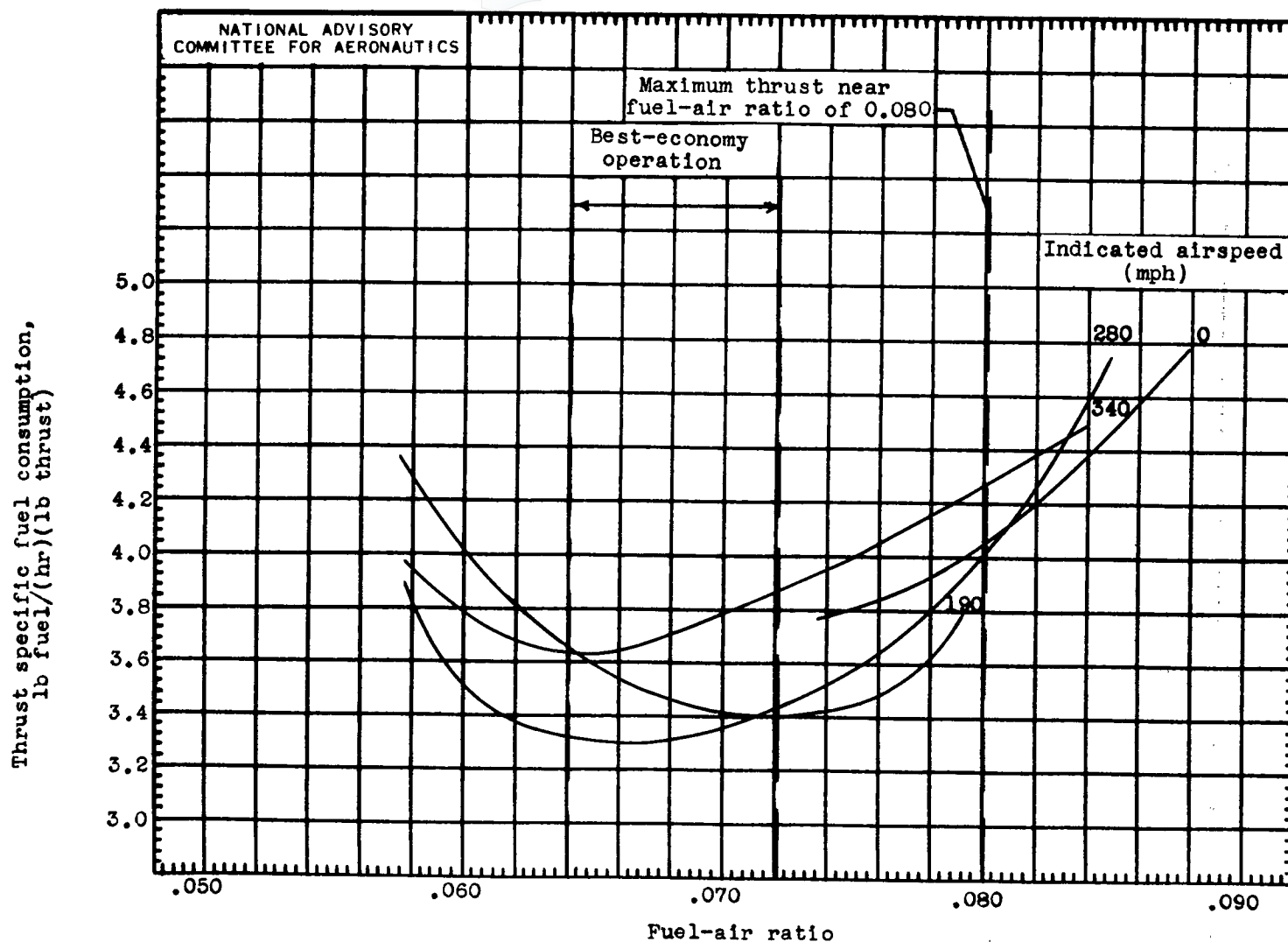
Figure 13.- Variation of thrust specific fuel consumption with fuel-air ratio for the various simulated flight speeds. (Sea-level operation in approximately NACA air.)
