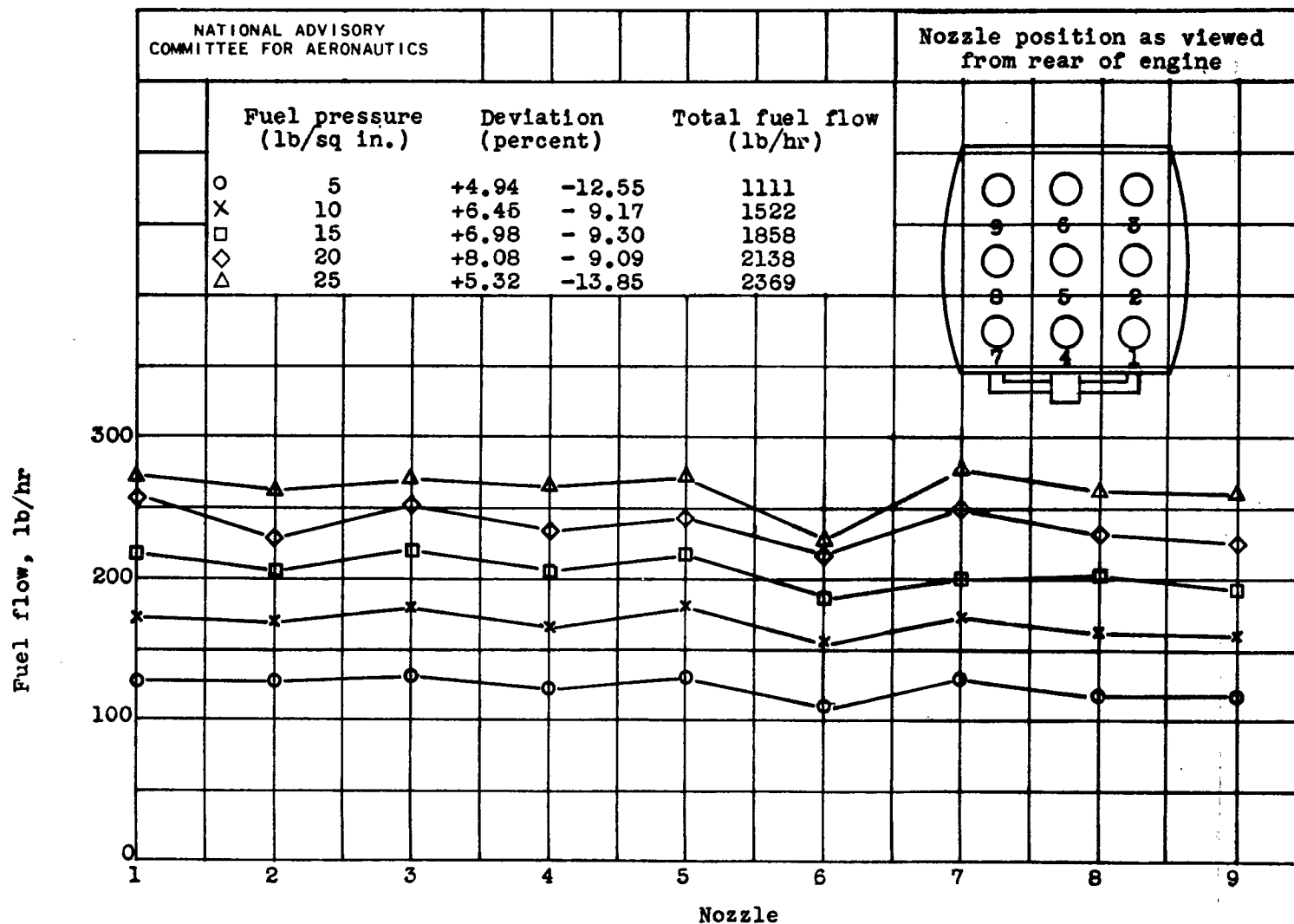
Figure 7.- Results of flow-bench tests on fuel-injection nozzles showing individual-nozzle fuel flows.
