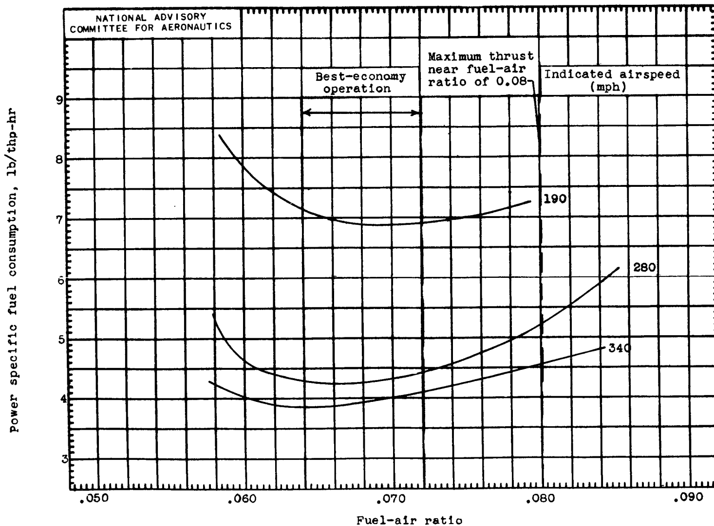
Figure 14. - Variation of power specific fuel consumption with fuel-air ratio for the various simulated flight speeds. (Sea-level operation in approximately NACA air.)
